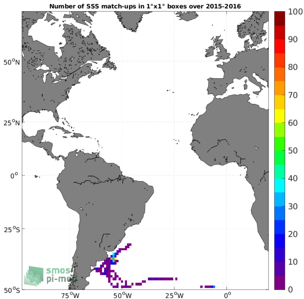
Figure 4: Number of SSS match-ups between Marine mammals SSS and the SMAP SSS L3 v5 - Monthly (RSS) SSS product for the Atlantic Ocean Pi-MEP region over 1°x1° boxes and for the full satellite product period.
