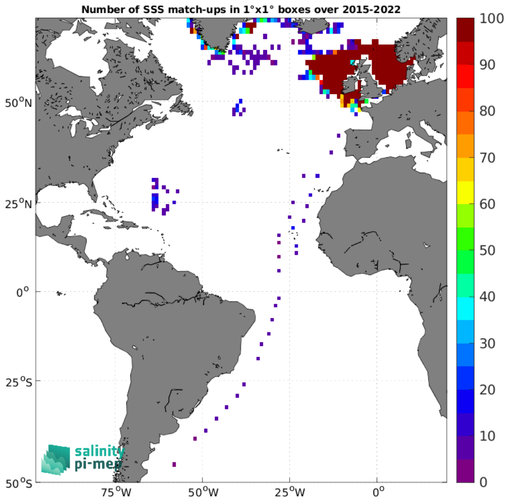
Figure 4: Number of SSS match-ups between ICES SSS and the SMAP SSS L3 v5 - Monthly (RSS) SSS product for the Atlantic Ocean Pi-MEP region over 1^\circ \times 1^\circ boxes and for the full satellite product period.
