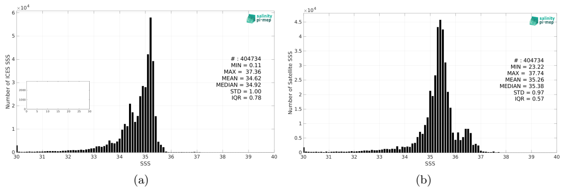
Figure 2: Histograms of SSS from ICES (a) and SMAP SSS L3 v5 - Monthly (RSS) (b) considering all match-up pairs per bins of 0.1 over the Atlantic Ocean Pi-MEP region and for the full satellite product period.
