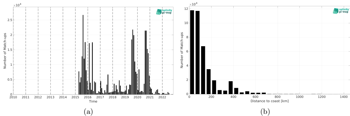
Figure 1: Number of match-ups between ICES and SMAP SSS L3 v5 - Monthly (RSS) SSS as a function of time (a) and as function of the distance to coast (b) over the Atlantic Ocean Pi-MEP region and for the full satellite product period.
