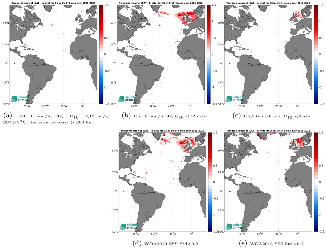
Figure 12: Temporal mean gridded over spatial boxes of size 1^\circ \times 1^\circ of \Delta SSS (SMAP SSS L3 v5 - Monthly (RSS) - ICES) for 5 different subdatasets corresponding to:RR=0 mm/h, 3 < U_{10} < 12 m/s, SST >5^\circ\text{C} , distance to coast > 800 km (a), RR=0 mm/h, 3 < U_{10} < 12 m/s (b), RR >1 mm/h and U_{10} < 4 m/s (c), WOA2013 SSS Std <0.2 (d), WOA2013 SSS Std >0.2 (e).
