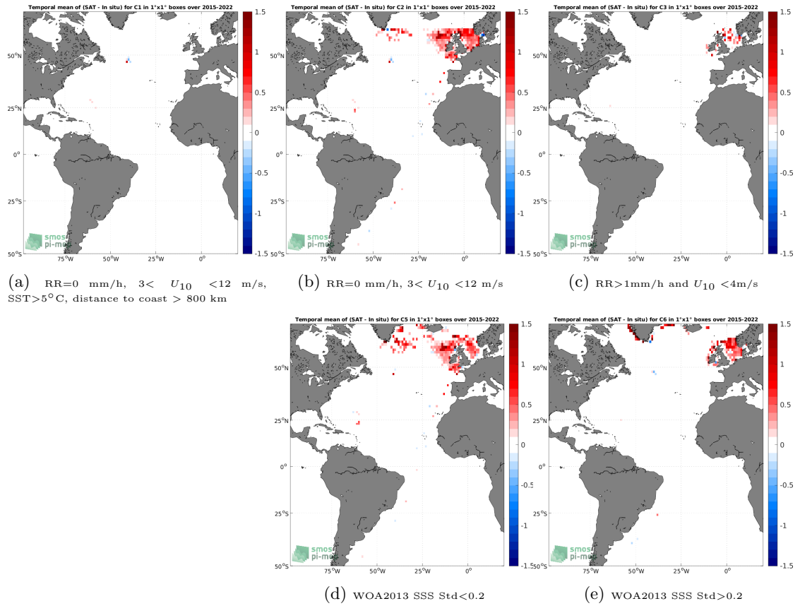
Figure 12: Temporal mean gridded over spatial boxes of size 1^\circ \times 1^\circ of \Delta SSS (SMAP SSS L3 v5 - Monthly (RSS) - ICES) for 5 different subdatasets corresponding to:RR=0 mm/h, 3 < U_{10} < 12 m/s, SST >5^\circ\text{C} , distance to coast > 800 km (a), RR=0 mm/h, 3 < U_{10} < 12 m/s (b), RR >1 mm/h and U_{10} < 4 m/s (c), WOA2013 SSS Std <0.2 (d), WOA2013 SSS Std >0.2 (e).
