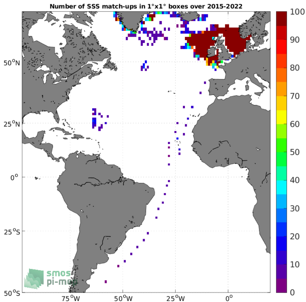
Figure 4: Number of SSS match-ups between ICES SSS and the SMAP SSS L3 v5 - Monthly (RSS) SSS product for the Atlantic Ocean Pi-MEP region over 1°x1° boxes and for the full satellite product period.
