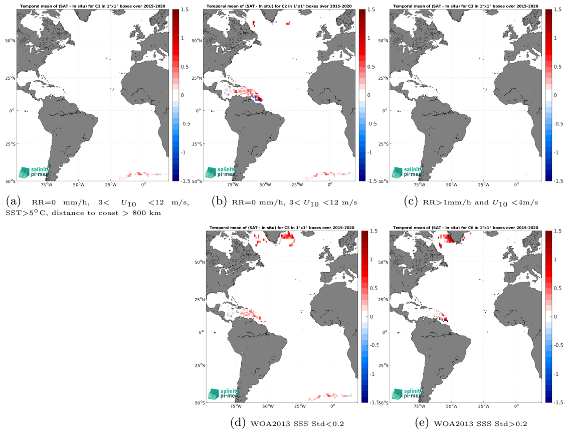
Figure 11: Temporal mean gridded over spatial boxes of size 1^\circ \times 1^\circ of \Delta SSS (SMAP SSS L3 v5 - Monthly (RSS) - Surface drifters) for 5 different subdatasets corresponding to:RR=0 mm/h, 3 < U_{10} < 12 m/s, SST >5^\circ\text{C} , distance to coast > 800 km (a), RR=0 mm/h, 3 < U_{10} < 12 m/s (b), RR >1 mm/h and U_{10} < 4 m/s (c), WOA2013 SSS Std <0.2 (d), WOA2013 SSS Std >0.2 (e).
