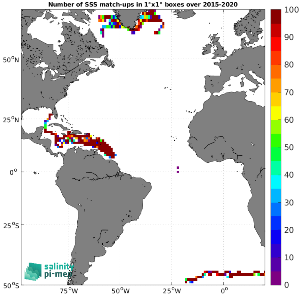
Figure 3: Number of SSS match-ups between Surface drifters SSS and the SMAP SSS L3 v5 - Monthly (RSS) SSS product for the Atlantic Ocean Pi-MEP region over 1^\circ \times 1^\circ boxes and for the full satellite product period.
