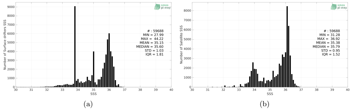
Figure 2: Histograms of SSS from Surface drifters (a) and SMAP SSS L3 v5 - Monthly (RSS) (b) considering all match-up pairs per bins of 0.1 over the Atlantic Ocean Pi-MEP region and for the full satellite product period.
