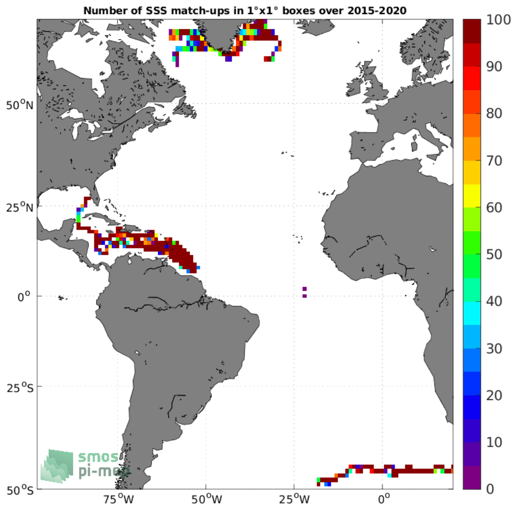
Figure 3: Number of SSS match-ups between Surface drifters SSS and the SMAP SSS L3 v5 - Monthly (RSS) SSS product for the Atlantic Ocean Pi-MEP region over 1°x1° boxes and for the full satellite product period.
