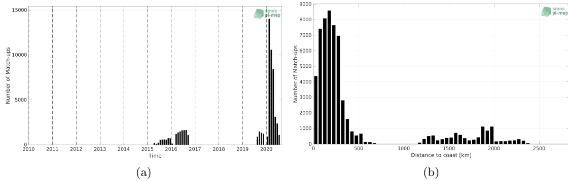
Figure 1: Number of match-ups between Surface drifters and SMAP SSS L3 v5 - Monthly (RSS) SSS as a function of time (a) and as function of the distance to coast (b) over the Atlantic Ocean Pi-MEP region and for the full satellite product period.
