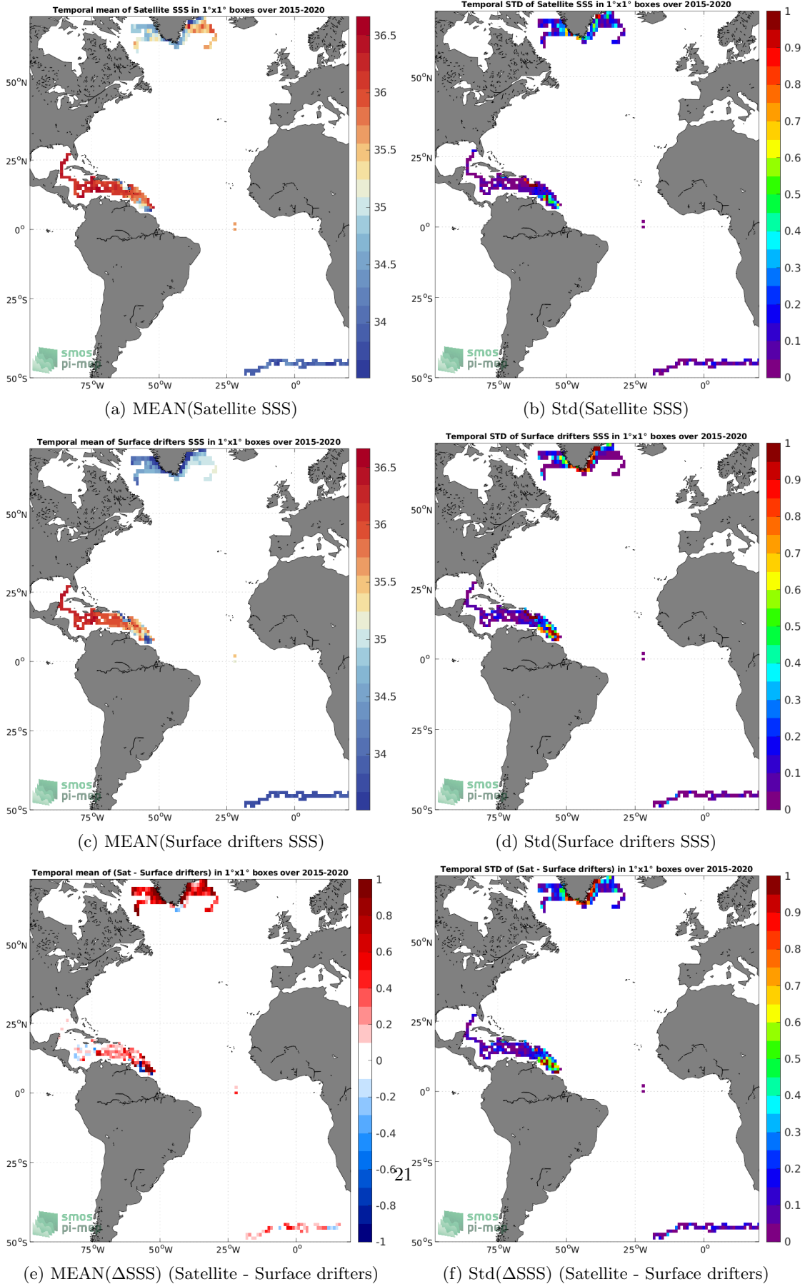
Figure 5: Temporal mean (left) and Std (right) of SSS from SMAP SSS L3 v5 - Monthly (RSS) (top), Surface drifters (middle), and of \Delta SSS (Satellite - Surface drifters). Only match-up pairs are used to generate these maps.
