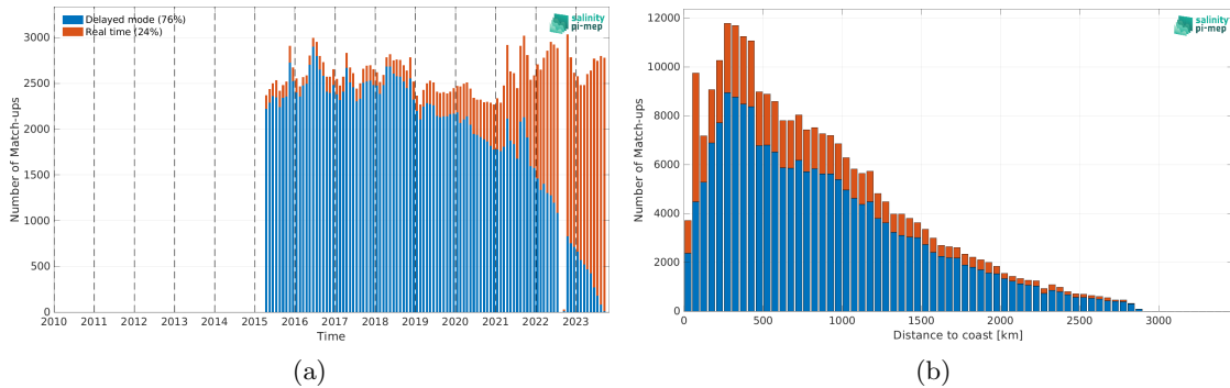
Figure 1: Number of match-ups between Argo and SMAP SSS L3 v5 - Monthly (RSS) SSS as a function of time (a) and as function of the distance to coast (b) over the Atlantic Ocean Pi-MEP region and for the full satellite product period.
