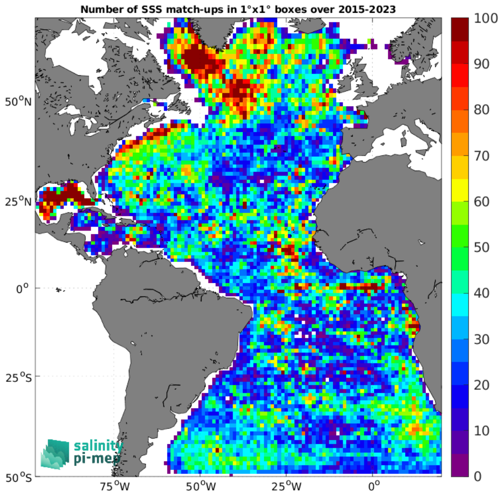
Figure 4: Number of SSS match-ups between Argo SSS and the SMAP SSS L3 v5 - Monthly (RSS) SSS product for the Atlantic Ocean Pi-MEP region over 1^\circ \times 1^\circ boxes and for the full satellite product period.
