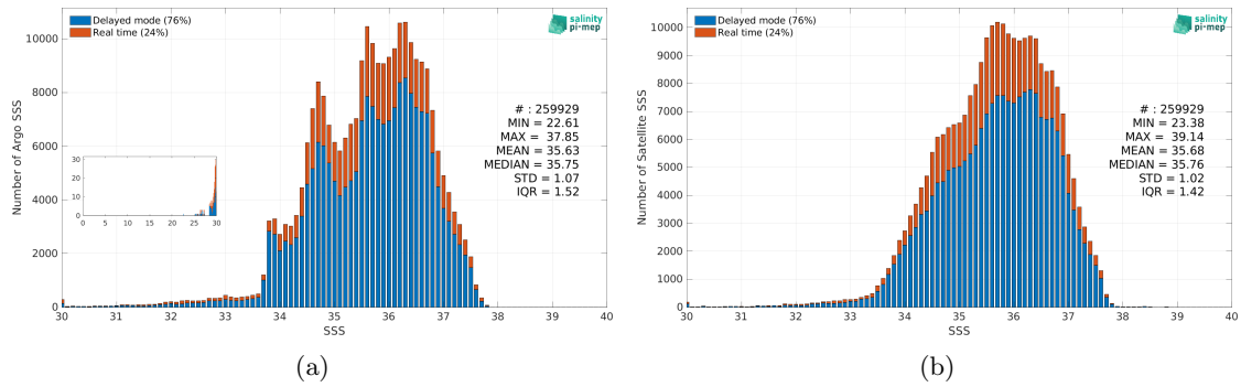
Figure 2: Histograms of SSS from Argo (a) and SMAP SSS L3 v5 - Monthly (RSS) (b) considering all match-up pairs per bins of 0.1 over the Atlantic Ocean Pi-MEP region and for the full satellite product period.
