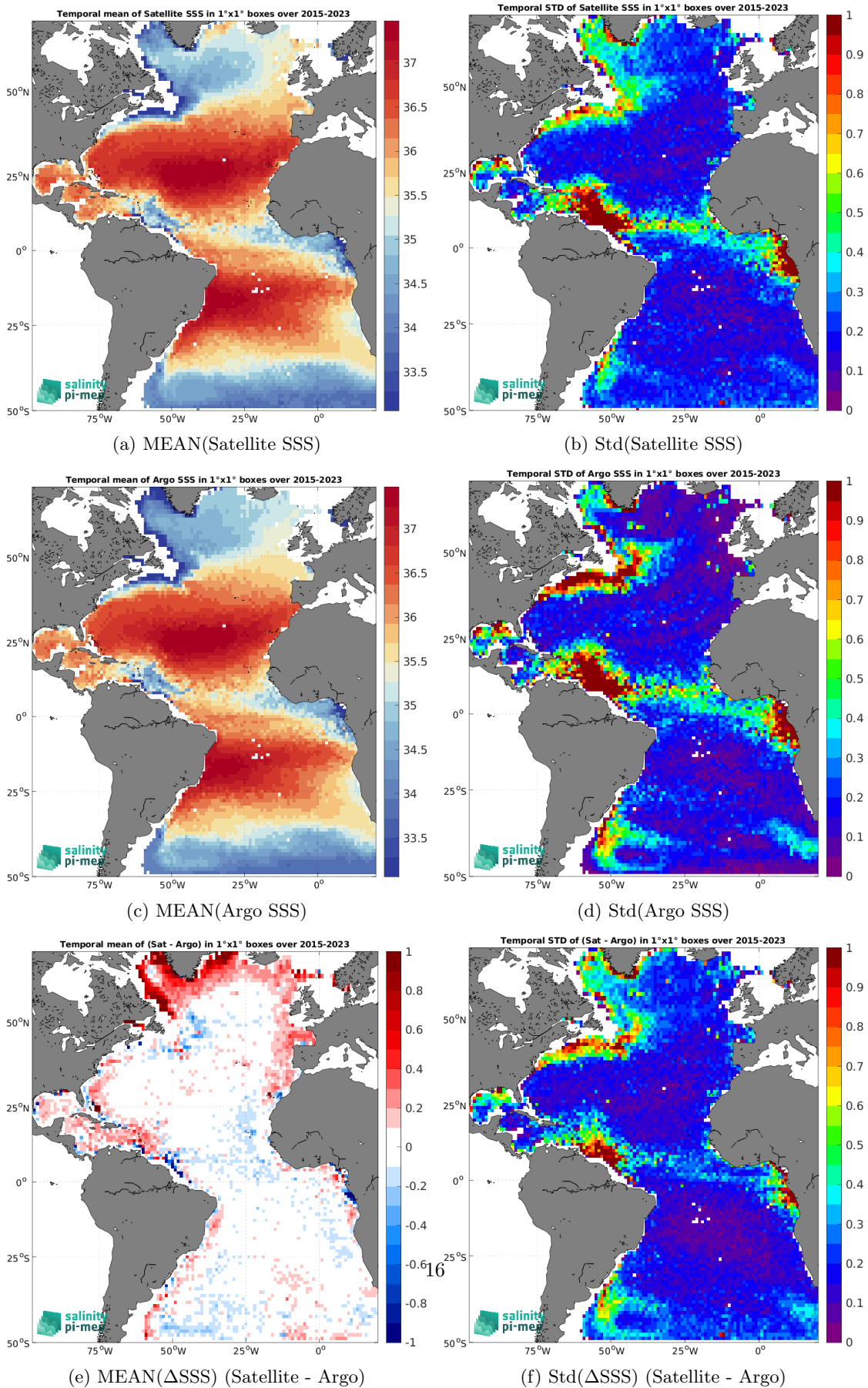
Figure 6: Temporal mean (left) and Std (right) of SSS from SMAP SSS L3 v5 - Monthly (RSS) (top), Argo (middle), and of \Delta SSS (Satellite - Argo). Only match-up pairs are used to generate these maps.
