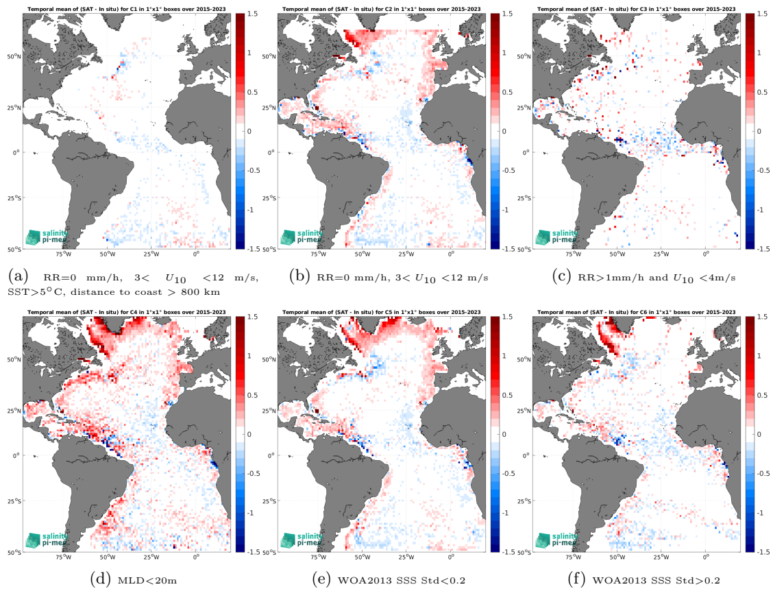
Figure 12: Temporal mean gridded over spatial boxes of size 1^\circ \times 1^\circ of \Delta SSS (SMAP SSS L3 v5 - Monthly (RSS) - Argo) for 6 different subdatasets corresponding to:RR=0 mm/h, 3 < U_{10} < 12 m/s, SST >5^\circ\text{C} , distance to coast > 800 km (a), RR=0 mm/h, 3 < U_{10} < 12 m/s (b), RR >1 mm/h and U_{10} < 4 m/s (c),MLD <20 m (d),WOA2013 SSS Std <0.2 (e),WOA2013 SSS Std >0.2 (f).
