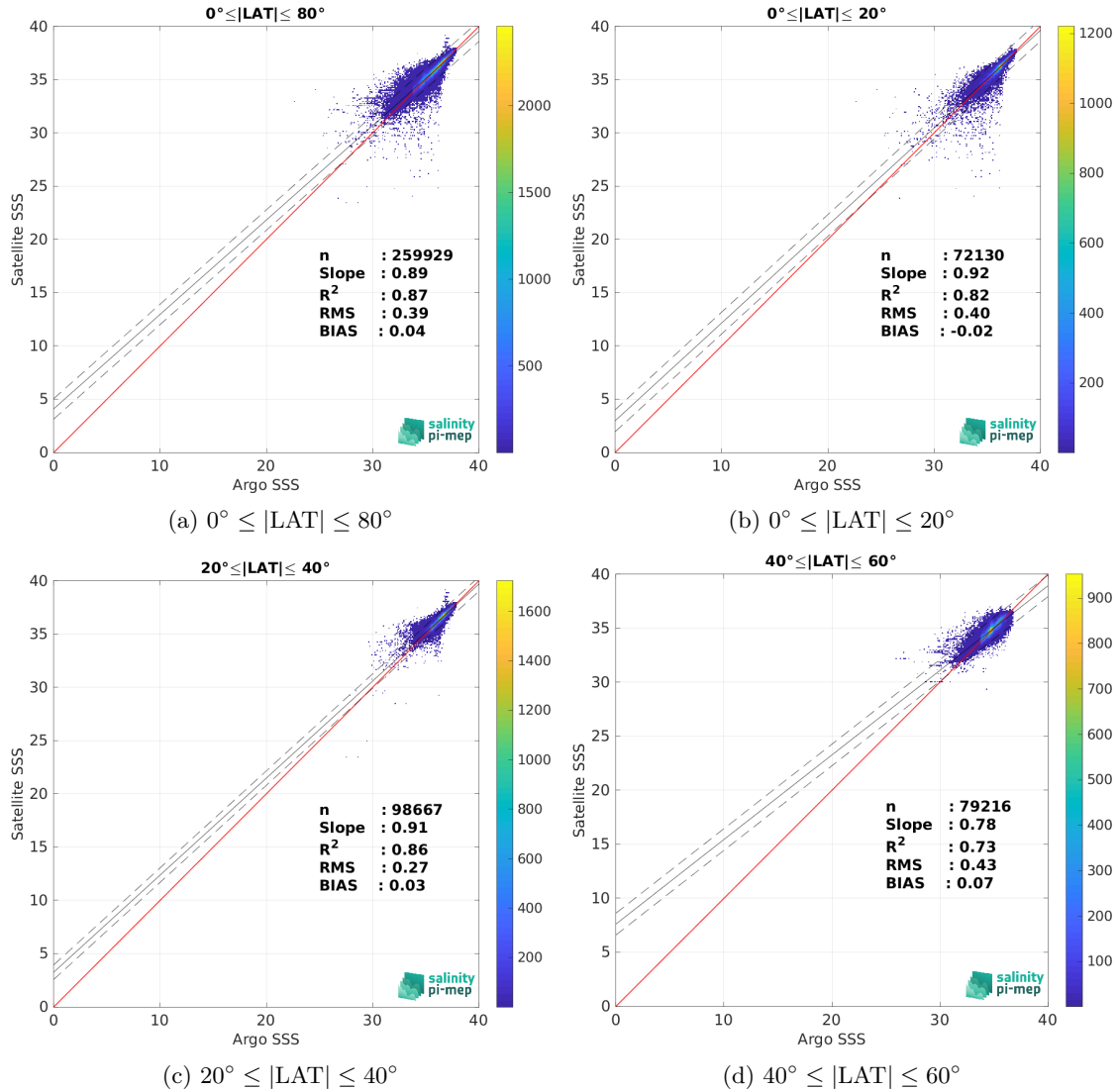
Figure 9: Contour maps of the concentration of SMAP SSS L3 v5 - Monthly (RSS) SSS (y-axis) versus Argo SSS (x-axis) at match-up pairs for different latitude bands. For each plot, the red line shows x=y . The black thin and dashed lines indicate a linear fit through the data cloud and the \pm 95\% confidence levels, respectively. The number match-up pairs n , the slope and R^2 coefficient of the linear fit, the root mean square (RMS) and the mean bias between satellite and in situ data are indicated for each latitude band in each plots.
