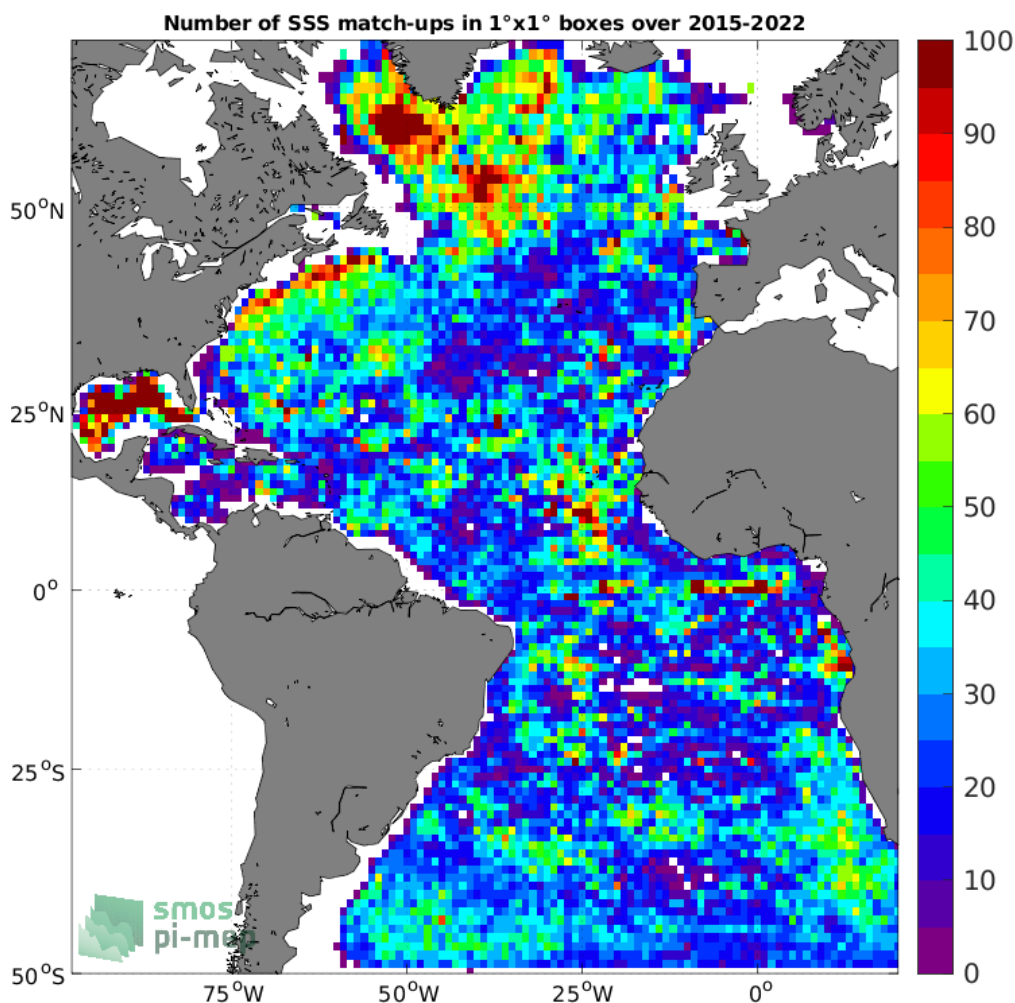
Figure 4: Number of SSS match-ups between Argo SSS and the SMAP SSS L3 v5 - Monthly (RSS) SSS product for the Atlantic Ocean Pi-MEP region over 1°x1° boxes and for the full satellite product period.
