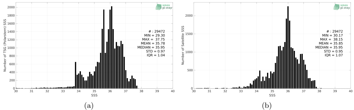
Figure 2: Histograms of SSS from TSG (Polarstern) (a) and SMAP SSS L3 v4 - 8-Day running (RSS) (b) considering all match-up pairs per bins of 0.1 over the Atlantic Ocean Pi-MEP region and for the full satellite product period.
