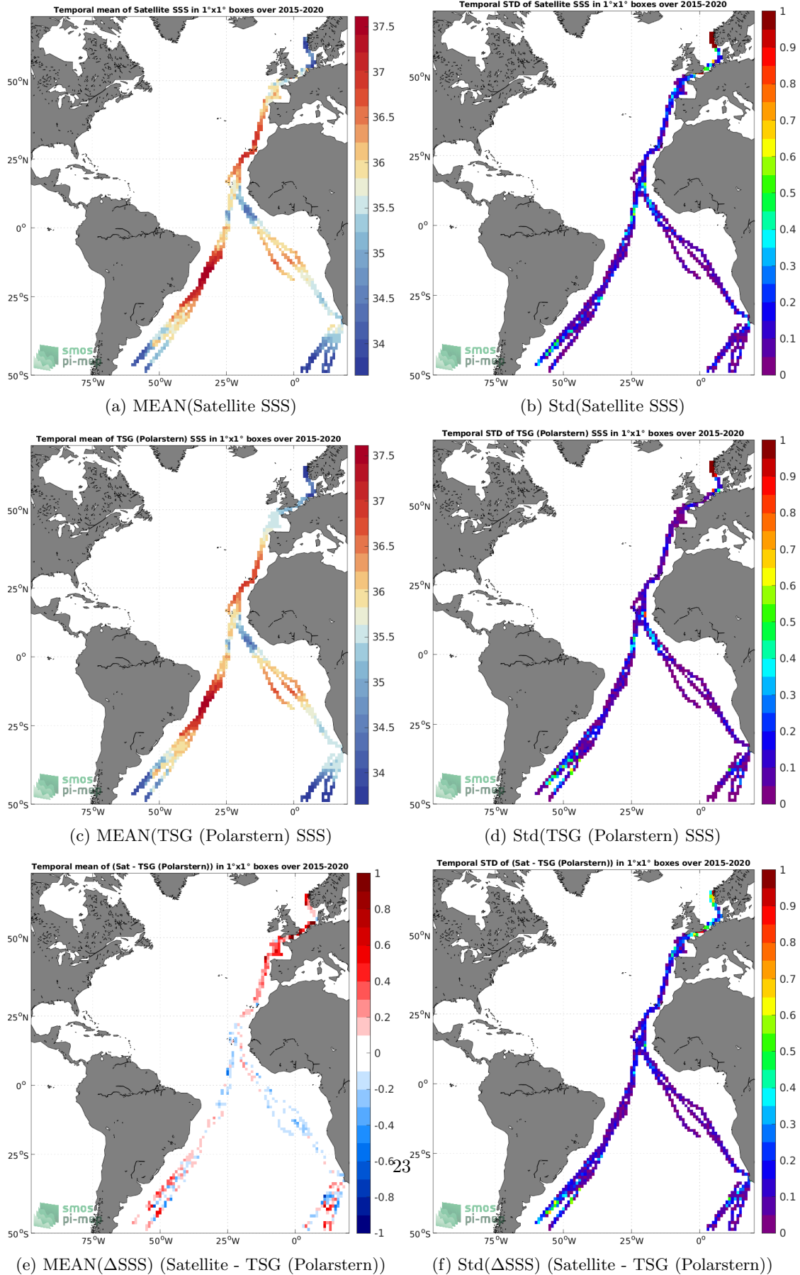
Figure 6: Temporal mean (left) and Std (right) of SSS from SMAP SSS L3 v4 - 8-Day running (RSS) (top), TSG (Polarstern) (middle), and of \Delta SSS (Satellite - TSG (Polarstern)). Only match-up pairs are used to generate these maps.
