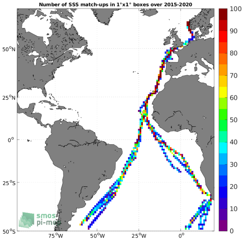
Figure 4: Number of SSS match-ups between TSG (Polarstern) SSS and the SMAP SSS L3 v4 - 8-Day running (RSS) SSS product for the Atlantic Ocean Pi-MEP region over 1°x1° boxes and for the full satellite product period.
