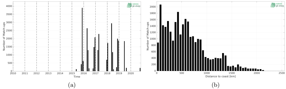
Figure 1: Number of match-ups between TSG (Polarstern) and SMAP SSS L3 v4 - 8-Day running (RSS) SSS as a function of time (a) and as function of the distance to coast (b) over the Atlantic Ocean Pi-MEP region and for the full satellite product period.
