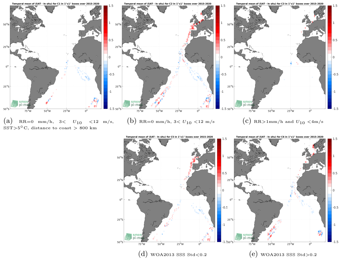
Figure 12: Temporal mean gridded over spatial boxes of size 1^\circ \times 1^\circ of \Delta SSS (SMAP SSS L3 v4 - 8-Day running (RSS) - TSG (Polarstern)) for 5 different subdatasets corresponding to:RR=0 mm/h, 3 < U_{10} < 12 m/s, SST >5^\circ\text{C} , distance to coast > 800 km (a), RR=0 mm/h, 3 < U_{10} < 12 m/s (b), RR >1 mm/h and U_{10} < 4 m/s (c), WOA2013 SSS Std <0.2 (d), WOA2013 SSS Std >0.2 (e).
