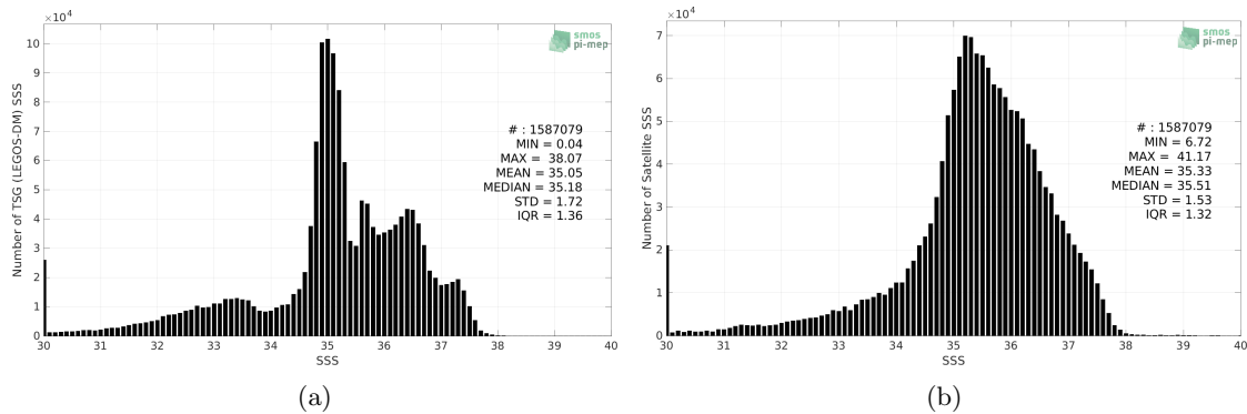
Figure 2: Histograms of SSS from TSG (LEGOS-DM) (a) and SMAP SSS L3 v4 - 8-Day running (RSS) (b) considering all match-up pairs per bins of 0.1 over the Atlantic Ocean Pi-MEP region and for the full satellite product period.
