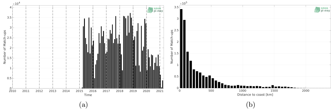
Figure 1: Number of match-ups between TSG (LEGOS-DM) and SMAP SSS L3 v4 - 8-Day running (RSS) SSS as a function of time (a) and as function of the distance to coast (b) over the Atlantic Ocean Pi-MEP region and for the full satellite product period.
