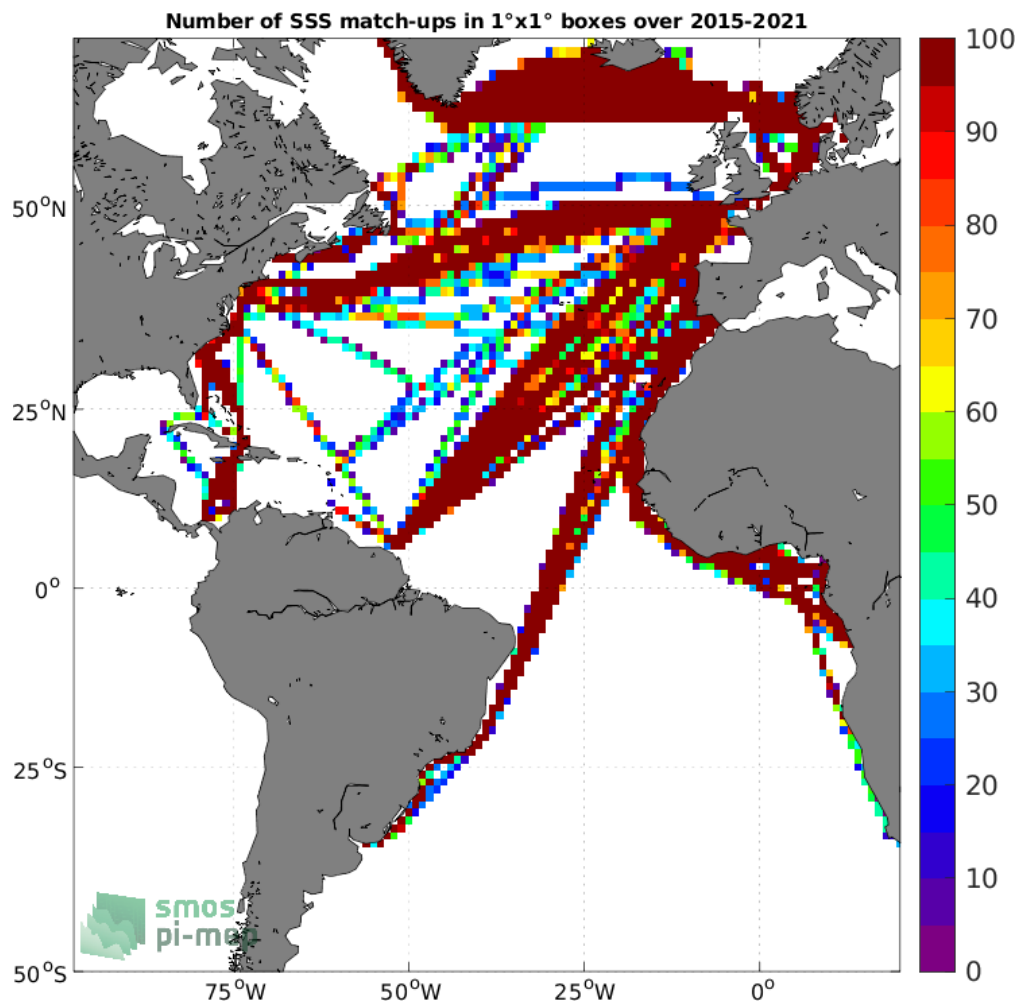
Figure 4: Number of SSS match-ups between TSG (LEGOS-DM) SSS and the SMAP SSS L3 v4 - 8-Day running (RSS) SSS product for the Atlantic Ocean Pi-MEP region over 1°×1° boxes and for the full satellite product period.
