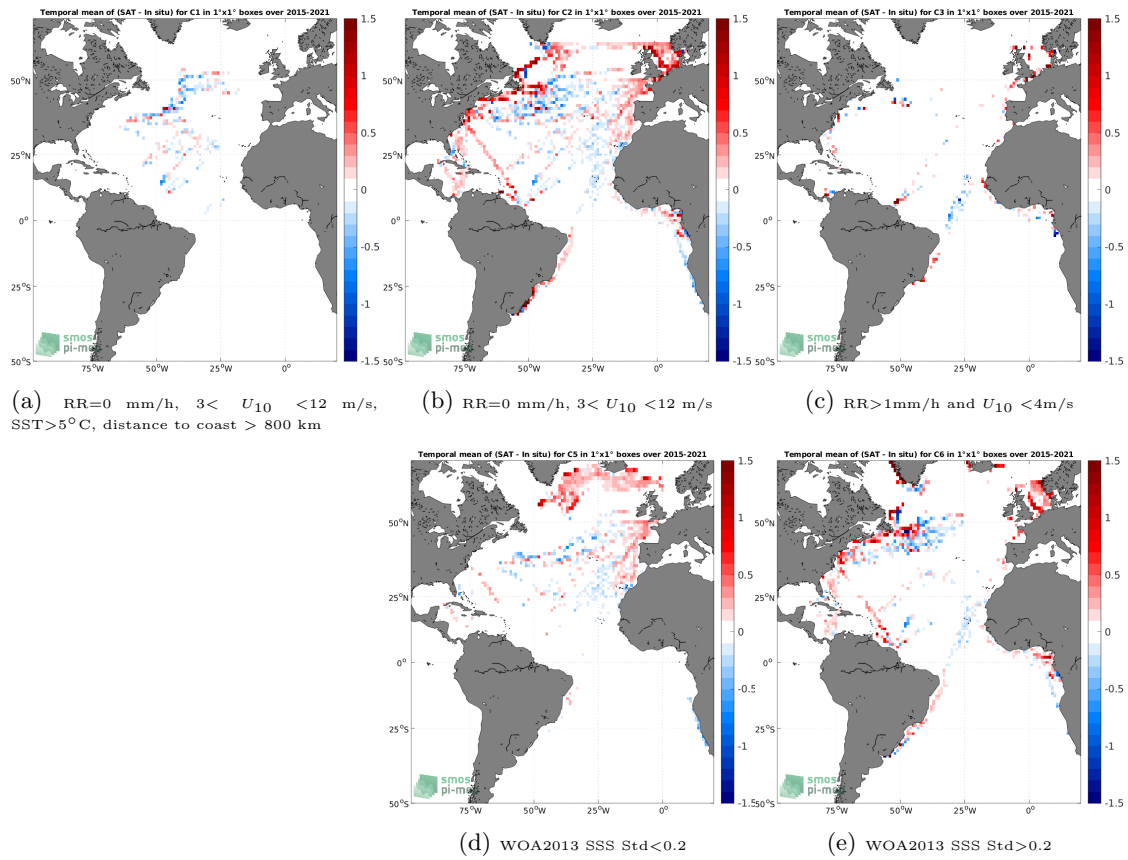
Figure 12: Temporal mean gridded over spatial boxes of size 1^\circ \times 1^\circ of \Delta SSS (SMAP SSS L3 v4 - 8-Day running (RSS) - TSG (LEGOS-DM)) for 5 different subdatasets corresponding to:RR=0 mm/h, 3 < U_{10} < 12 m/s, SST >5^\circ\text{C} , distance to coast > 800 km (a), RR=0 mm/h, 3 < U_{10} < 12 m/s (b), RR >1 mm/h and U_{10} < 4 m/s (c), WOA2013 SSS Std <0.2 (d), WOA2013 SSS Std >0.2 (e).
