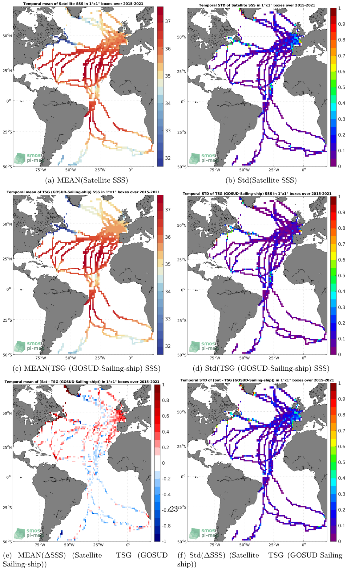
Figure 6: Temporal mean (left) and Std (right) of SSS from SMAP SSS L3 v4 - 8-Day running (RSS) (top), TSG (GOSUD-Sailing-ship) (middle), and of \Delta SSS (Satellite - TSG (GOSUD-Sailing-ship)). Only match-up pairs are used to generate these maps.
