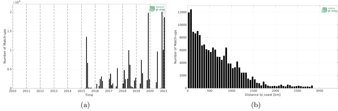
Figure 1: Number of match-ups between TSG (GOSUD-Sailing-ship) and SMAP SSS L3 v4 - 8-Day running (RSS) SSS as a function of time (a) and as function of the distance to coast (b) over the Atlantic Ocean Pi-MEP region and for the full satellite product period.
