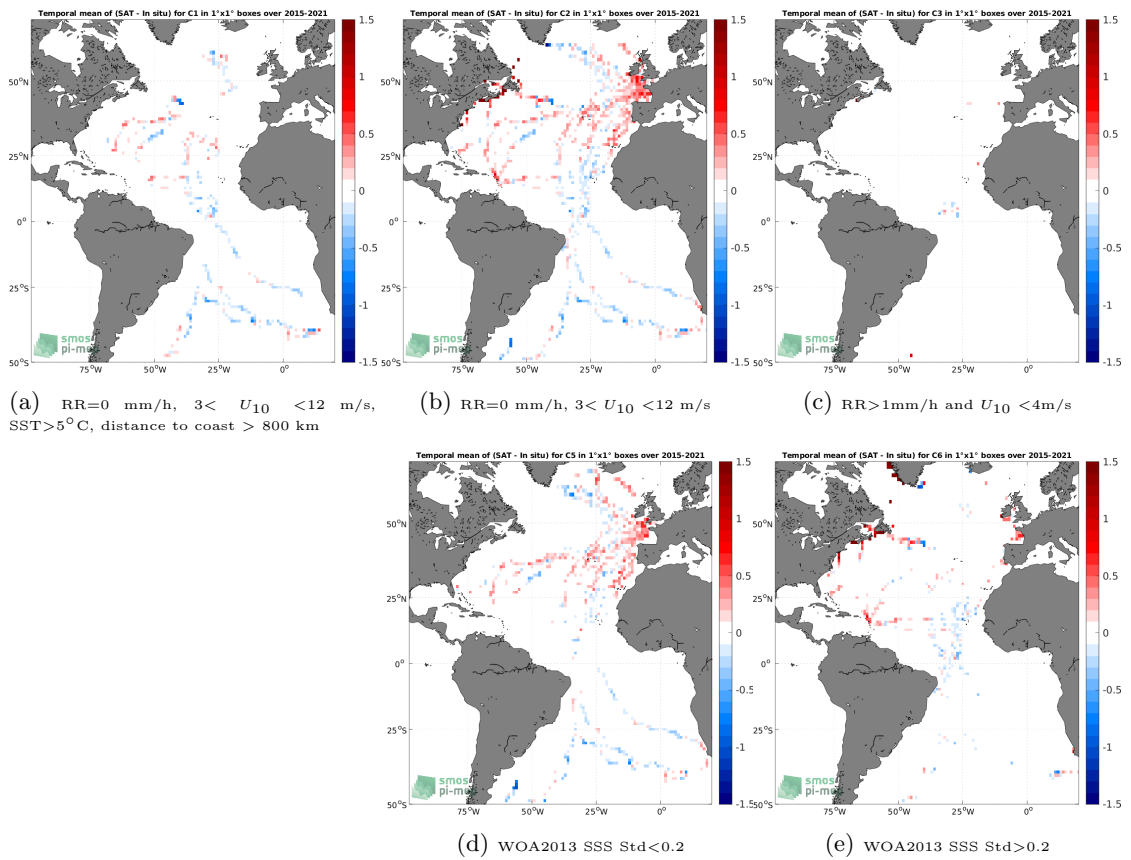
Figure 12: Temporal mean gridded over spatial boxes of size 1^\circ \times 1^\circ of \Delta SSS (SMAP SSS L3 v4 - 8-Day running (RSS) - TSG (GOSUD-Sailing-ship)) for 5 different subdatasets corresponding to:RR=0 mm/h, 3 < U_{10} < 12 m/s, SST>5°C, distance to coast > 800 km (a), RR=0 mm/h, 3 < U_{10} < 12 m/s (b), RR>1mm/h and U_{10} < 4 m/s (c), WOA2013 SSS Std<0.2 (d), WOA2013 SSS Std>0.2 (e).
