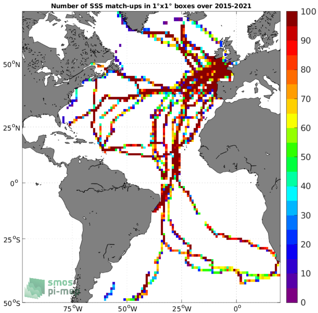
Figure 4: Number of SSS match-ups between TSG (GOSUD-Sailing-ship) SSS and the SMAP SSS L3 v4 - 8-Day running (RSS) SSS product for the Atlantic Ocean Pi-MEP region over 1°x1° boxes and for the full satellite product period.
