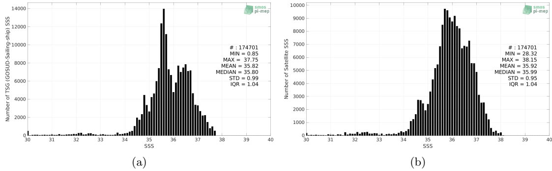
Figure 2: Histograms of SSS from TSG (GOSUD-Sailing-ship) (a) and SMAP SSS L3 v4 - 8-Day running (RSS) (b) considering all match-up pairs per bins of 0.1 over the Atlantic Ocean Pi-MEP region and for the full satellite product period.
