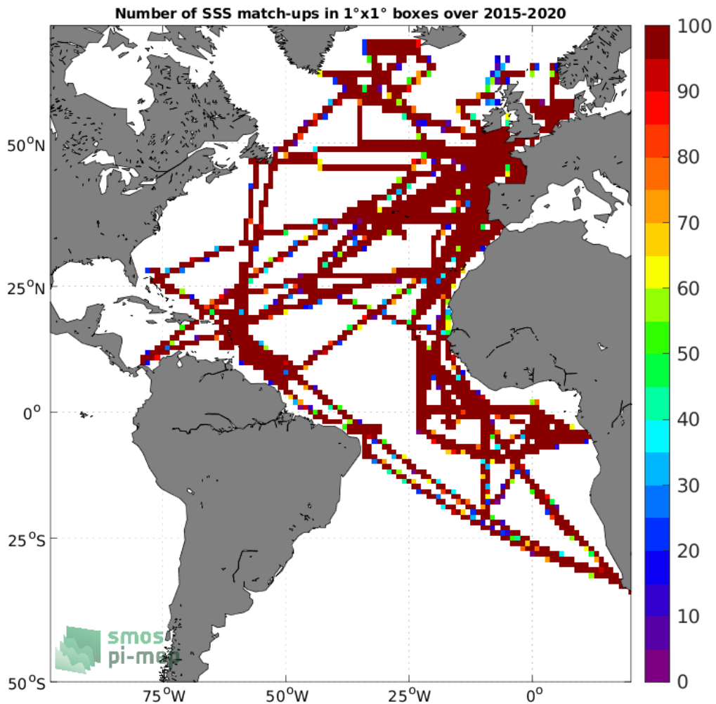
Figure 4: Number of SSS match-ups between TSG (GOSUD-Research-vessel) SSS and the SMAP SSS L3 v4 - 8-Day running (RSS) SSS product for the Atlantic Ocean Pi-MEP region over 1^\circ \times 1^\circ boxes and for the full satellite product period.
