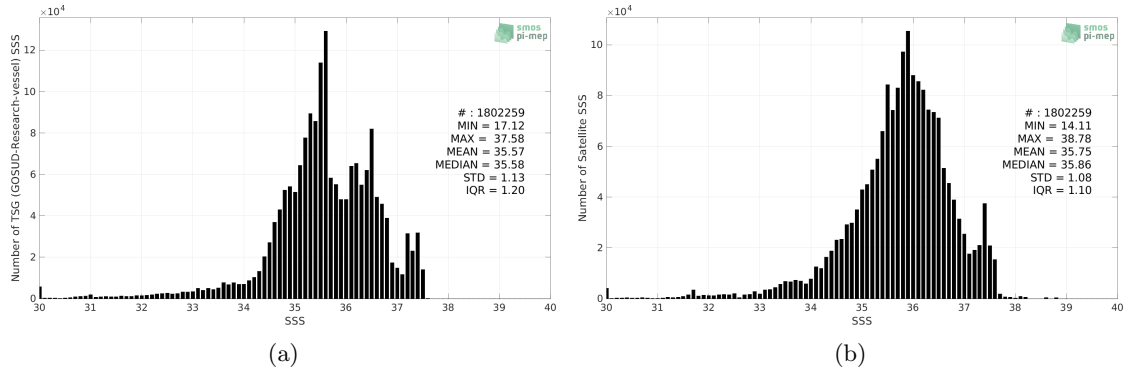
Figure 2: Histograms of SSS from TSG (GOSUD-Research-vessel) (a) and SMAP SSS L3 v4 - 8-Day running (RSS) (b) considering all match-up pairs per bins of 0.1 over the Atlantic Ocean Pi-MEP region and for the full satellite product period.
