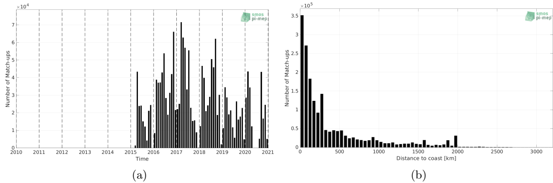
Figure 1: Number of match-ups between TSG (GOSUD-Research-vessel) and SMAP SSS L3 v4 - 8-Day running (RSS) SSS as a function of time (a) and as function of the distance to coast (b) over the Atlantic Ocean Pi-MEP region and for the full satellite product period.
