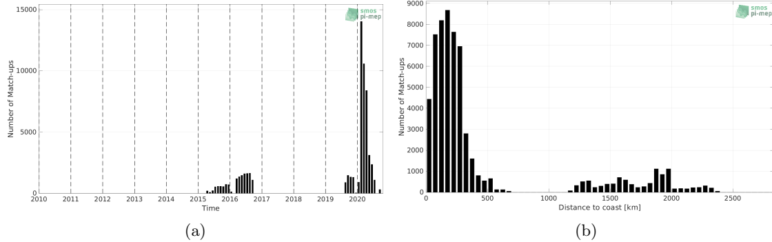
Figure 1: Number of match-ups between Surface drifters and SMAP SSS L3 v4 - 8-Day running (RSS) SSS as a function of time (a) and as function of the distance to coast (b) over the Atlantic Ocean Pi-MEP region and for the full satellite product period.
