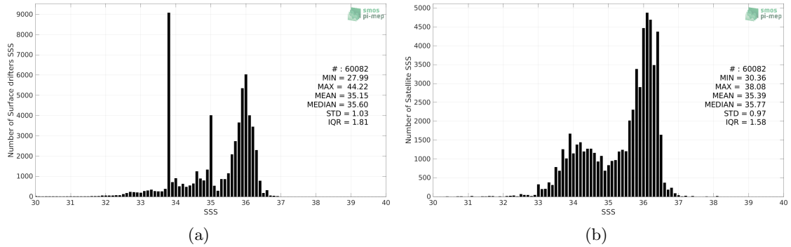
Figure 2: Histograms of SSS from Surface drifters (a) and SMAP SSS L3 v4 - 8-Day running (RSS) (b) considering all match-up pairs per bins of 0.1 over the Atlantic Ocean Pi-MEP region and for the full satellite product period.
