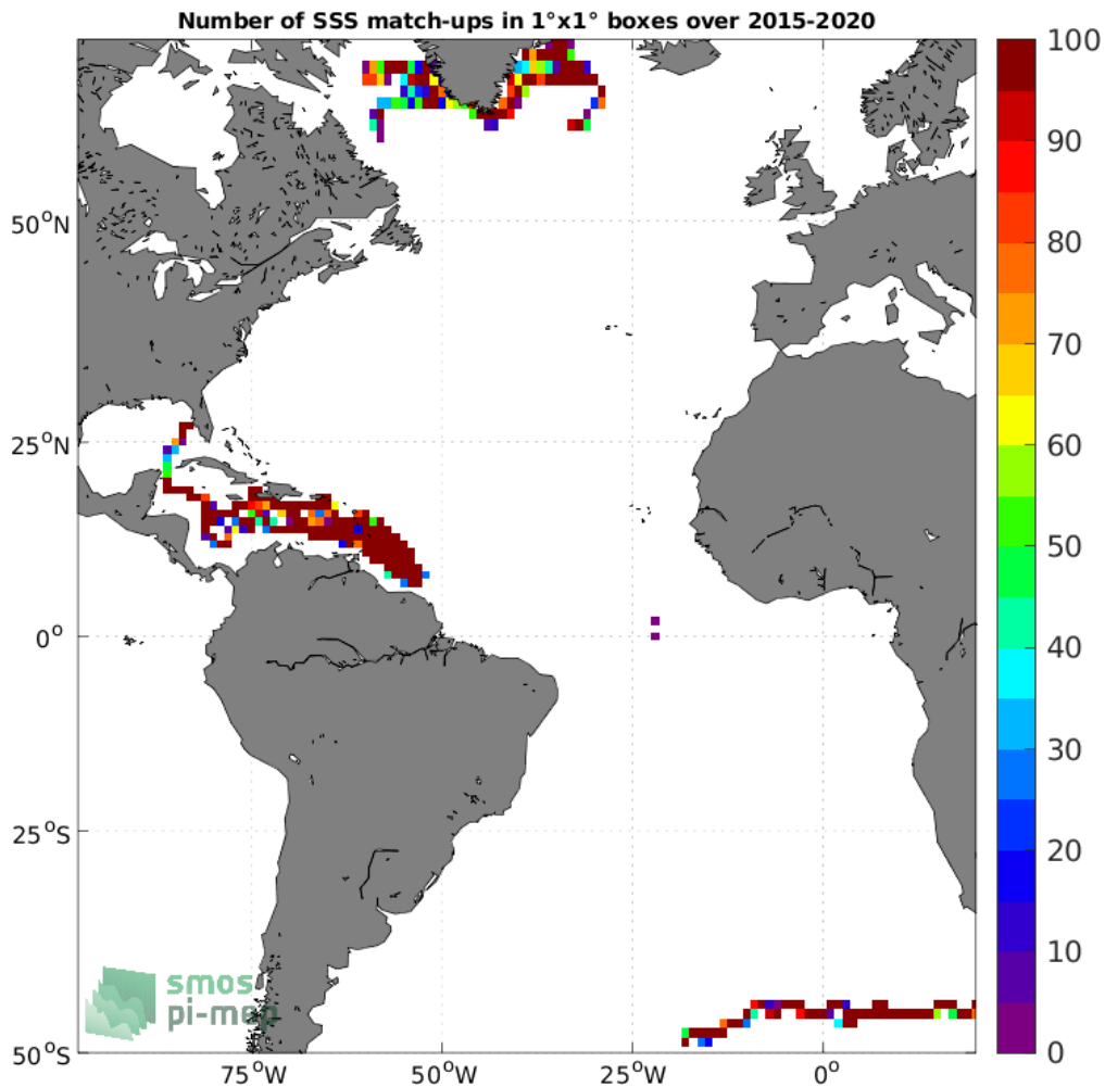
Figure 3: Number of SSS match-ups between Surface drifters SSS and the SMAP SSS L3 v4 - 8-Day running (RSS) SSS product for the Atlantic Ocean Pi-MEP region over 1°x1° boxes and for the full satellite product period.
