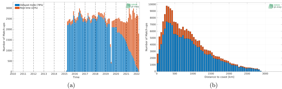
Figure 1: Number of match-ups between Argo and SMAP SSS L3 v4 - 8-Day running (RSS) SSS as a function of time (a) and as function of the distance to coast (b) over the Atlantic Ocean Pi-MEP region and for the full satellite product period.
