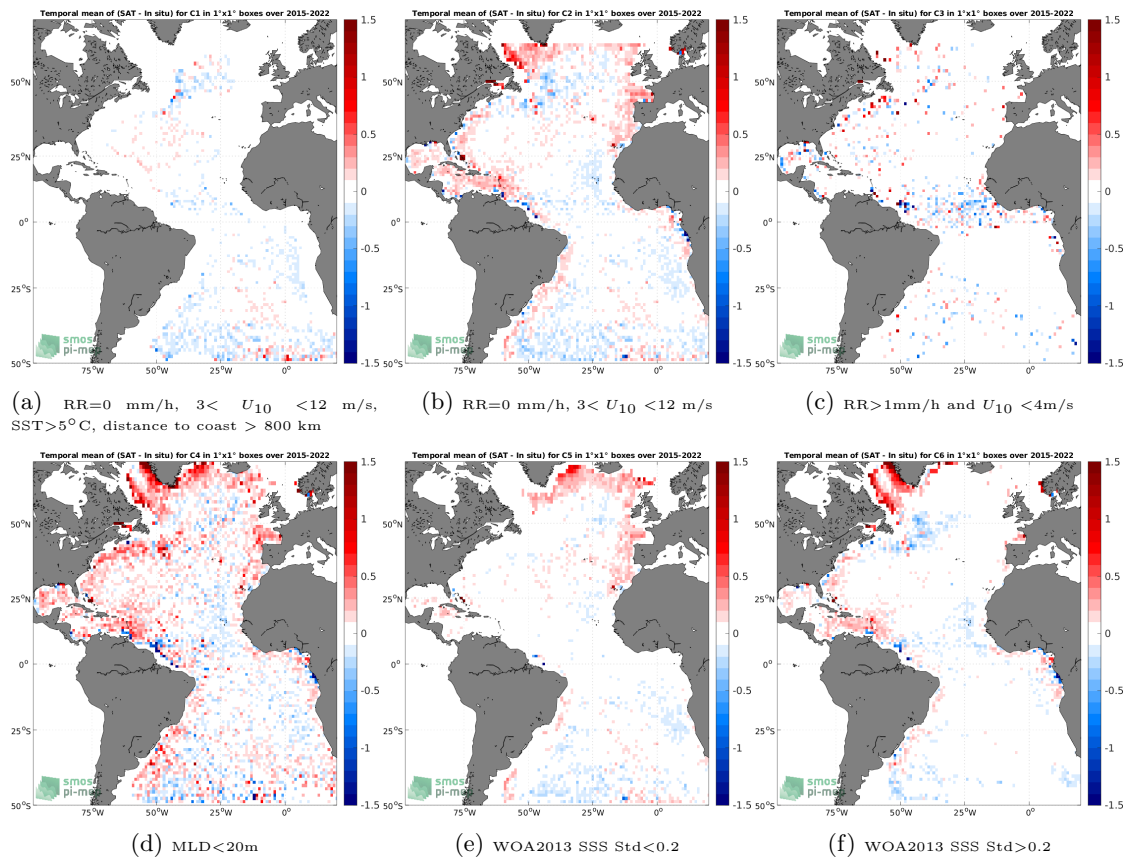
Figure 12: Temporal mean gridded over spatial boxes of size 1^\circ \times 1^\circ of \Delta SSS (SMAP SSS L3 v4 - 8-Day running (RSS) - Argo) for 6 different subdatasets corresponding to:RR=0 mm/h, 3 < U_{10} < 12 m/s, SST >5^\circ C, distance to coast > 800 km (a), RR=0 mm/h, 3 < U_{10} < 12 m/s (b), RR >1 mm/h and U_{10} < 4 m/s (c),MLD <20 m (d),WOA2013 SSS Std <0.2 (e),WOA2013 SSS Std >0.2 (f).
