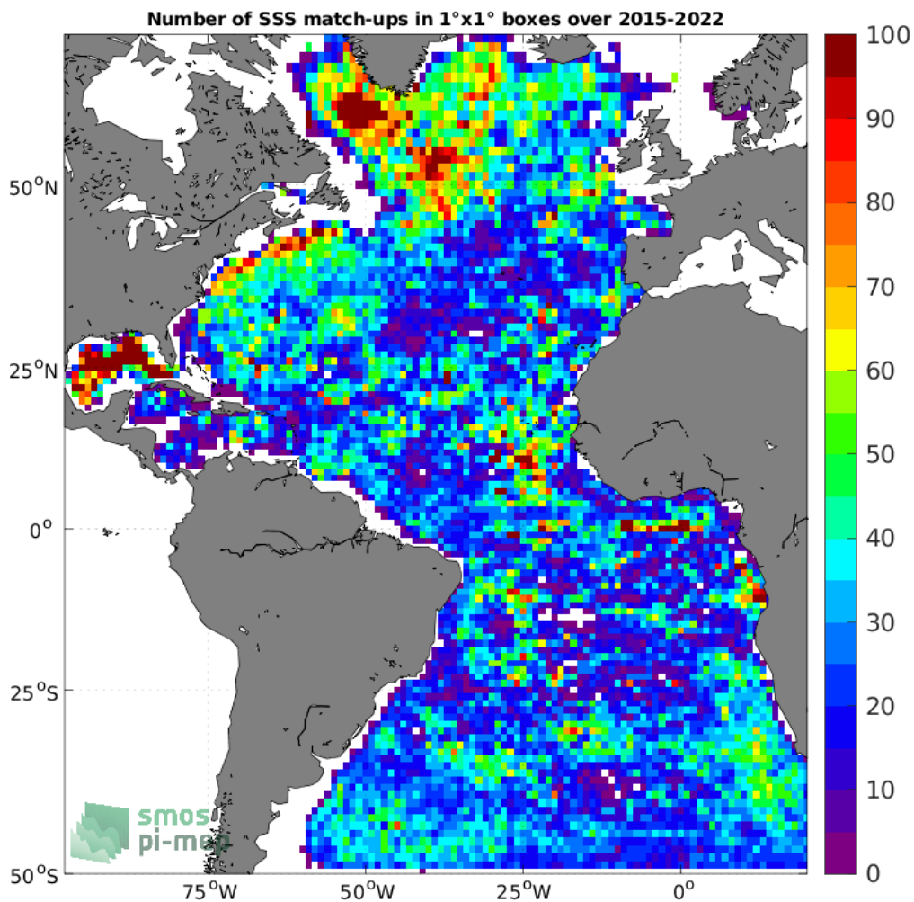
Figure 4: Number of SSS match-ups between Argo SSS and the SMAP SSS L3 v4 - 8-Day running (RSS) SSS product for the Atlantic Ocean Pi-MEP region over 1^\circ \times 1^\circ boxes and for the full satellite product period.
