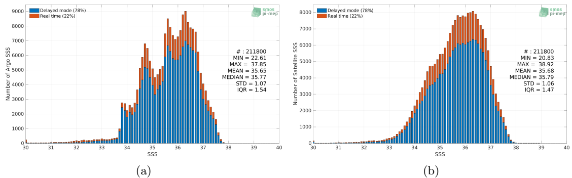
Figure 2: Histograms of SSS from Argo (a) and SMAP SSS L3 v4 - 8-Day running (RSS) (b) considering all match-up pairs per bins of 0.1 over the Atlantic Ocean Pi-MEP region and for the full satellite product period.
