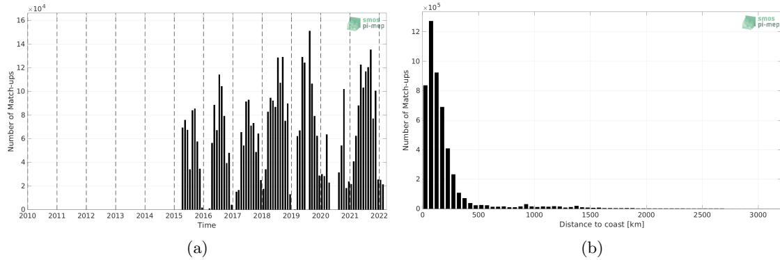
Figure 1: Number of match-ups between TSG (SAMOS) and SMAP SSS L3 v4 - Monthly (RSS) SSS as a function of time (a) and as function of the distance to coast (b) over the Atlantic Ocean Pi-MEP region and for the full satellite product period.
