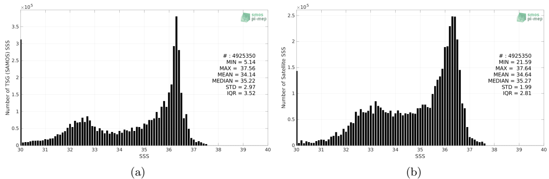
Figure 2: Histograms of SSS from TSG (SAMOS) (a) and SMAP SSS L3 v4 - Monthly (RSS) (b) considering all match-up pairs per bins of 0.1 over the Atlantic Ocean Pi-MEP region and for the full satellite product period.
