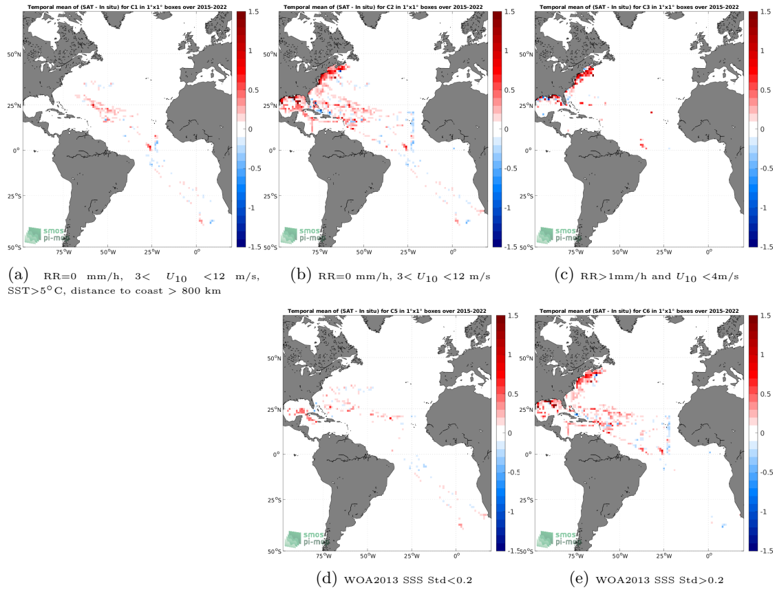
Figure 12: Temporal mean gridded over spatial boxes of size 1^\circ \times 1^\circ of \Delta SSS (SMAP SSS L3 v4 - Monthly (RSS) - TSG (SAMOS)) for 5 different subdatasets corresponding to:RR=0 mm/h, 3 < U_{10} < 12 m/s, SST >5^\circ\text{C} , distance to coast > 800 km (a), RR=0 mm/h, 3 < U_{10} < 12 m/s (b), RR >1 mm/h and U_{10} < 4 m/s (c), WOA2013 SSS Std <0.2 (d), WOA2013 SSS Std >0.2 (e).
