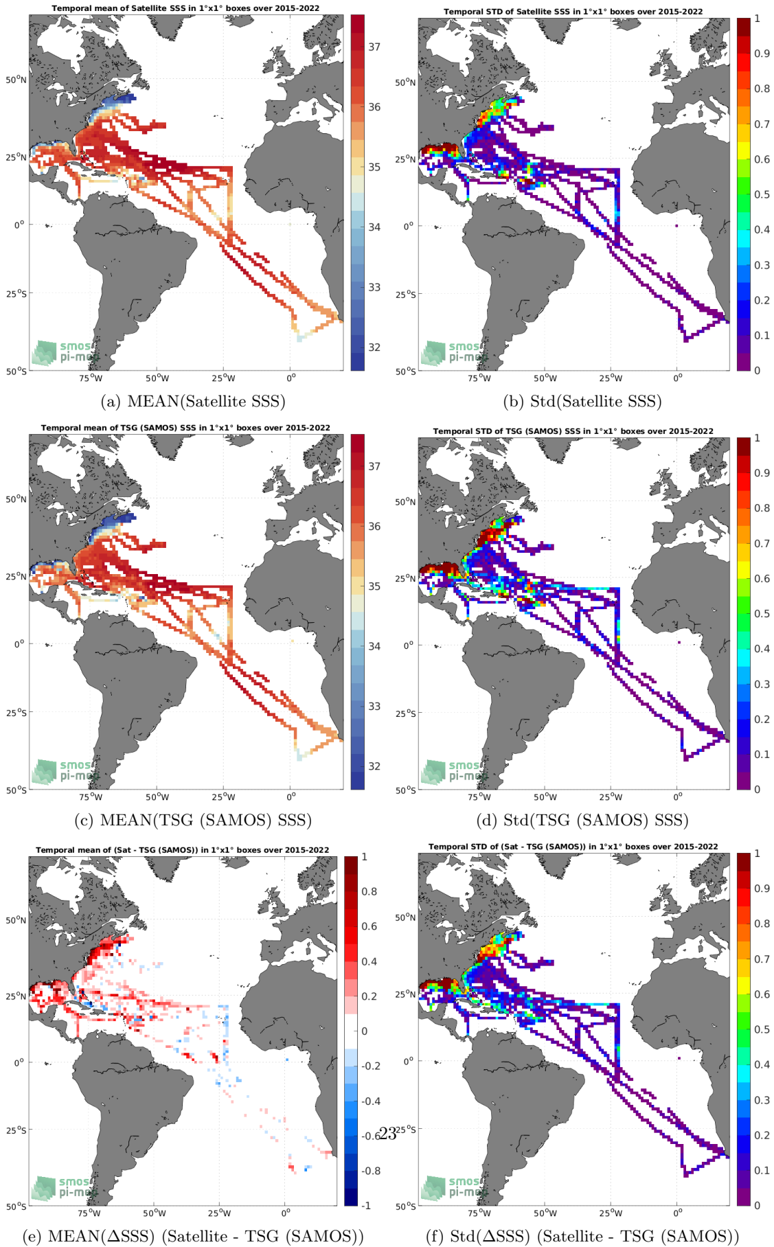
Figure 6: Temporal mean (left) and Std (right) of SSS from SMAP SSS L3 v4 - Monthly (RSS) (top), TSG (SAMOS) (middle), and of \Delta SSS (Satellite - TSG (SAMOS)). Only match-up pairs are used to generate these maps.
