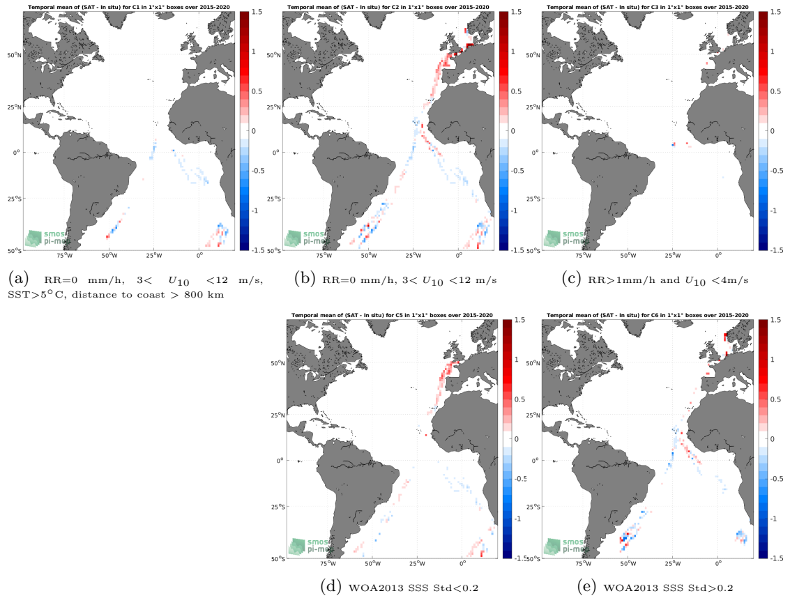
Figure 12: Temporal mean gridded over spatial boxes of size 1^\circ \times 1^\circ of \Delta SSS (SMAP SSS L3 v4 - Monthly (RSS) - TSG (Polarstern)) for 5 different subdatasets corresponding to:RR=0 mm/h, 3 < U_{10} < 12 m/s, SST >5^\circ\text{C} , distance to coast > 800 km (a), RR=0 mm/h, 3 < U_{10} < 12 m/s (b), RR >1 mm/h and U_{10} < 4 m/s (c), WOA2013 SSS Std <0.2 (d), WOA2013 SSS Std >0.2 (e).
