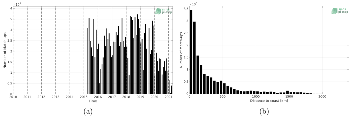
Figure 1: Number of match-ups between TSG (LEGOS-DM) and SMAP SSS L3 v4 - Monthly (RSS) SSS as a function of time (a) and as function of the distance to coast (b) over the Atlantic Ocean Pi-MEP region and for the full satellite product period.
