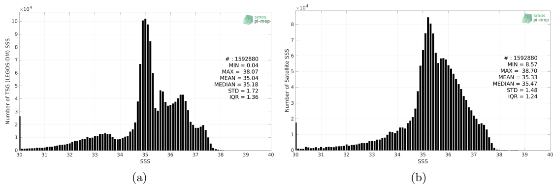
Figure 2: Histograms of SSS from TSG (LEGOS-DM) (a) and SMAP SSS L3 v4 - Monthly (RSS) (b) considering all match-up pairs per bins of 0.1 over the Atlantic Ocean Pi-MEP region and for the full satellite product period.
