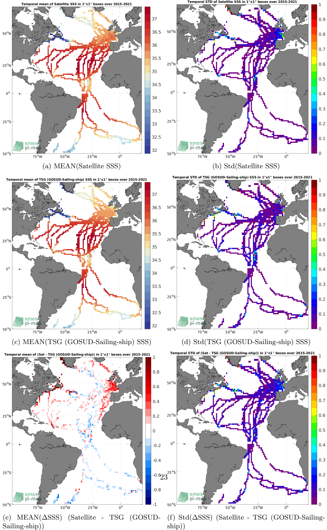
Figure 6: Temporal mean (left) and Std (right) of SSS from SMAP SSS L3 v4 - Monthly (RSS) (top), TSG (GOSUD-Sailing-ship) (middle), and of \Delta SSS (Satellite - TSG (GOSUD-Sailing-ship)). Only match-up pairs are used to generate these maps.
