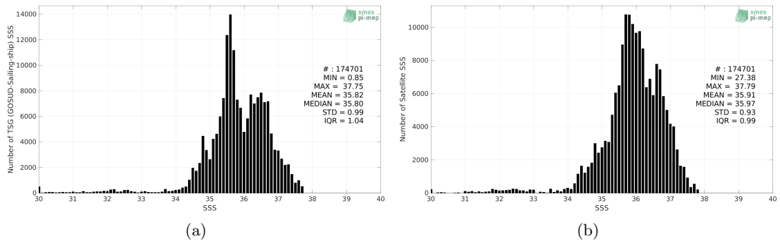
Figure 2: Histograms of SSS from TSG (GOSUD-Sailing-ship) (a) and SMAP SSS L3 v4 - Monthly (RSS) (b) considering all match-up pairs per bins of 0.1 over the Atlantic Ocean Pi-MEP region and for the full satellite product period.
