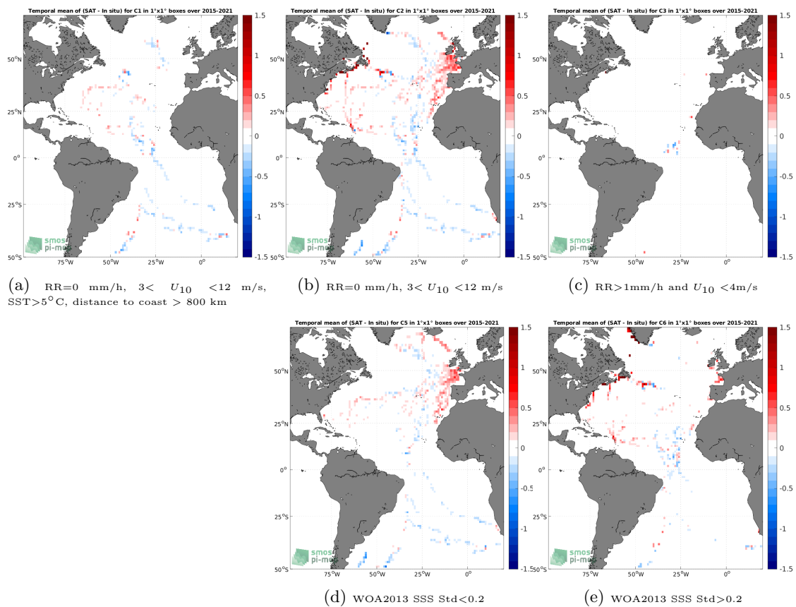
Figure 12: Temporal mean gridded over spatial boxes of size 1^\circ \times 1^\circ of \Delta SSS (SMAP SSS L3 v4 - Monthly (RSS) - TSG (GOSUD-Sailing-ship)) for 5 different subdatasets corresponding to:RR=0 mm/h, 3 < U_{10} < 12 m/s, SST>5°C, distance to coast > 800 km (a), RR=0 mm/h, 3 < U_{10} < 12 m/s (b), RR>1mm/h and U_{10} < 4 m/s (c), WOA2013 SSS Std<0.2 (d), WOA2013 SSS Std>0.2 (e).
