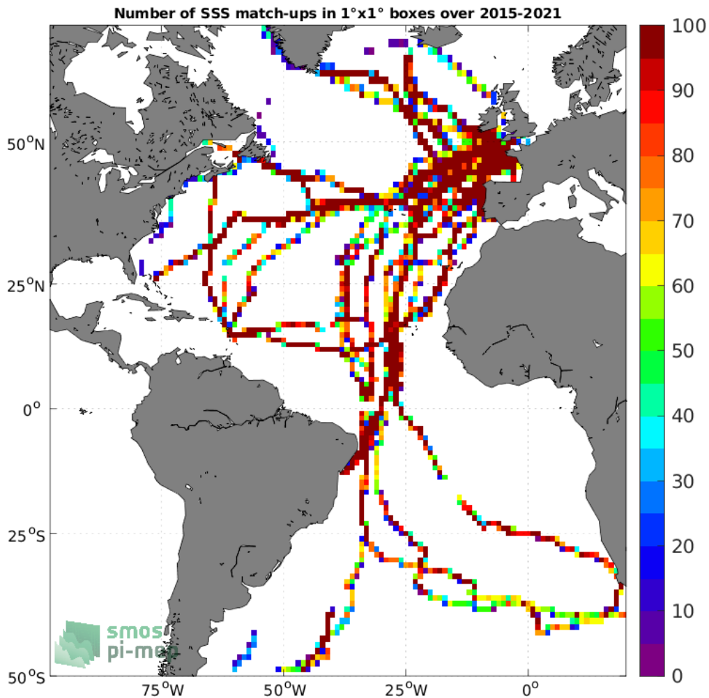
Figure 4: Number of SSS match-ups between TSG (GOSUD-Sailing-ship) SSS and the SMAP SSS L3 v4 - Monthly (RSS) SSS product for the Atlantic Ocean Pi-MEP region over 1°x1° boxes and for the full satellite product period.
