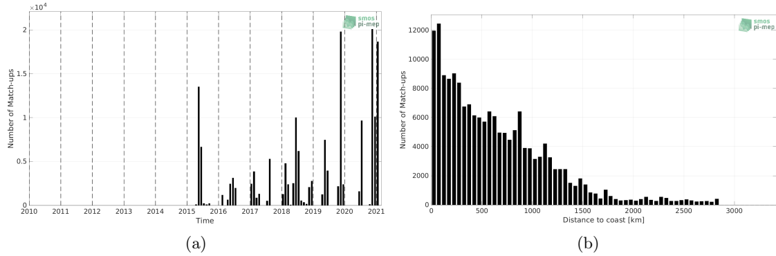
Figure 1: Number of match-ups between TSG (GOSUD-Sailing-ship) and SMAP SSS L3 v4 - Monthly (RSS) SSS as a function of time (a) and as function of the distance to coast (b) over the Atlantic Ocean Pi-MEP region and for the full satellite product period.
