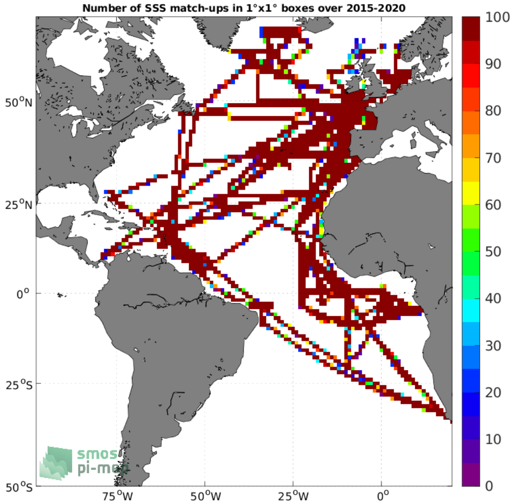
Figure 4: Number of SSS match-ups between TSG (GOSUD-Research-vessel) SSS and the SMAP SSS L3 v4 - Monthly (RSS) SSS product for the Atlantic Ocean Pi-MEP region over 1^\circ \times 1^\circ boxes and for the full satellite product period.
