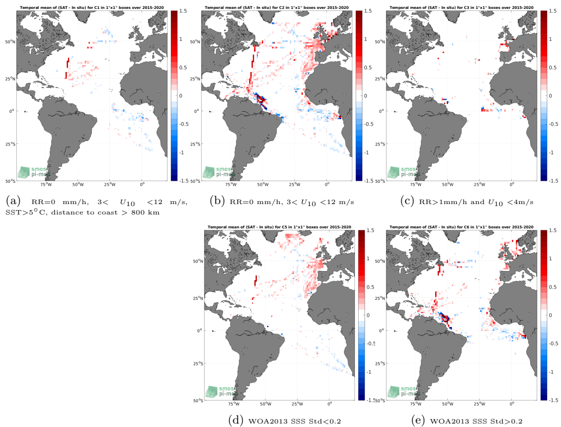
Figure 12: Temporal mean gridded over spatial boxes of size 1^\circ \times 1^\circ of \Delta SSS (SMAP SSS L3 v4 - Monthly (RSS) - TSG (GOSUD-Research-vessel)) for 5 different subdatasets corresponding to:RR=0 mm/h, 3 < U_{10} < 12 m/s, SST>5°C, distance to coast > 800 km (a), RR=0 mm/h, 3 < U_{10} < 12 m/s (b), RR>1mm/h and U_{10} < 4 m/s (c), WOA2013 SSS Std<0.2 (d), WOA2013 SSS Std>0.2 (e).
