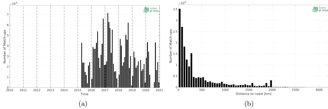
Figure 1: Number of match-ups between TSG (GOSUD-Research-vessel) and SMAP SSS L3 v4 - Monthly (RSS) SSS as a function of time (a) and as function of the distance to coast (b) over the Atlantic Ocean Pi-MEP region and for the full satellite product period.
