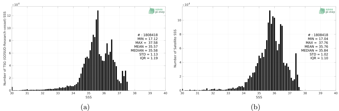
Figure 2: Histograms of SSS from TSG (GOSUD-Research-vessel) (a) and SMAP SSS L3 v4 - Monthly (RSS) (b) considering all match-up pairs per bins of 0.1 over the Atlantic Ocean Pi-MEP region and for the full satellite product period.
