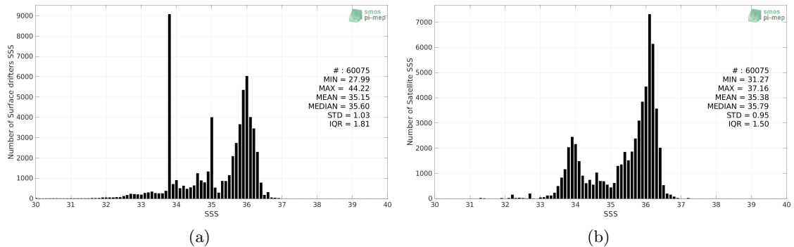
Figure 2: Histograms of SSS from Surface drifters (a) and SMAP SSS L3 v4 - Monthly (RSS) (b) considering all match-up pairs per bins of 0.1 over the Atlantic Ocean Pi-MEP region and for the full satellite product period.
