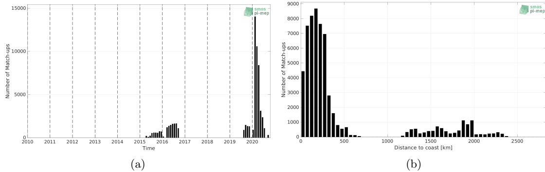
Figure 1: Number of match-ups between Surface drifters and SMAP SSS L3 v4 - Monthly (RSS) SSS as a function of time (a) and as function of the distance to coast (b) over the Atlantic Ocean Pi-MEP region and for the full satellite product period.
