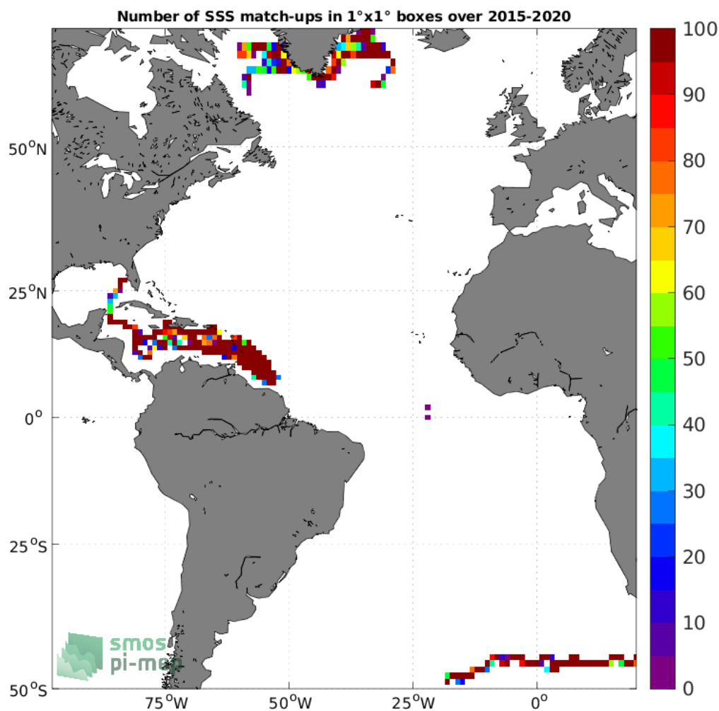
Figure 3: Number of SSS match-ups between Surface drifters SSS and the SMAP SSS L3 v4 - Monthly (RSS) SSS product for the Atlantic Ocean Pi-MEP region over 1°x1° boxes and for the full satellite product period.
