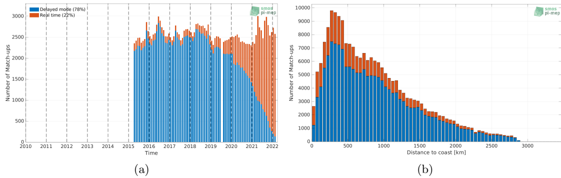
Figure 1: Number of match-ups between Argo and SMAP SSS L3 v4 - Monthly (RSS) SSS as a function of time (a) and as function of the distance to coast (b) over the Atlantic Ocean Pi-MEP region and for the full satellite product period.
