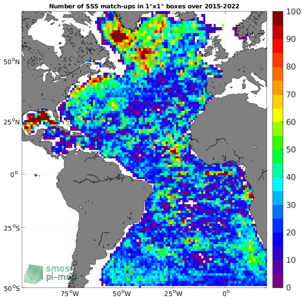
Figure 4: Number of SSS match-ups between Argo SSS and the SMAP SSS L3 v4 - Monthly (RSS) SSS product for the Atlantic Ocean Pi-MEP region over 1°x1° boxes and for the full satellite product period.
