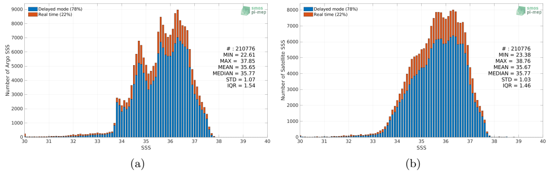
Figure 2: Histograms of SSS from Argo (a) and SMAP SSS L3 v4 - Monthly (RSS) (b) considering all match-up pairs per bins of 0.1 over the Atlantic Ocean Pi-MEP region and for the full satellite product period.
