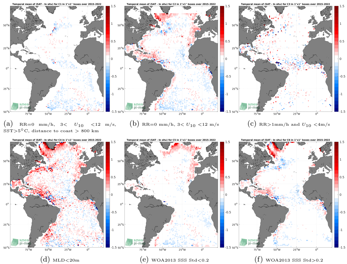
Figure 12: Temporal mean gridded over spatial boxes of size 1^\circ \times 1^\circ of \Delta SSS (SMAP SSS L3 v4 - Monthly (RSS) - Argo) for 6 different subdatasets corresponding to:RR=0 mm/h, 3 < U_{10} < 12 m/s, SST > 5^\circ\text{C} , distance to coast > 800 km (a), RR=0 mm/h, 3 < U_{10} < 12 m/s (b), RR > 1 mm/h and U_{10} < 4 m/s (c),MLD < 20 m (d),WOA2013 SSS Std < 0.2 (e),WOA2013 SSS Std > 0.2 (f).
