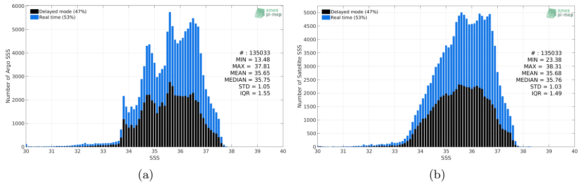
Figure 2: Histograms of SSS from Argo (a) and SMAP-L3-RSS-V4-MONTHLY (b) considering all match-up pairs per bins of 0.1 over the Atlantic Ocean Pi-MEP region and for the full satellite product period.
