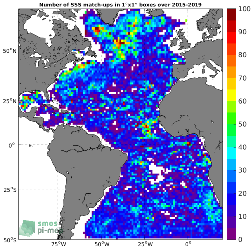
Figure 4: Number of SSS match-ups between Argo SSS and the SMAP-L3-RSS-V4-MONTHLY SSS product for the Atlantic Ocean Pi-MEP region over 1°x1° boxes and for the full satellite product period.
