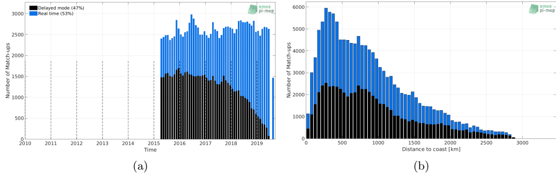
Figure 1: Number of match-ups between Argo and SMAP-L3-RSS-V4-MONTHLY SSS as a function of time (a) and as function of the distance to coast (b) over the Atlantic Ocean Pi-MEP region and for the full satellite product period.
