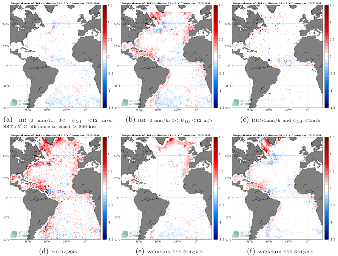
Figure 12: Temporal mean gridded over spatial boxes of size 1°x1° of \Delta SSS (SMAP-L3-RSS-V4-MONTHLY - Argo) for 6 different subdatasets corresponding to:RR=0 mm/h, 3 < U_{10} < 12 m/s, SST>5°C, distance to coast > 800 km (a), RR=0 mm/h, 3 < U_{10} < 12 m/s (b), RR>1mm/h and U_{10} < 4 m/s (c),MLD<20m (d),WOA2013 SSS Std<0.2 (e),WOA2013 SSS Std>0.2 (f).
