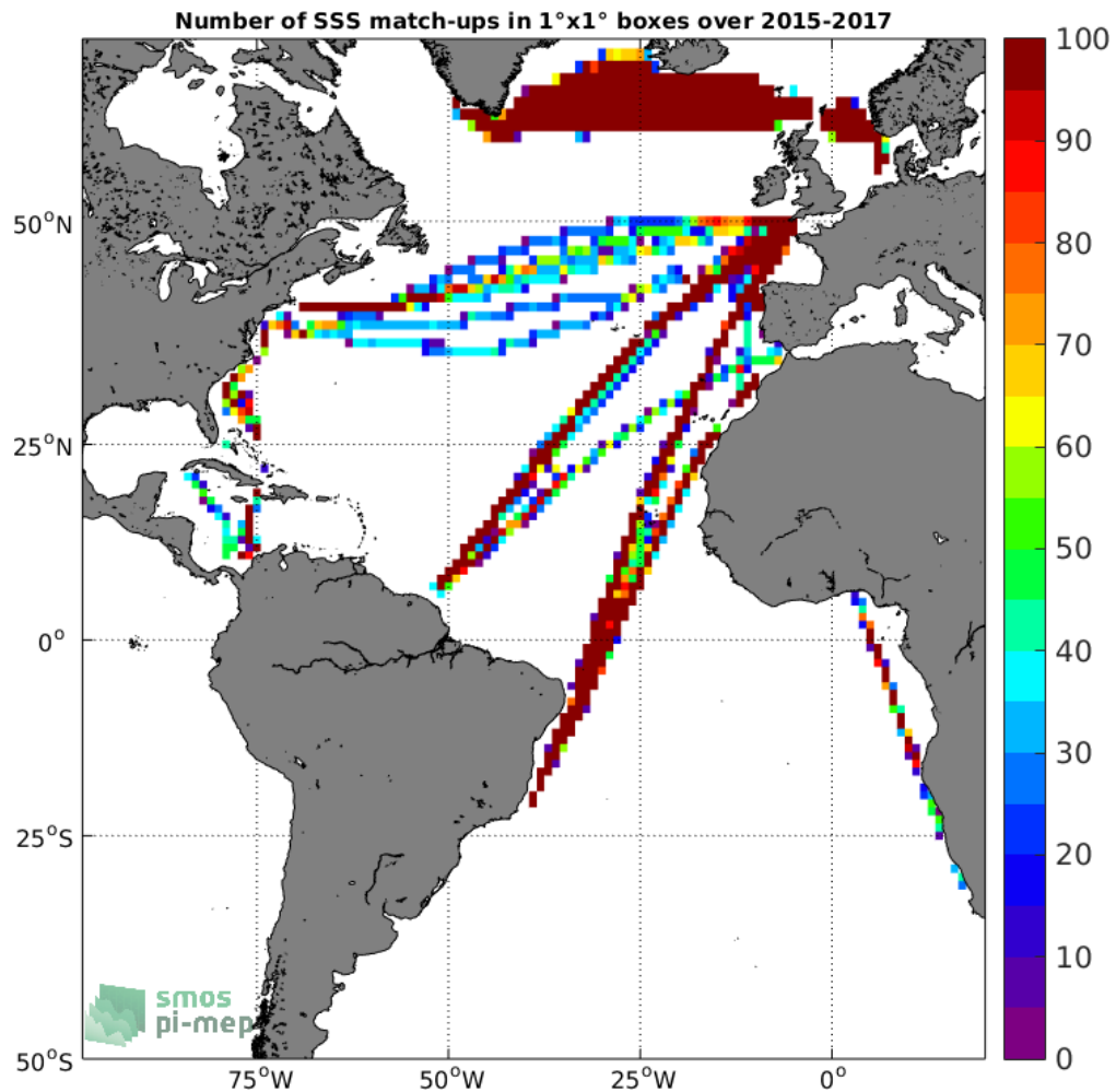
Figure 4: Number of SSS match-ups between TSG-LEGOS-DM SSS and the SMAP-L3-RSS-V3-8DAY-RUNNING-70KM SSS product for the Atlantic Ocean Pi-MEP region over 1°x1° boxes and for the full satellite product period.
