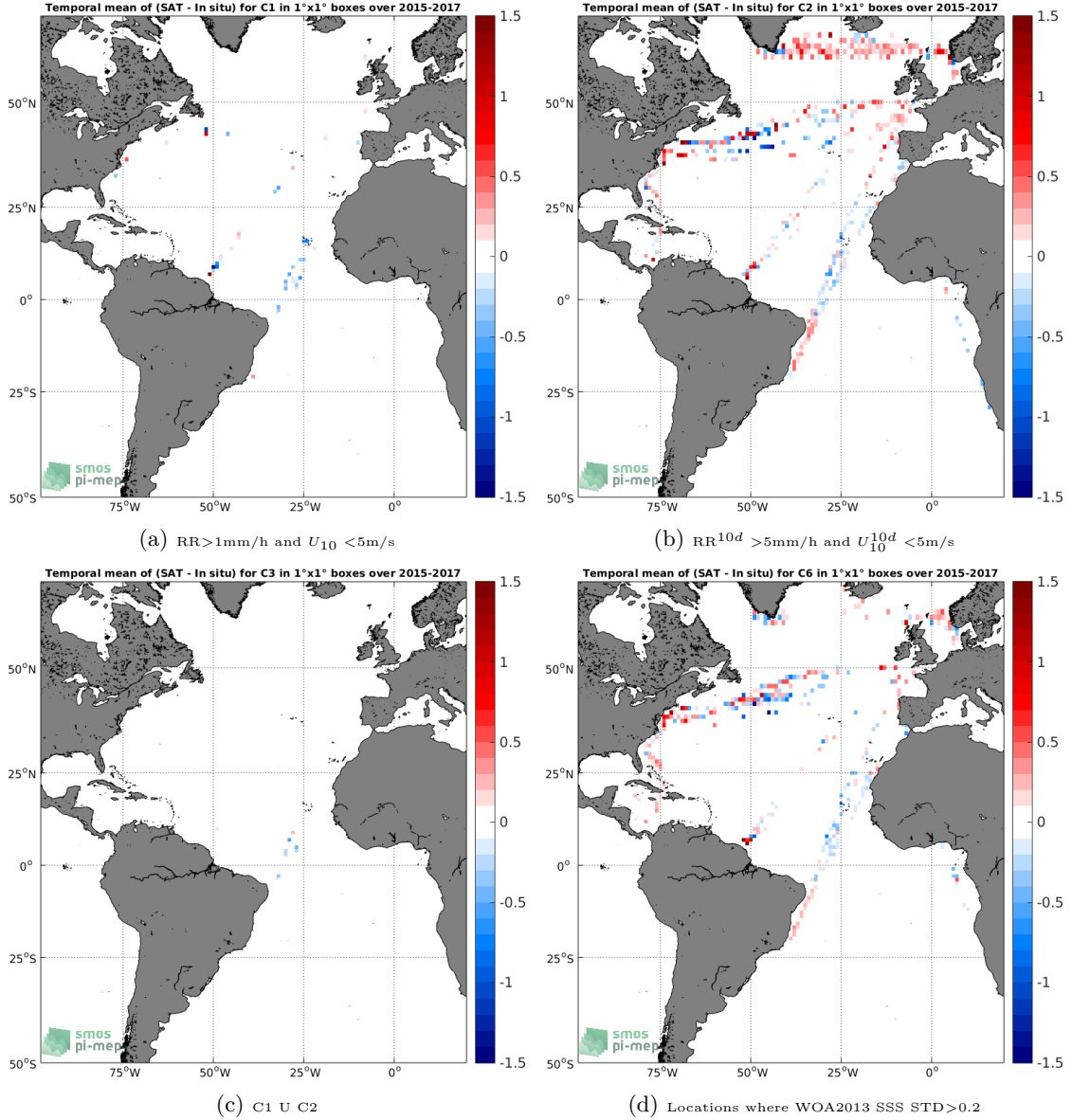
Figure 12: Temporal mean gridded over spatial boxes of size 1^\circ \times 1^\circ of \Delta SSS (SMAP-L3-RSS-V3-8DAY-RUNNING-70KM - TSG-LEGOS-DM) for 4 different subdatasets corresponding to: RR > 1\text{mm/h} and U_{10} < 5\text{m/s} (a), RR^{10d} > 5\text{mm/h} and U_{10}^{10d} < 5\text{m/s} (b), C1 U C2 (c), Locations where WOA2013 SSS STD > 0.2 (d).
