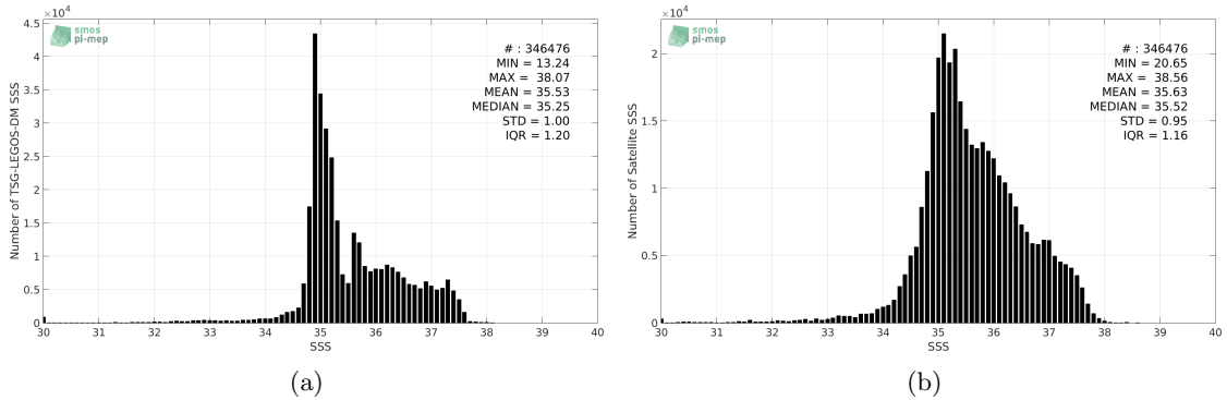
Figure 2: Histograms of SSS from TSG-LEGOS-DM (a) and SMAP-L3-RSS-V3-8DAY-RUNNING-70KM (b) considering all match-up pairs per bins of 0.1 over the Atlantic Ocean Pi-MEP region and for the full satellite product period.
