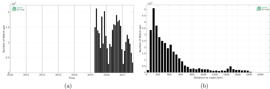
Figure 1: Number of match-ups between TSG-LEGOS-DM and SMAP-L3-RSS-V3-8DAY-RUNNING-70KM SSS as a function of time (a) and as function of the distance to coast (b) over the Atlantic Ocean Pi-MEP region and for the full satellite product period.
