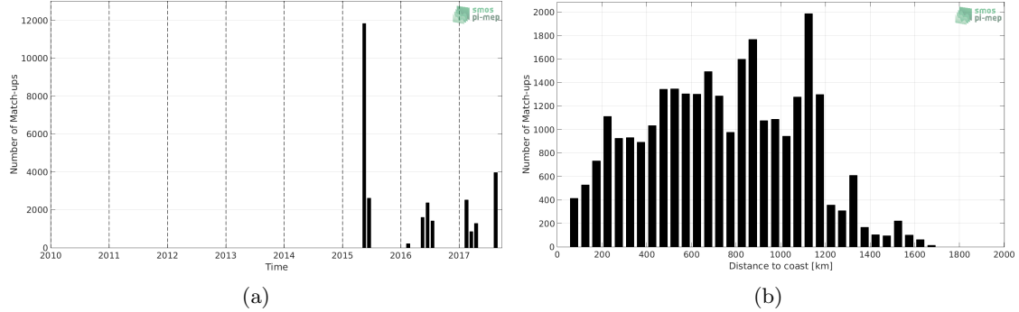
Figure 1: Number of match-ups between TSG-GOSUD-Sailing-ship and SMAP-L3-RSS-V3-8DAY-RUNNING-70KM SSS as a function of time (a) and as function of the distance to coast (b) over the Atlantic Ocean Pi-MEP region and for the full satellite product period.
