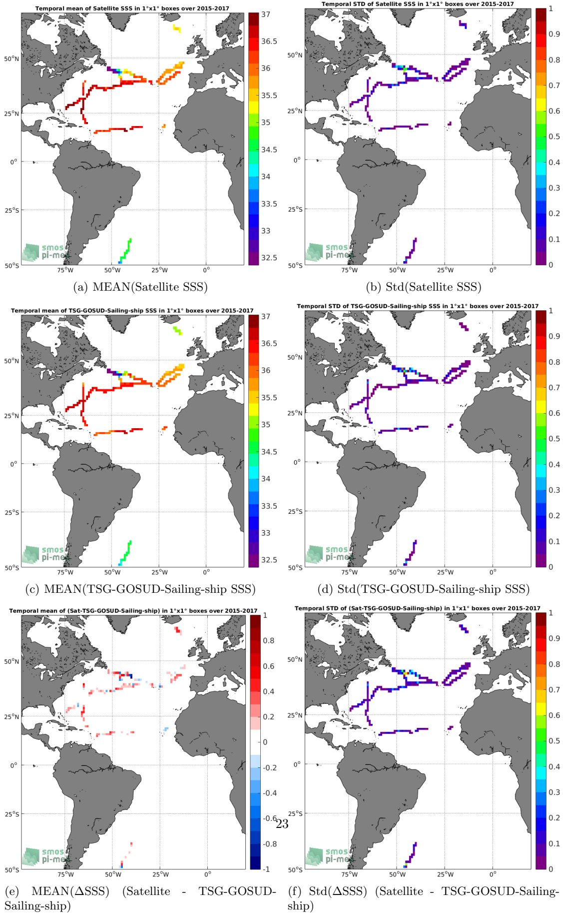
Figure 6: Temporal mean (left) and Std (right) of SSS from SMAP-L3-RSS-V3-8DAY-RUNNING-70KM (top), TSG-GOSUD-Sailing-ship (middle), and of \Delta SSS (Satellite - TSG-GOSUD-Sailing-ship). Only match-up pairs are used to generate these maps.
