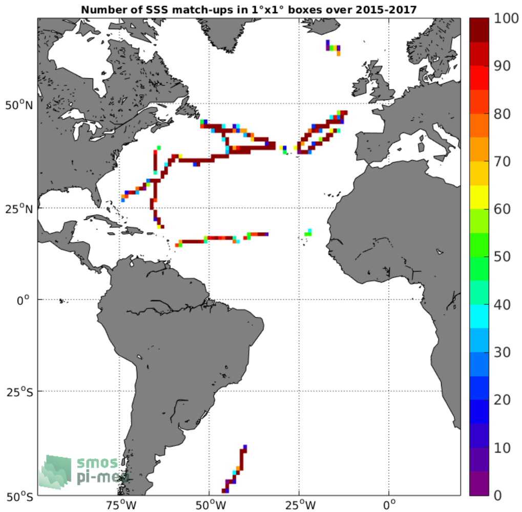
Figure 4: Number of SSS match-ups between TSG-GOSUD-Sailing-ship SSS and the SMAP-L3-RSS-V3-8DAY-RUNNING-70KM SSS product for the Atlantic Ocean Pi-MEP region over 1°x1° boxes and for the full satellite product period.
