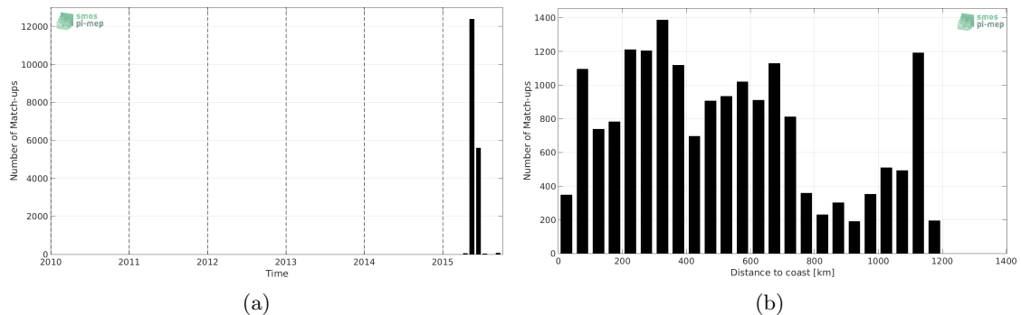
Figure 1: Number of match-ups between TSG-GOSUD-Sailing-ship and SMAP-L3-RSS-V3-8DAY-RUNNING-70KM SSS as a function of time (a) and as function of the distance to coast (b) over the Atlantic Ocean Pi-MEP region and for the full satellite product period.
