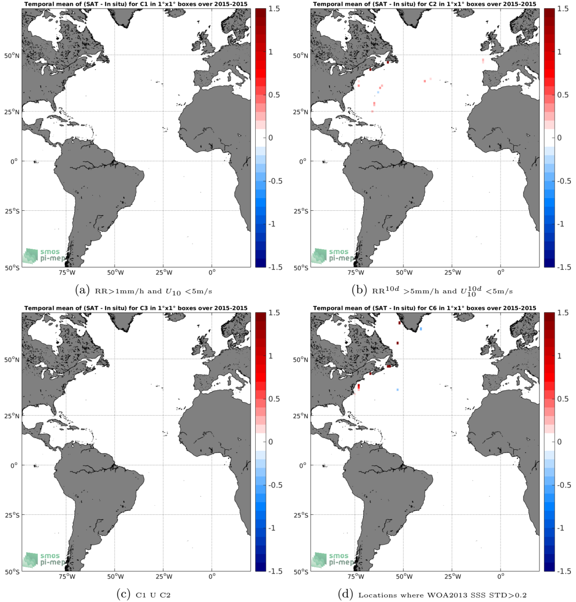
Figure 12: Temporal mean gridded over spatial boxes of size 1^\circ \times 1^\circ of \Delta SSS (SMAP-L3-RSS-V3-8DAY-RUNNING-70KM - TSG-GOSUD-Sailing-ship) for 4 different subdatasets corresponding to:RR>1mm/h and U_{10} < 5\text{m/s} (a), RR^{10d} > 5\text{mm/h} and U_{10}^{10d} < 5\text{m/s} (b), C1 U C2 (c),Locations where WOA2013 SSS STD>0.2 (d).
