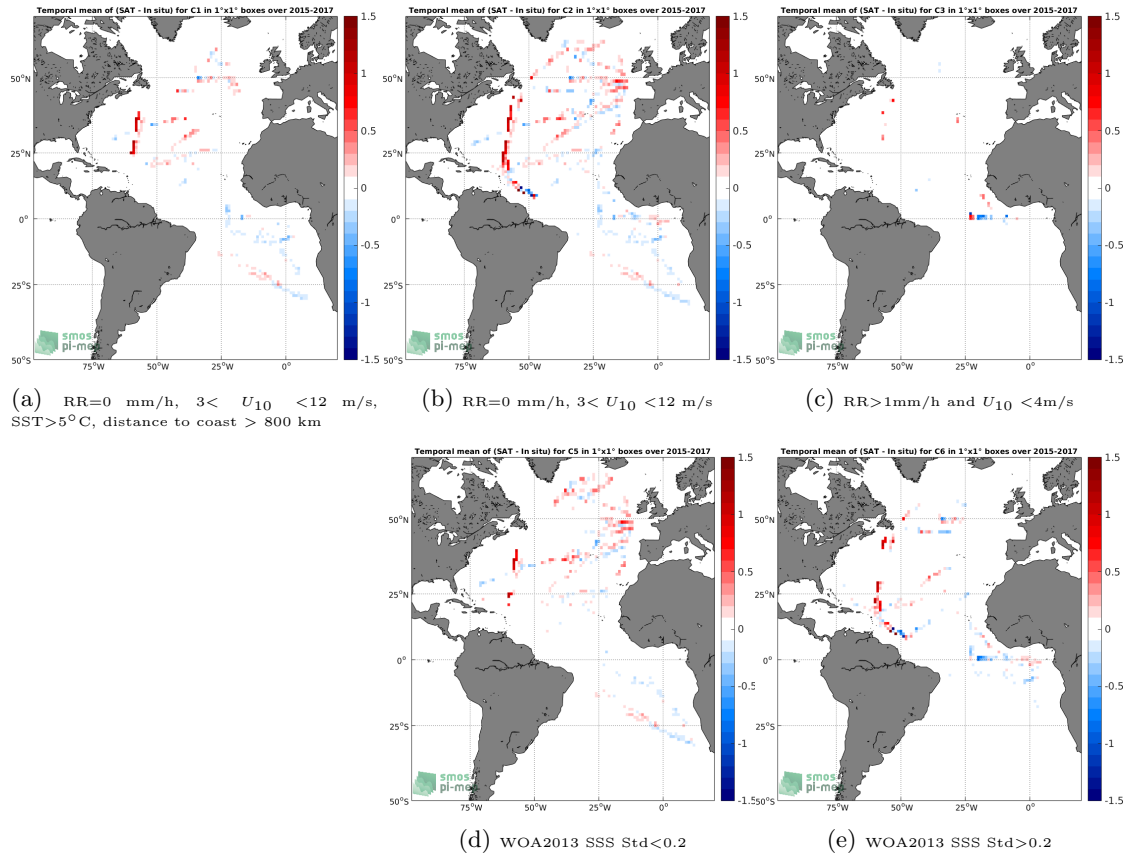
Figure 12: Temporal mean gridded over spatial boxes of size 1^\circ \times 1^\circ of \Delta SSS (SMAP-L3-RSS-V3-8DAY-RUNNING-70KM - TSG-GOSUD-Research-vessel) for 5 different subdatasets corresponding to:RR=0 mm/h, 3 < U_{10} < 12 m/s, SST >5^\circ C, distance to coast > 800 km (a), RR=0 mm/h, 3 < U_{10} < 12 m/s (b), RR >1 mm/h and U_{10} < 4 m/s (c), WOA2013 SSS Std <0.2 (d), WOA2013 SSS Std >0.2 (e).
