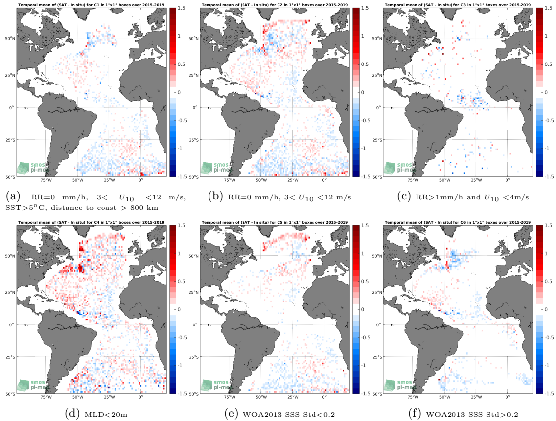
Figure 12: Temporal mean gridded over spatial boxes of size 1^\circ \times 1^\circ of \Delta SSS (SMAP-L3-RSS-V3-8DAY-RUNNING-70KM - Argo) for 6 different subdatasets corresponding to:RR=0 mm/h, 3 < U_{10} < 12 m/s, SST >5^\circ C, distance to coast > 800 km (a), RR=0 mm/h, 3 < U_{10} < 12 m/s (b), RR >1 mm/h and U_{10} < 4 m/s (c),MLD <20 m (d),WOA2013 SSS Std <0.2 (e),WOA2013 SSS Std >0.2 (f).
