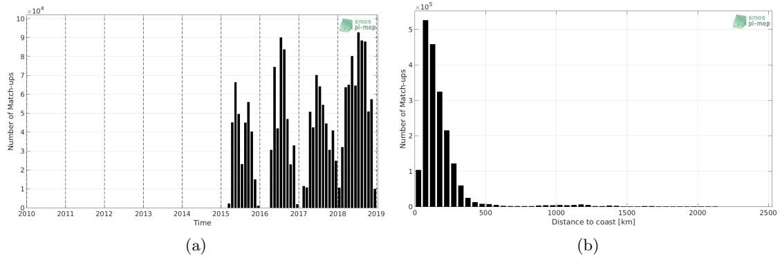
Figure 1: Number of match-ups between TSG-SAMOS and SMAP-L3-RSS-V3-8DAY-RUNNING-40KM SSS as a function of time (a) and as function of the distance to coast (b) over the Atlantic Ocean Pi-MEP region and for the full satellite product period.
