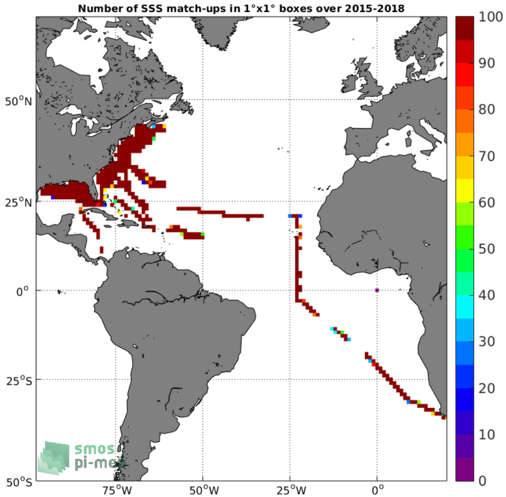
Figure 4: Number of SSS match-ups between TSG-SAMOS SSS and the SMAP-L3-RSS-V3-8DAY-RUNNING-40KM SSS product for the Atlantic Ocean Pi-MEP region over 1^{\circ} \times 1^{\circ} boxes and for the full satellite product period.
