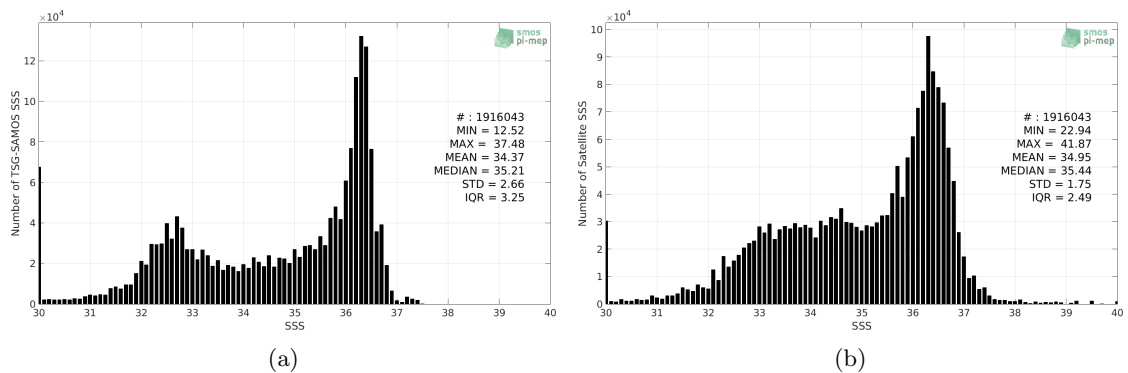
Figure 2: Histograms of SSS from TSG-SAMOS (a) and SMAP-L3-RSS-V3-8DAY-RUNNING-40KM (b) considering all match-up pairs per bins of 0.1 over the Atlantic Ocean Pi-MEP region and for the full satellite product period.
