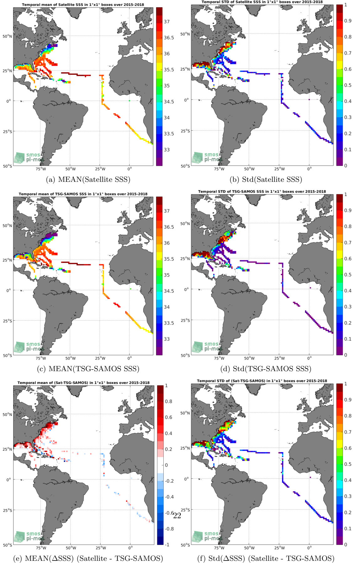
Figure 6: Temporal mean (left) and Std (right) of SSS from SMAP-L3-RSS-V3-8DAY-RUNNING-40KM (top), TSG-SAMOS (middle), and of \Delta SSS (Satellite - TSG-SAMOS). Only match-up pairs are used to generate these maps.
