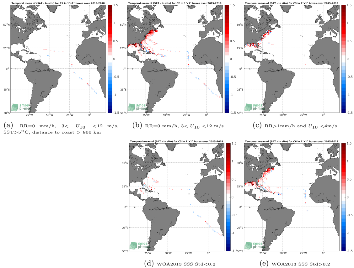
Figure 12: Temporal mean gridded over spatial boxes of size 1^\circ \times 1^\circ of \Delta SSS (SMAP-L3-RSS-V3-8DAY-RUNNING-40KM - TSG-SAMOS) for 5 different subdatasets corresponding to:RR=0 mm/h, 3 < U_{10} < 12 m/s, SST >5^\circ\text{C} , distance to coast > 800 km (a), RR=0 mm/h, 3 < U_{10} < 12 m/s (b), RR >1 mm/h and U_{10} < 4 m/s (c), WOA2013 SSS Std <0.2 (d), WOA2013 SSS Std >0.2 (e).
