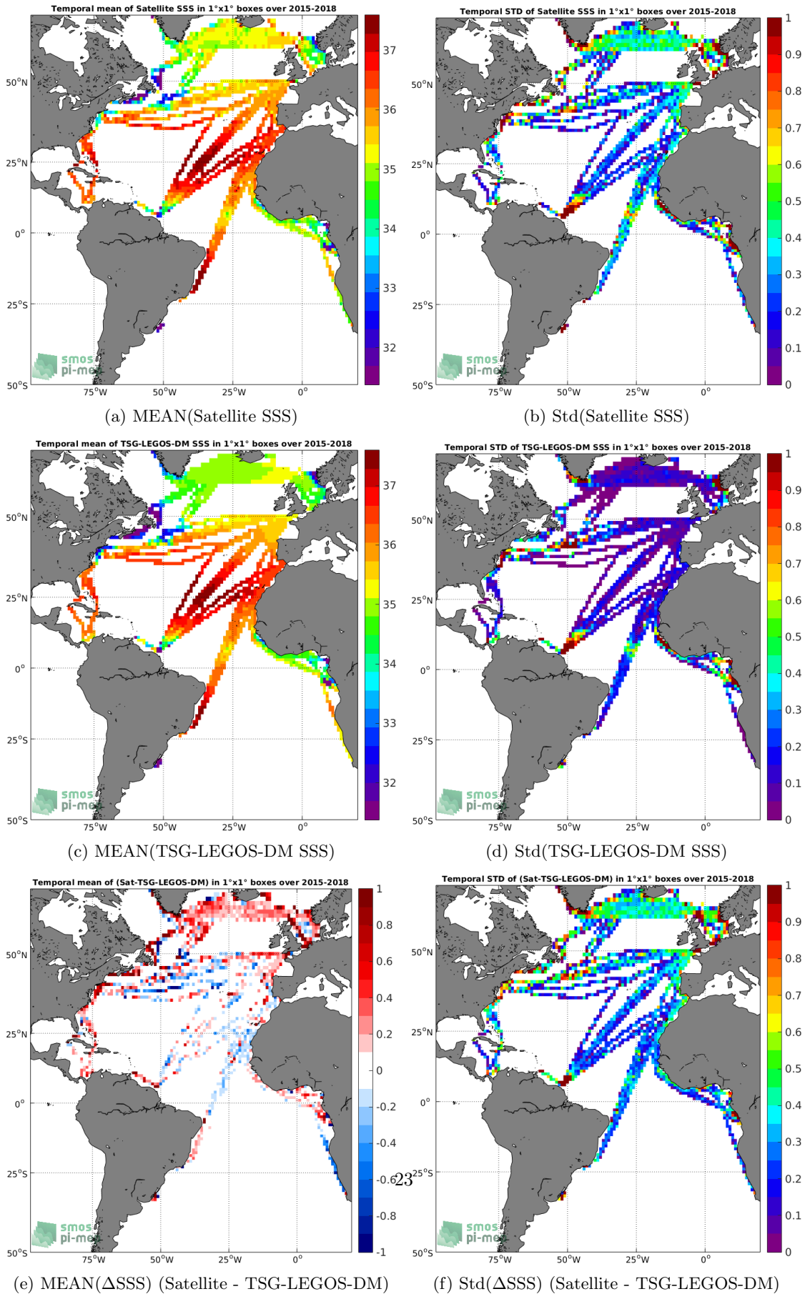
Figure 6: Temporal mean (left) and Std (right) of SSS from SMAP-L3-RSS-V3-8DAY-RUNNING-40KM (top), TSG-LEGOS-DM (middle), and of \Delta SSS (Satellite - TSG-LEGOS-DM). Only match-up pairs are used to generate these maps.
