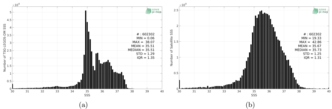
Figure 2: Histograms of SSS from TSG-LEGOS-DM (a) and SMAP-L3-RSS-V3-8DAY-RUNNING-40KM (b) considering all match-up pairs per bins of 0.1 over the Atlantic Ocean Pi-MEP region and for the full satellite product period.
