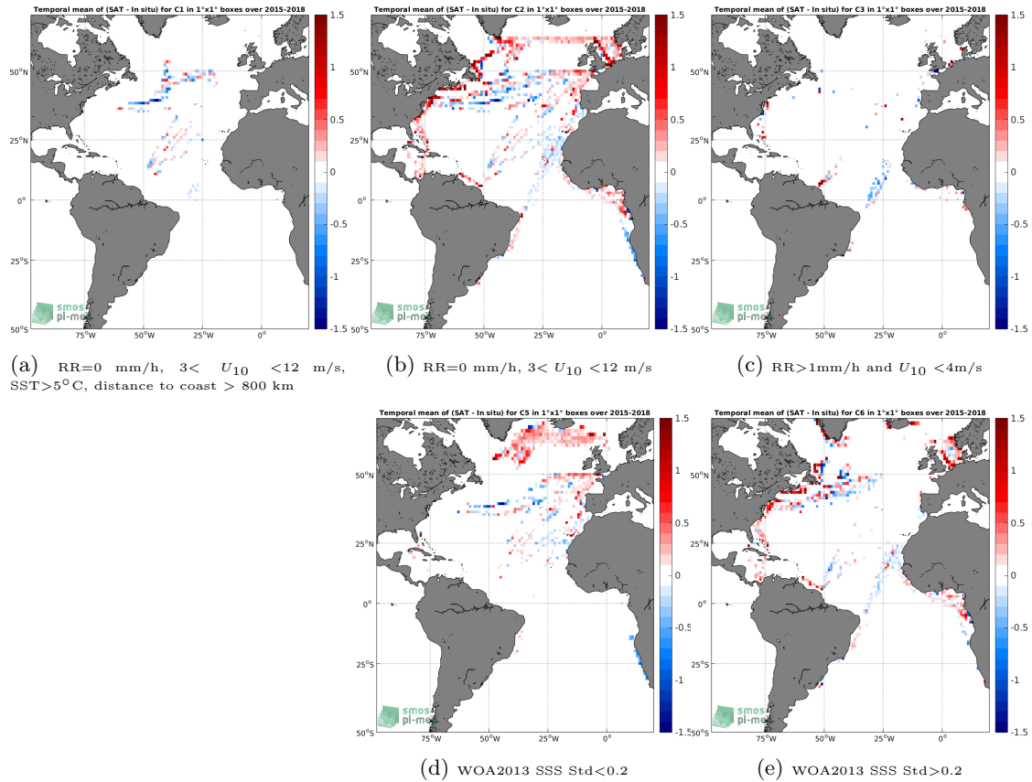
Figure 12: Temporal mean gridded over spatial boxes of size 1^\circ \times 1^\circ of \Delta SSS (SMAP-L3-RSS-V3-8DAY-RUNNING-40KM - TSG-LEGOS-DM) for 5 different subdatasets corresponding to:RR=0 mm/h, 3 < U_{10} < 12 m/s, SST >5^\circ\text{C} , distance to coast > 800 km (a), RR=0 mm/h, 3 < U_{10} < 12 m/s (b), RR >1 mm/h and U_{10} < 4 m/s (c), WOA2013 SSS Std <0.2 (d), WOA2013 SSS Std >0.2 (e).
