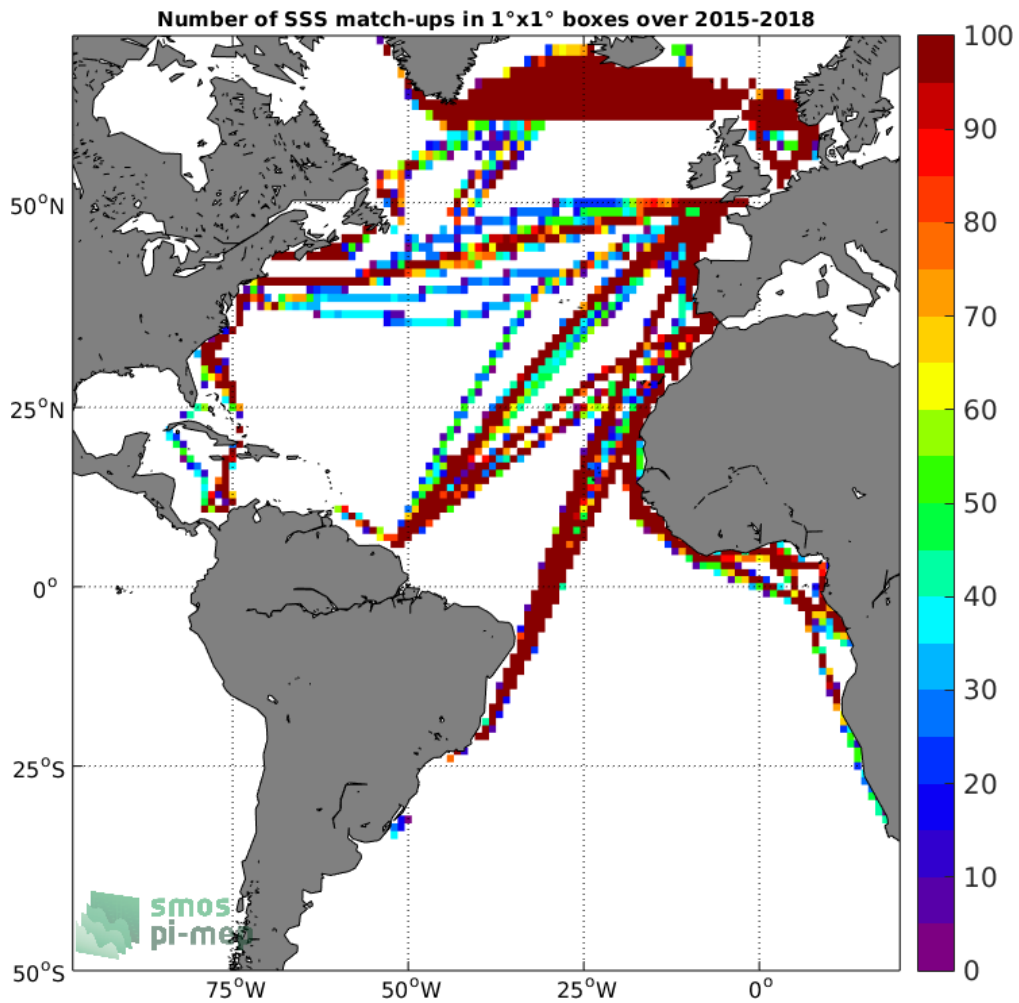
Figure 4: Number of SSS match-ups between TSG-LEGOS-DM SSS and the SMAP-L3-RSS-V3-8DAY-RUNNING-40KM SSS product for the Atlantic Ocean Pi-MEP region over 1°x1° boxes and for the full satellite product period.
