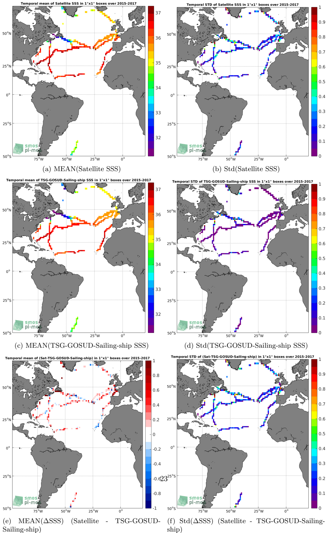
Figure 6: Temporal mean (left) and Std (right) of SSS from SMAP-L3-RSS-V3-8DAY-RUNNING-40KM (top), TSG-GOSUD-Sailing-ship (middle), and of \Delta SSS (Satellite - TSG-GOSUD-Sailing-ship). Only match-up pairs are used to generate these maps.
