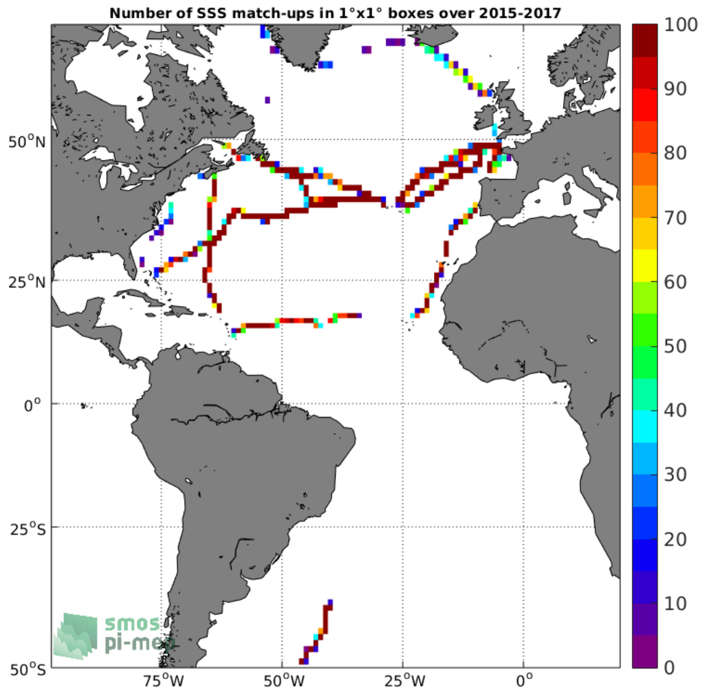
Figure 4: Number of SSS match-ups between TSG-GOSUD-Sailing-ship SSS and the SMAP-L3-RSS-V3-8DAY-RUNNING-40KM SSS product for the Atlantic Ocean Pi-MEP region over 1°x1° boxes and for the full satellite product period.
