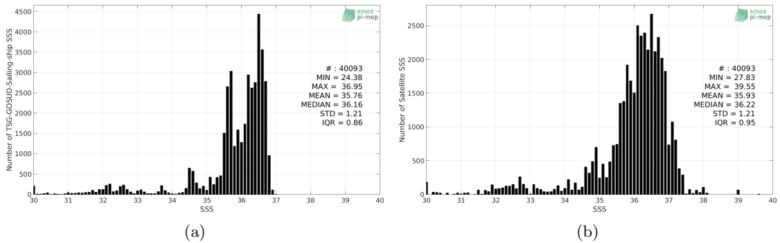
Figure 2: Histograms of SSS from TSG-GOSUD-Sailing-ship (a) and SMAP-L3-RSS-V3-8DAY-RUNNING-40KM (b) considering all match-up pairs per bins of 0.1 over the Atlantic Ocean Pi-MEP region and for the full satellite product period.
