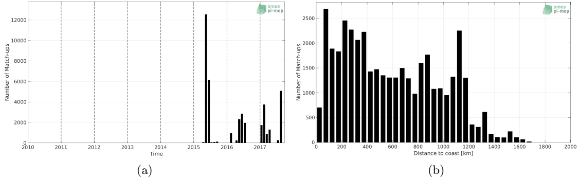
Figure 1: Number of match-ups between TSG-GOSUD-Sailing-ship and SMAP-L3-RSS-V3-8DAY-RUNNING-40KM SSS as a function of time (a) and as function of the distance to coast (b) over the Atlantic Ocean Pi-MEP region and for the full satellite product period.
