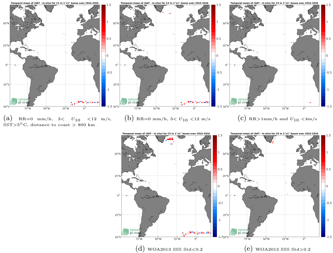
Figure 11: Temporal mean gridded over spatial boxes of size 1^\circ \times 1^\circ of \Delta SSS (SMAP-L3-RSS-V3-8DAY-RUNNING-40KM - Surface drifters) for 5 different subdatasets corresponding to:RR=0 mm/h, 3 < U_{10} < 12 m/s, SST >5^\circ\text{C} , distance to coast > 800 km (a), RR=0 mm/h, 3 < U_{10} < 12 m/s (b), RR >1 mm/h and U_{10} < 4 m/s (c), WOA2013 SSS Std <0.2 (d), WOA2013 SSS Std >0.2 (e).
