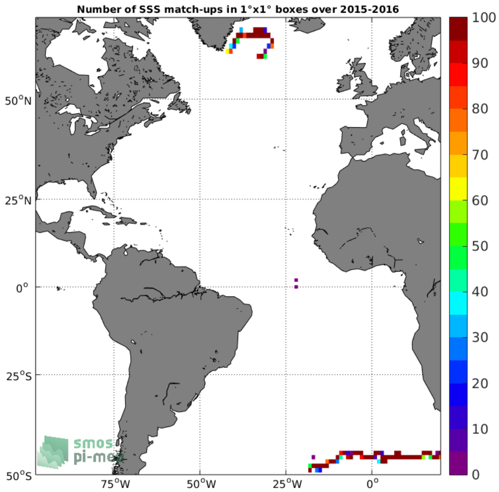
Figure 3: Number of SSS match-ups between Surface drifters SSS and the SMAP-L3-RSS-V3-8DAY-RUNNING-40KM SSS product for the Atlantic Ocean Pi-MEP region over 1°x1° boxes and for the full satellite product period.
