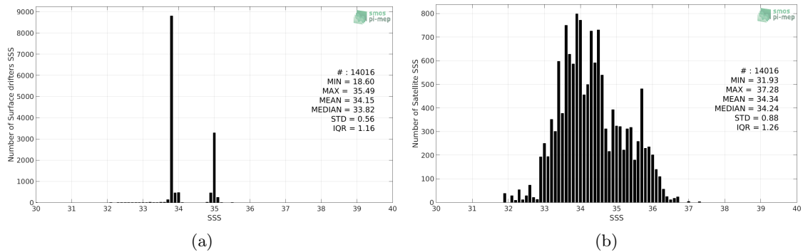
Figure 2: Histograms of SSS from Surface drifters (a) and SMAP-L3-RSS-V3-8DAY-RUNNING-40KM (b) considering all match-up pairs per bins of 0.1 over the Atlantic Ocean Pi-MEP region and for the full satellite product period.
