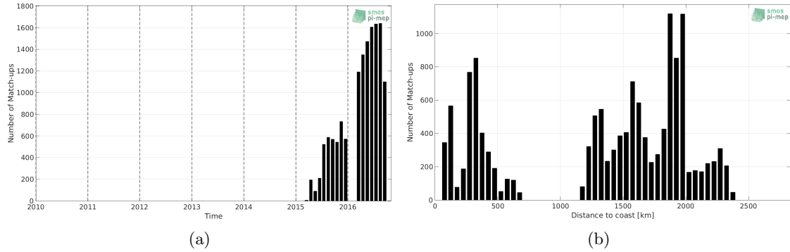
Figure 1: Number of match-ups between Surface drifters and SMAP-L3-RSS-V3-8DAY-RUNNING-40KM SSS as a function of time (a) and as function of the distance to coast (b) over the Atlantic Ocean Pi-MEP region and for the full satellite product period.
