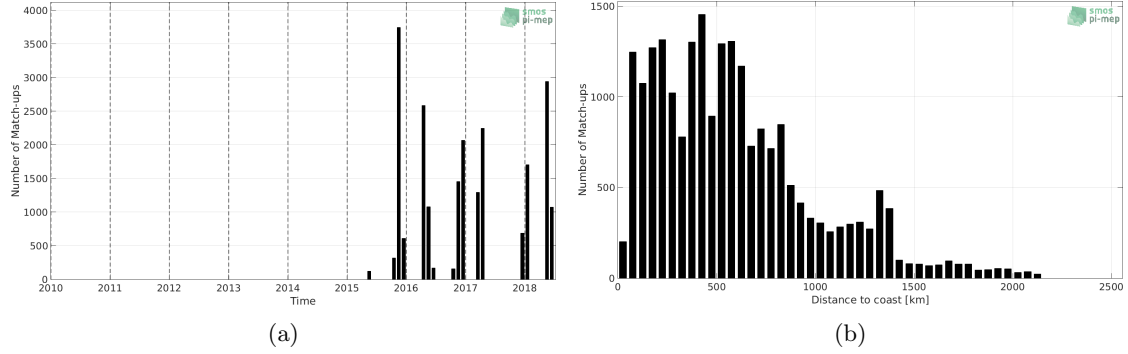
Figure 1: Number of match-ups between TSG-POLARSTERN and SMAP-L3-RSS-V3-MONTHLY-0.25DEG-40KM SSS as a function of time (a) and as function of the distance to coast (b) over the Atlantic Ocean Pi-MEP region and for the full satellite product period.
