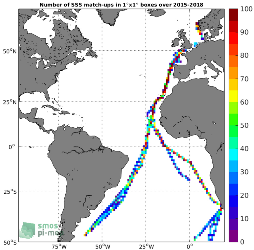
Figure 4: Number of SSS match-ups between TSG-POLARSTERN SSS and the SMAP-L3-RSS-V3-MONTHLY-0.25DEG-40KM SSS product for the Atlantic Ocean Pi-MEP region over 1°x1° boxes and for the full satellite product period.
