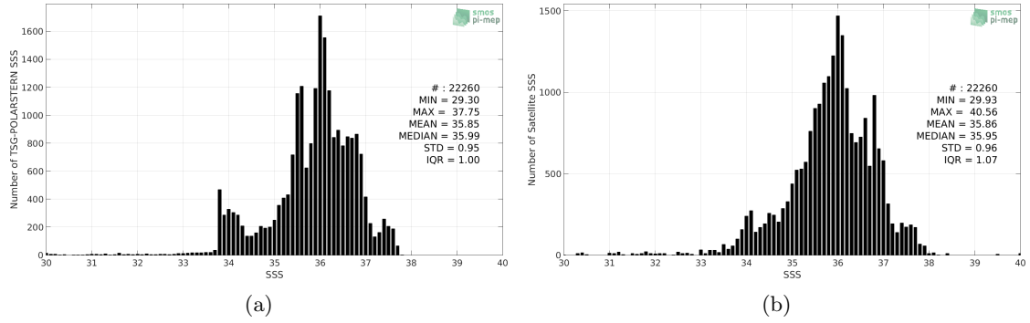
Figure 2: Histograms of SSS from TSG-POLARSTERN (a) and SMAP-L3-RSS-V3-MONTHLY-0.25DEG-40KM (b) considering all match-up pairs per bins of 0.1 over the Atlantic Ocean Pi-MEP region and for the full satellite product period.
