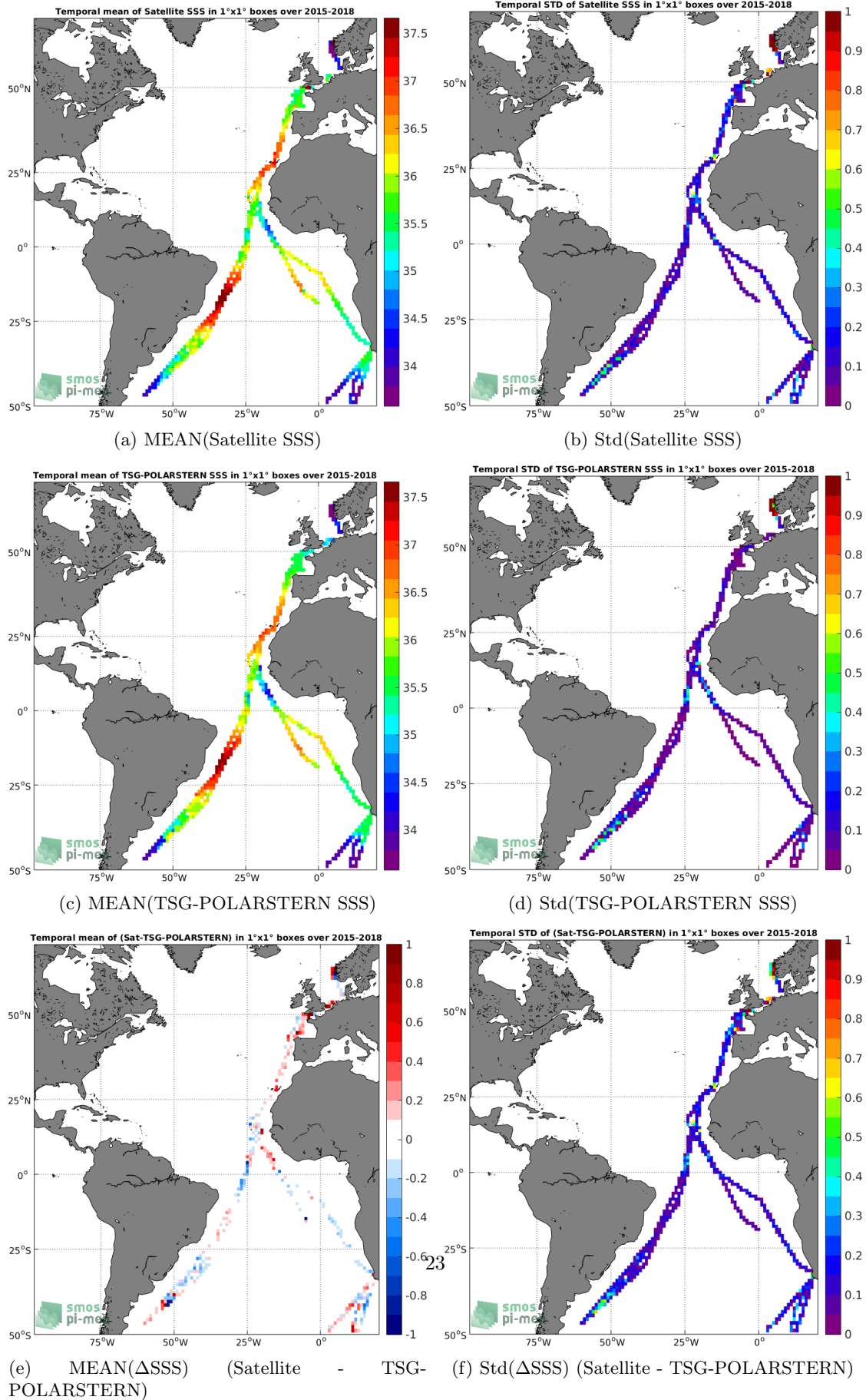
Figure 6: Temporal mean (left) and Std (right) of SSS from SMAP-L3-RSS-V3-MONTHLY-0.25DEG-40KM (top), TSG-POLARSTERN (middle), and of \Delta SSS (Satellite - TSG-POLARSTERN). Only match-up pairs are used to generate these maps.
