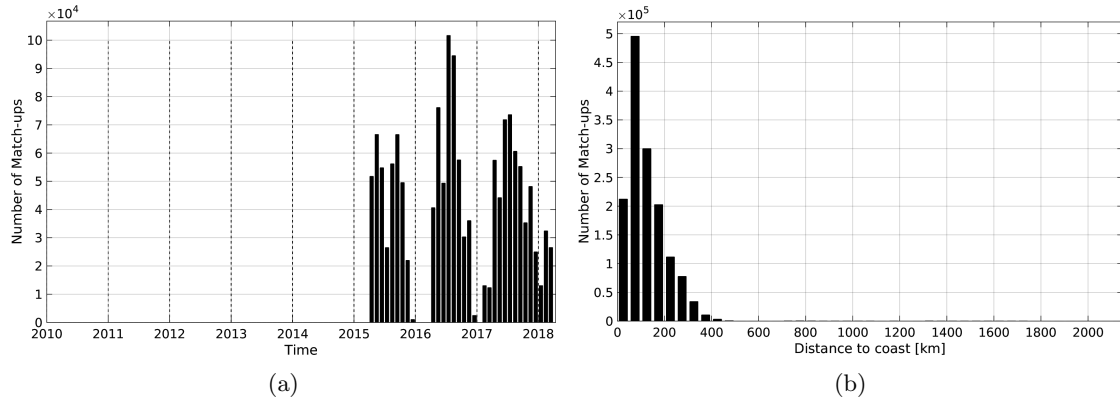
Figure 1: Number of match-ups between TSG-SAMOS and SMAP-L3-RSS-V2-MONTHLY-0.25DEG-40KM SSS as a function of time (a) and as function of the distance to coast (b) over the Atlantic Ocean Pi-MEP region and for the full satellite product period.
