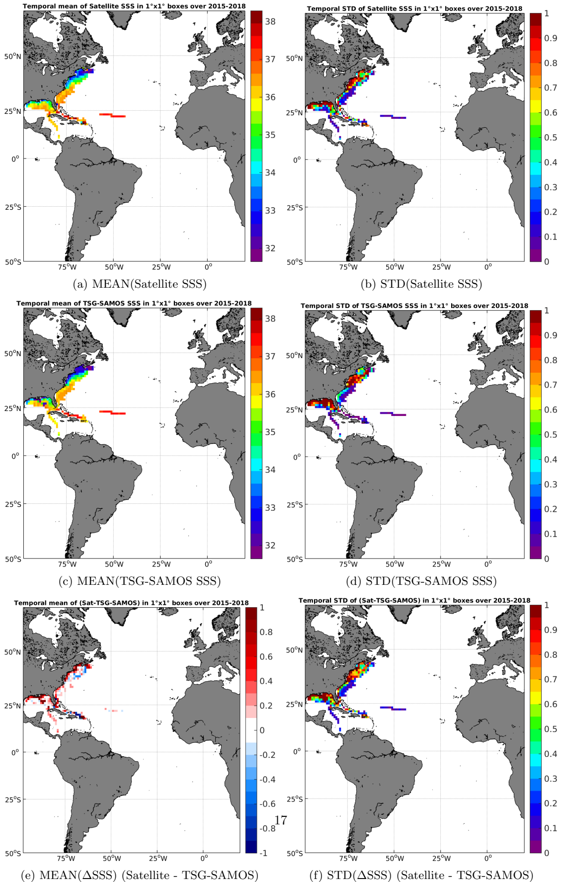
Figure 6: Temporal mean (left) and STD (right) of SSS from SMAP-L3-RSS-V2-MONTHLY-0.25DEG-40KM (top), TSG-SAMOS (middle), and of \Delta SSS (Satellite - TSG-SAMOS). Only match-up pairs are used to generate these maps.
