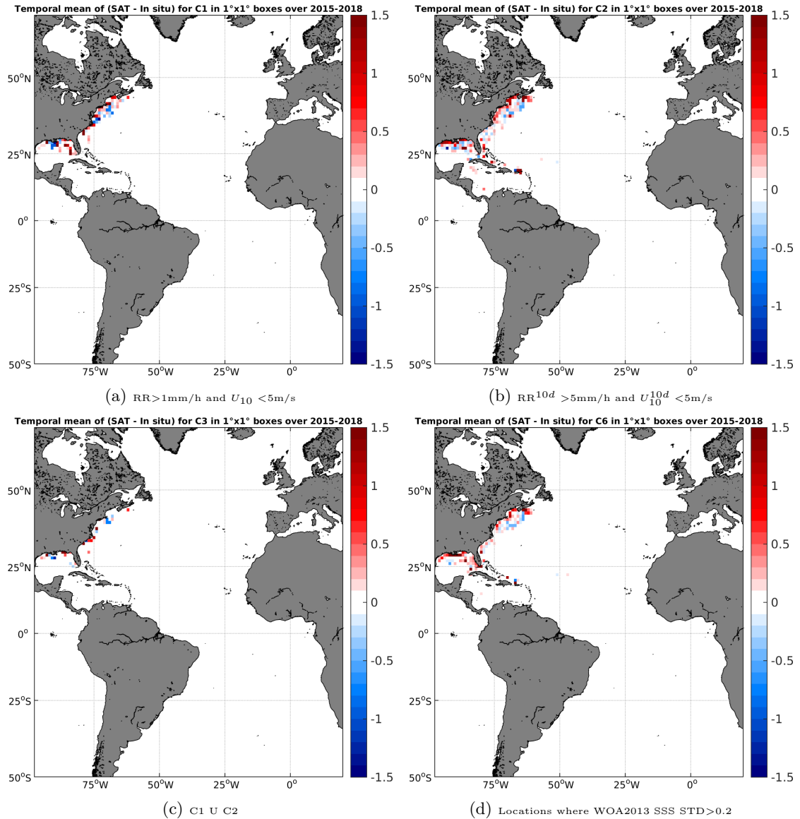
Figure 12: Temporal mean gridded over spatial boxes of size 1^\circ \times 1^\circ of \Delta SSS (SMAP-L3-RSS-V2-MONTHLY-0.25DEG-40KM - TSG-SAMOS) for 4 different subdatasets corresponding to: RR > 1 mm/h and U_{10} < 5 m/s (a), RR 10d > 5 mm/h and U_{10}^{10d} < 5 m/s (b), C1 U C2 (c), Locations where WOA2013 SSS STD > 0.2 (d).
