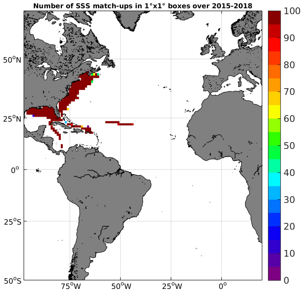
Figure 4: Number of SSS match-ups between TSG-SAMOS SSS and the SMAP-L3-RSS-V2-MONTHLY-0.25DEG-40KM SSS product for the Atlantic Ocean Pi-MEP region over 1°x1° boxes and for the full satellite product period.
