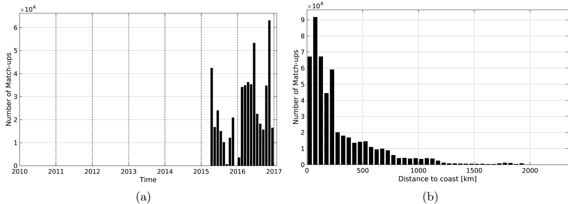
Figure 1: Number of match-ups between TSG-GOSUD-Research-vessel and SMAP-L3-RSS-V2-MONTHLY-0.25DEG-40KM SSS as a function of time (a) and as function of the distance to coast (b) over the Atlantic Ocean Pi-MEP region and for the full satellite product period.
