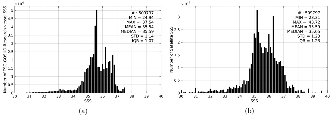
Figure 2: Histograms of SSS from TSG-GOSUD-Research-vessel (a) and SMAP-L3-RSS-V2-MONTHLY-0.25DEG-40KM (b) considering all match-up pairs per bins of 0.1 over the Atlantic Ocean Pi-MEP region and for the full satellite product period.
