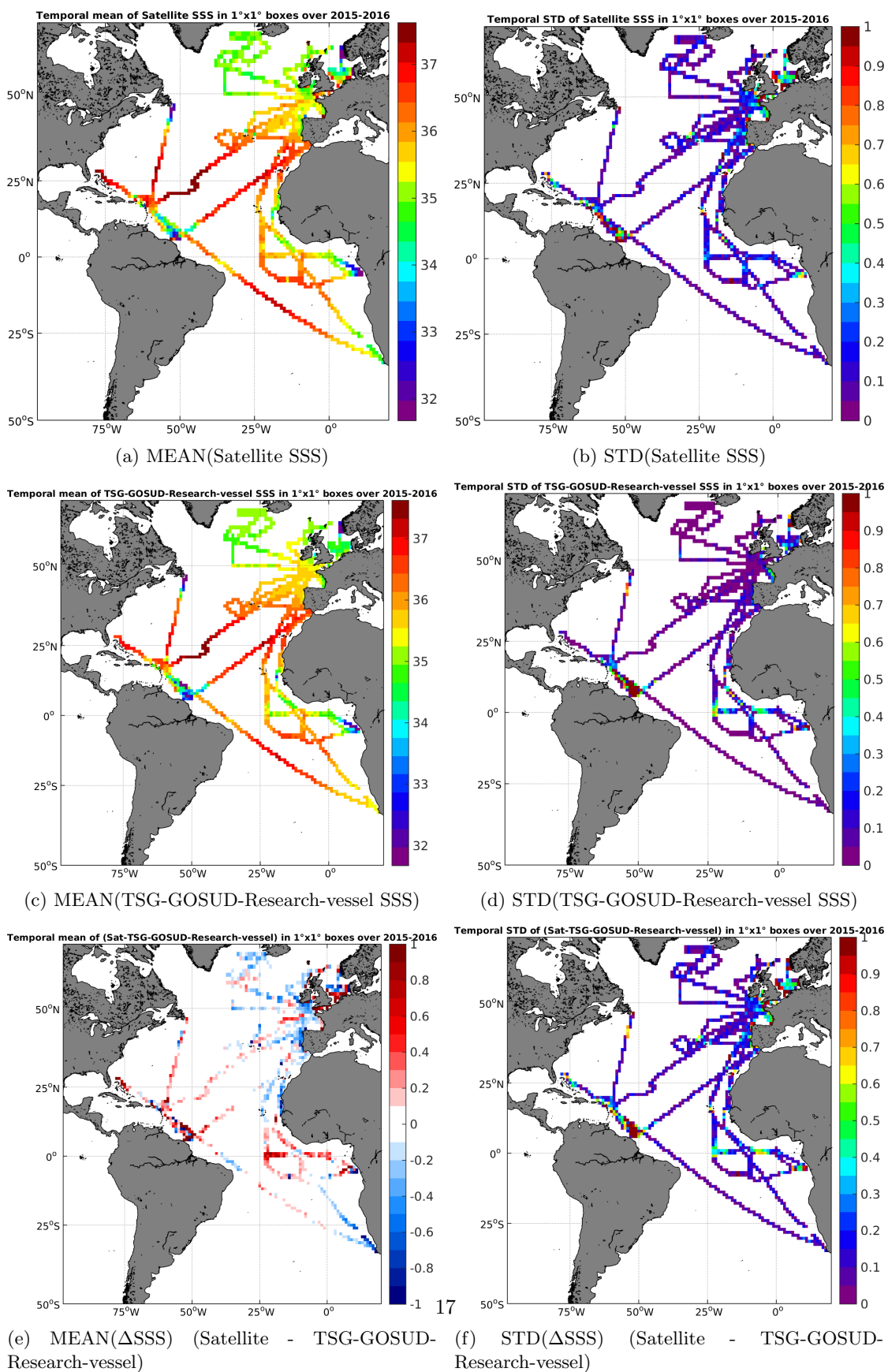
Figure 6: Temporal mean (left) and STD (right) of SSS from SMAP-L3-RSS-V2-MONTHLY-0.25DEG-40KM (top), TSG-GOSUD-Research-vessel (middle), and of \Delta SSS (Satellite - TSG-GOSUD-Research-vessel). Only match-up pairs are used to generate these maps.
