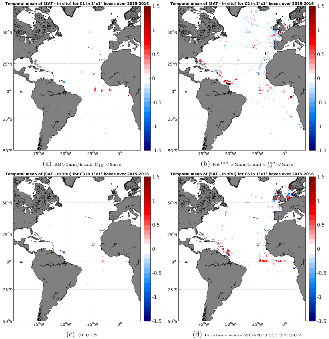
Figure 12: Temporal mean gridded over spatial boxes of size 1^\circ \times 1^\circ of \Delta\text{SSS} (SMAP-L3-RSS-V2-MONTHLY-0.25DEG-40KM - TSG-GOSUD-Research-vessel) for 4 different subdatasets corresponding to: RR > 1\text{mm/h} and U_{10} < 5\text{m/s} (a), RR^{10d} > 5\text{mm/h} and U_{10}^{10d} < 5\text{m/s} (b), C1 U C2 (c), Locations where WOA2013 SSS STD > 0.2 (d).
