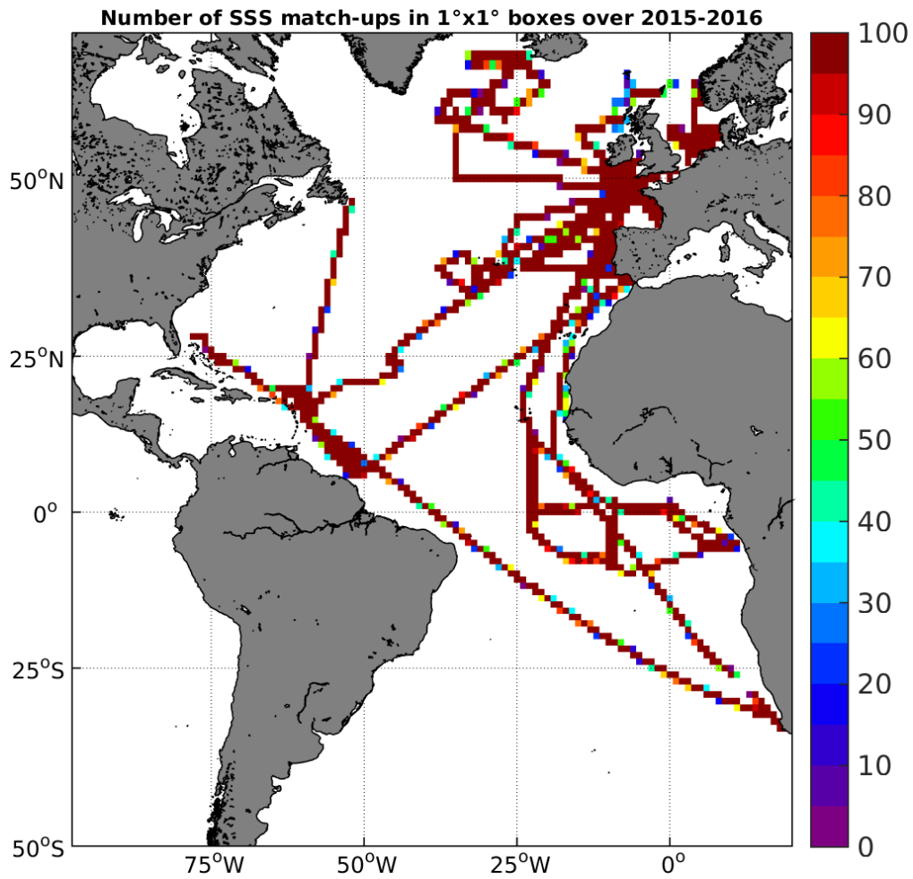
Figure 4: Number of SSS match-ups between TSG-GOSUD-Research-vessel SSS and the SMAP-L3-RSS-V2-MONTHLY-0.25DEG-40KM SSS product for the Atlantic Ocean Pi-MEP region over 1°x1° boxes and for the full satellite product period.
