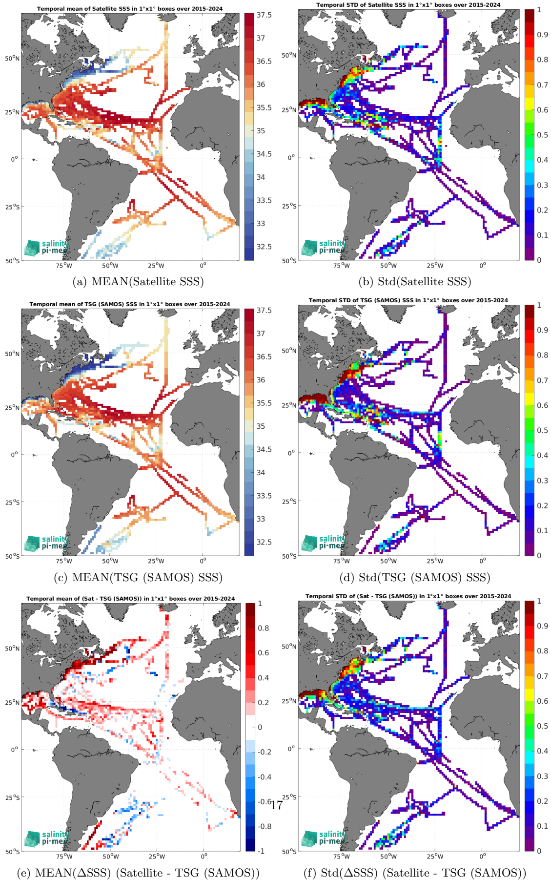
Figure 7: Temporal mean (left) and Std (right) of SSS from SMAP SSS L3 v5.0 - 8-Day running (JPL) (top), TSG (SAMOS) (middle), and of \Delta SSS (Satellite - TSG (SAMOS)). Only match-up pairs are used to generate these maps.
