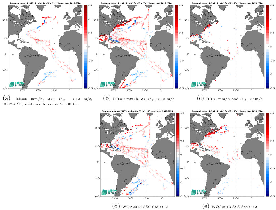
Figure 14: Temporal mean gridded over spatial boxes of size 1^\circ \times 1^\circ of \Delta SSS (SMAP SSS L3 v5.0 - 8-Day running (JPL) - TSG (SAMOS)) for 5 different subdatasets corresponding to:RR=0 mm/h, 3 < U_{10} < 12 m/s, SST>5°C, distance to coast > 800 km (a), RR=0 mm/h, 3 < U_{10} < 12 m/s (b), RR>1mm/h and U_{10} < 4 m/s (c), WOA2013 SSS Std<0.2 (d), WOA2013 SSS Std>0.2 (e).
