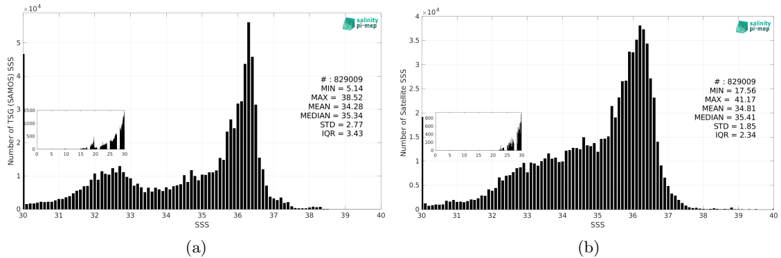
Figure 3: Histograms of SSS from TSG (SAMOS) (a) and SMAP SSS L3 v5.0 - 8-Day running (JPL) (b) considering all match-up pairs per bins of 0.1 over the Atlantic Ocean Pi-MEP region and for the full satellite product period.
