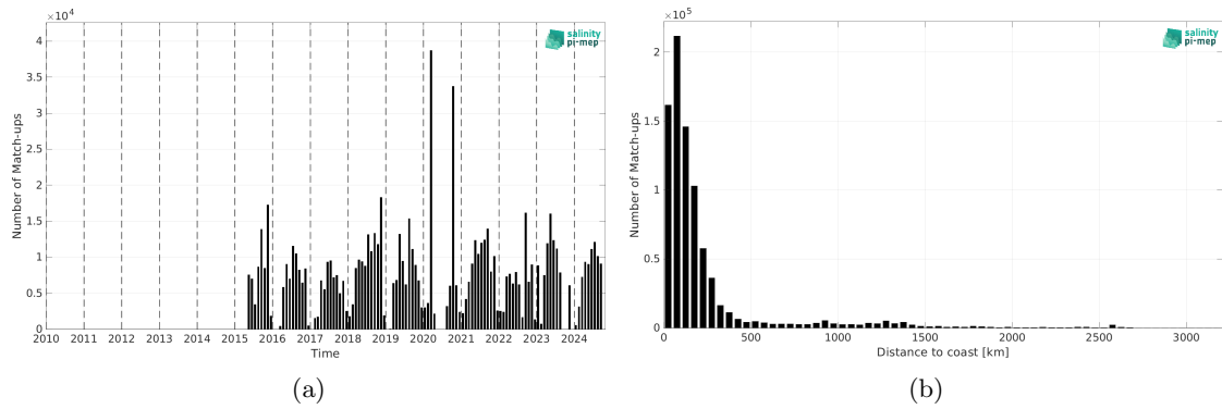
Figure 2: Number of match-ups between TSG (SAMOS) and SMAP SSS L3 v5.0 - 8-Day running (JPL) SSS as a function of time (a) and as function of the distance to coast (b) over the Atlantic Ocean Pi-MEP region and for the full satellite product period.
