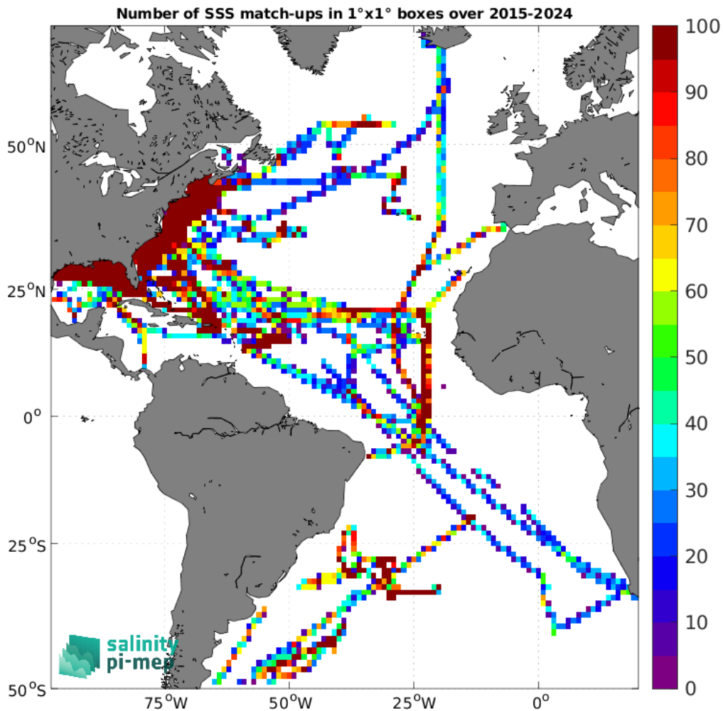
Figure 5: Number of SSS match-ups between TSG (SAMOS) SSS and the SMAP SSS L3 v5.0 - 8-Day running (JPL) SSS product for the Atlantic Ocean Pi-MEP region over 1^\circ \times 1^\circ boxes and for the full satellite product period.
