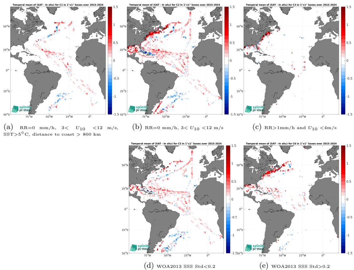
Figure 14: Temporal mean gridded over spatial boxes of size 1^\circ \times 1^\circ of \Delta\text{SSS} (SMAP SSS L3 v5.0 - 8-Day running (JPL) - TSG (SAMOS)) for 5 different subdatasets corresponding to:RR=0 mm/h, 3 < U_{10} < 12 m/s, SST>5°C, distance to coast > 800 km (a), RR=0 mm/h, 3 < U_{10} < 12 m/s (b), RR>1mm/h and U_{10} < 4 m/s (c), WOA2013 SSS Std<0.2 (d), WOA2013 SSS Std>0.2 (e).
