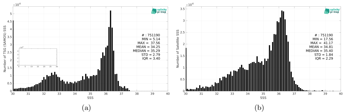
Figure 2: Histograms of SSS from TSG (SAMOS) (a) and SMAP SSS L3 v5.0 - 8-Day running (JPL) (b) considering all match-up pairs per bins of 0.1 over the Atlantic Ocean Pi-MEP region and for the full satellite product period.
