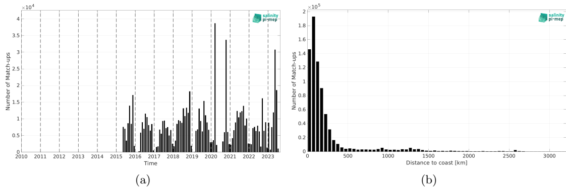
Figure 1: Number of match-ups between TSG (SAMOS) and SMAP SSS L3 v5.0 - 8-Day running (JPL) SSS as a function of time (a) and as function of the distance to coast (b) over the Atlantic Ocean Pi-MEP region and for the full satellite product period.
