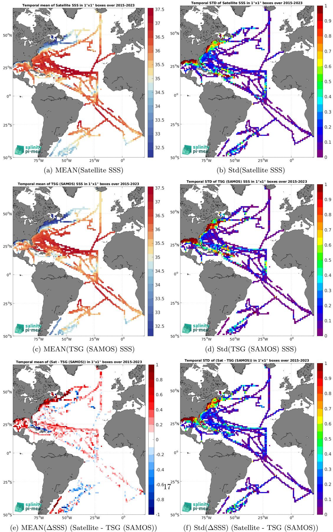
Figure 6: Temporal mean (left) and Std (right) of SSS from SMAP SSS L3 v5.0 - 8-Day running (JPL) (top), TSG (SAMOS) (middle), and of \Delta SSS (Satellite - TSG (SAMOS)). Only match-up pairs are used to generate these maps.
