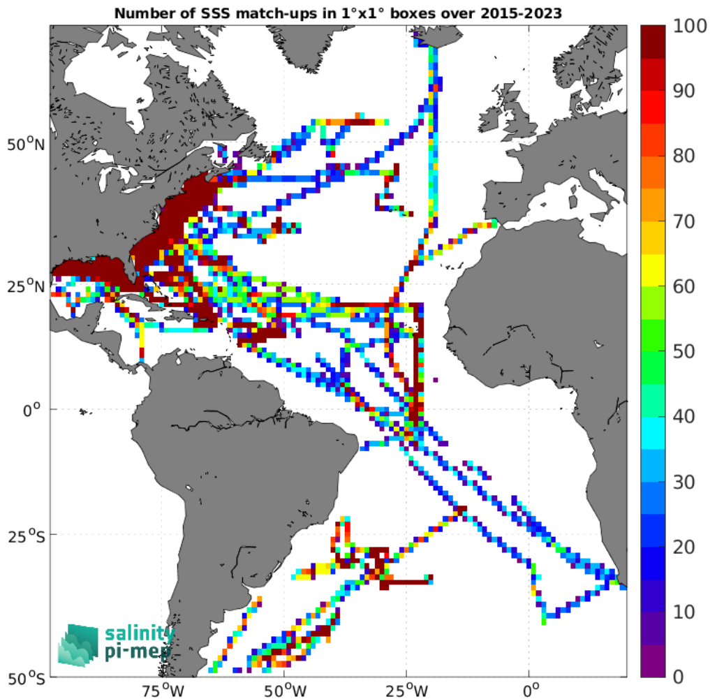
Figure 4: Number of SSS match-ups between TSG (SAMOS) SSS and the SMAP SSS L3 v5.0 - 8-Day running (JPL) SSS product for the Atlantic Ocean Pi-MEP region over 1^\circ \times 1^\circ boxes and for the full satellite product period.
