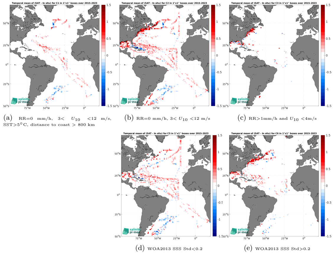
Figure 12: Temporal mean gridded over spatial boxes of size 1^\circ \times 1^\circ of \Delta SSS (SMAP SSS L3 v5.0 - 8-Day running (JPL) - TSG (SAMOS)) for 5 different subdatasets corresponding to:RR=0 mm/h, 3 < U_{10} < 12 m/s, SST >5^\circ\text{C} , distance to coast > 800 km (a), RR=0 mm/h, 3 < U_{10} < 12 m/s (b), RR >1 mm/h and U_{10} < 4 m/s (c), WOA2013 SSS Std <0.2 (d), WOA2013 SSS Std >0.2 (e).
