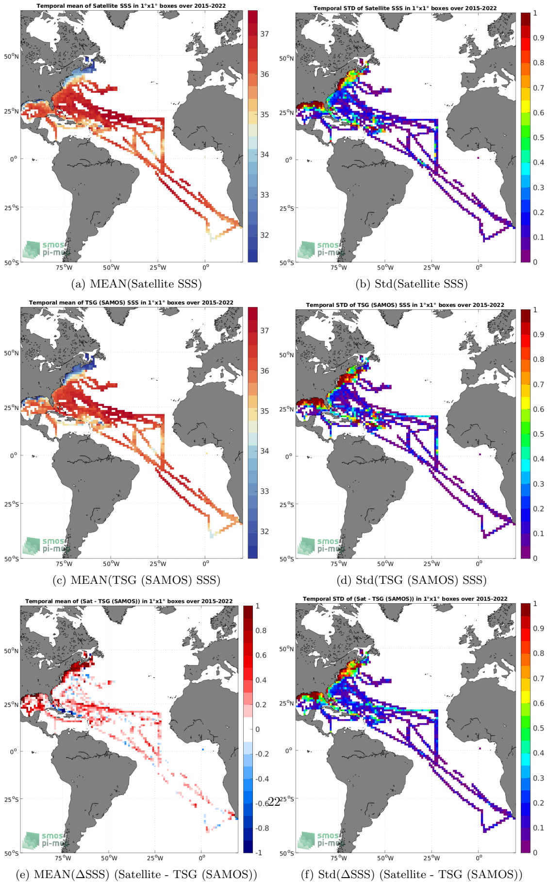
Figure 6: Temporal mean (left) and Std (right) of SSS from SMAP SSS L3 v5.0 - 8-Day running (JPL) (top), TSG (SAMOS) (middle), and of \Delta SSS (Satellite - TSG (SAMOS)). Only match-up pairs are used to generate these maps.
