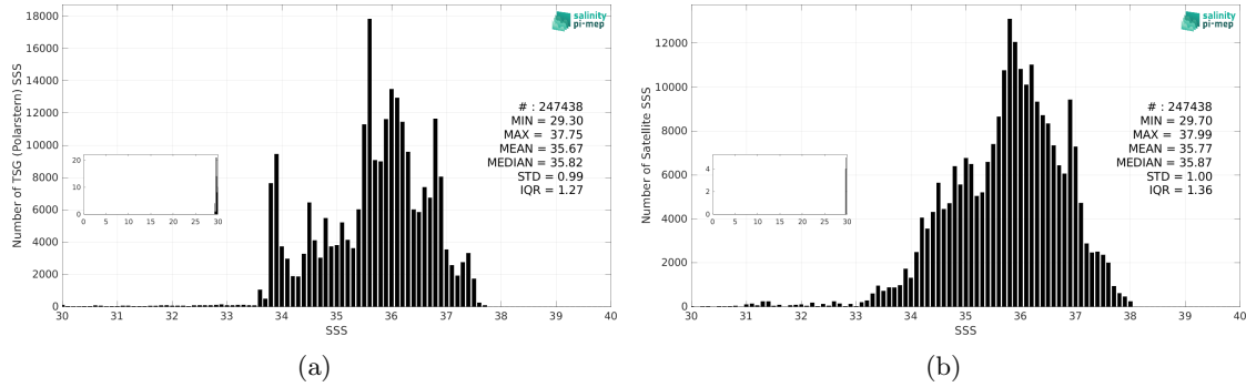
Figure 3: Histograms of SSS from TSG (Polarstern) (a) and SMAP SSS L3 v5.0 - 8-Day running (JPL) (b) considering all match-up pairs per bins of 0.1 over the Atlantic Ocean Pi-MEP region and for the full satellite product period.
