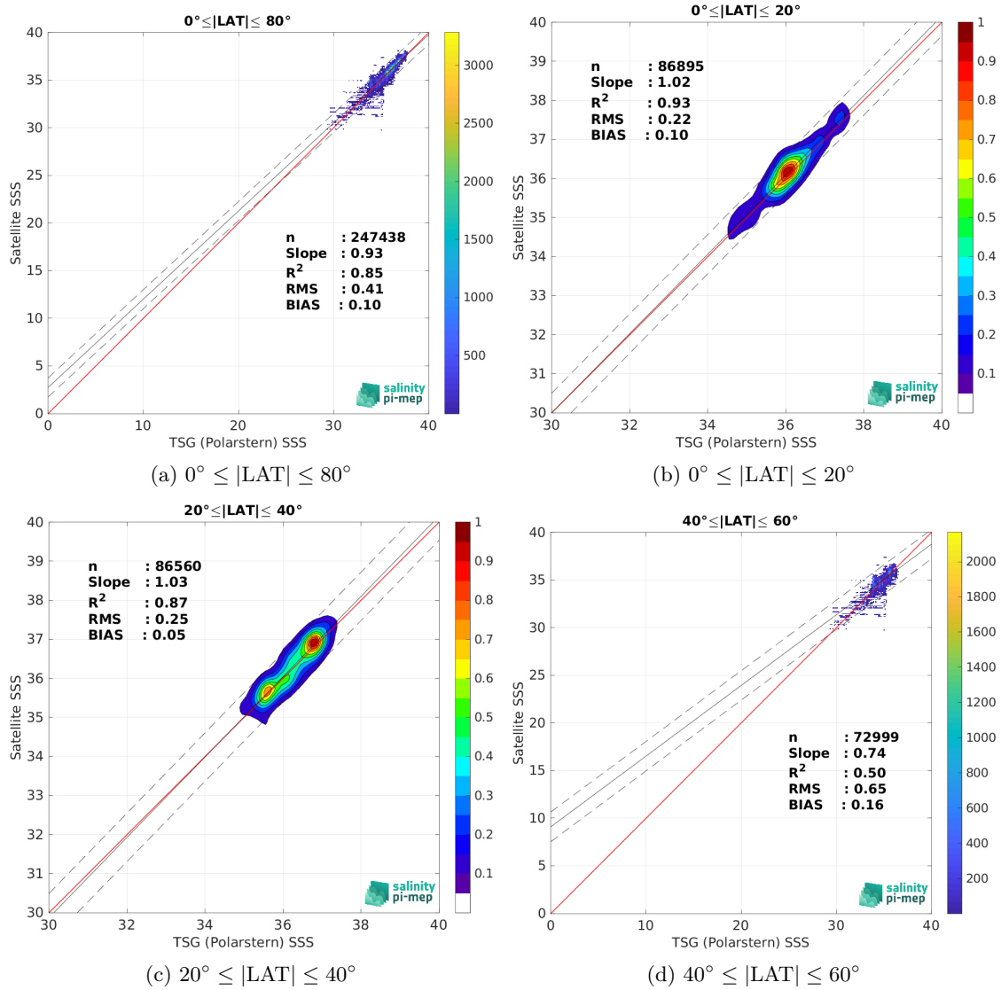
Figure 10: Contour maps of the concentration of SMAP SSS L3 v5.0 - 8-Day running (JPL) SSS (y-axis) versus TSG (Polarstern) SSS (x-axis) at match-up pairs for different latitude bands. For each plot, the red line shows x=y . The black thin and dashed lines indicate a linear fit through the data cloud and the \pm 95\% confidence levels, respectively. The number match-up pairs n , the slope and R^2 coefficient of the linear fit, the root mean square (RMS) and the mean bias between satellite and in situ data are indicated for each latitude band in each plots.
