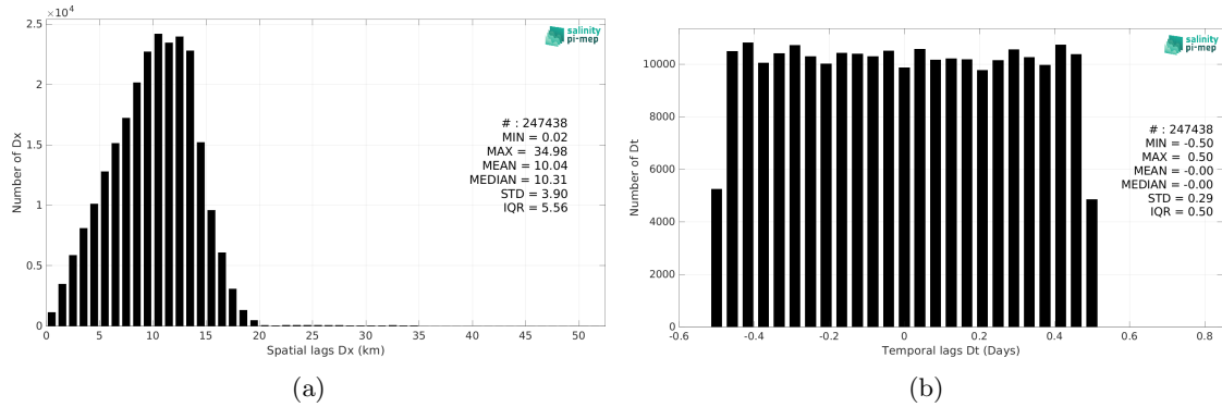
Figure 6: Histograms of the spatial (a) and temporal (b) lags between the location/time of the TSG (Polarstern) measurement and the date of the corresponding SMAP SSS L3 v5.0 - 8-Day running (JPL) SSS pixel.
