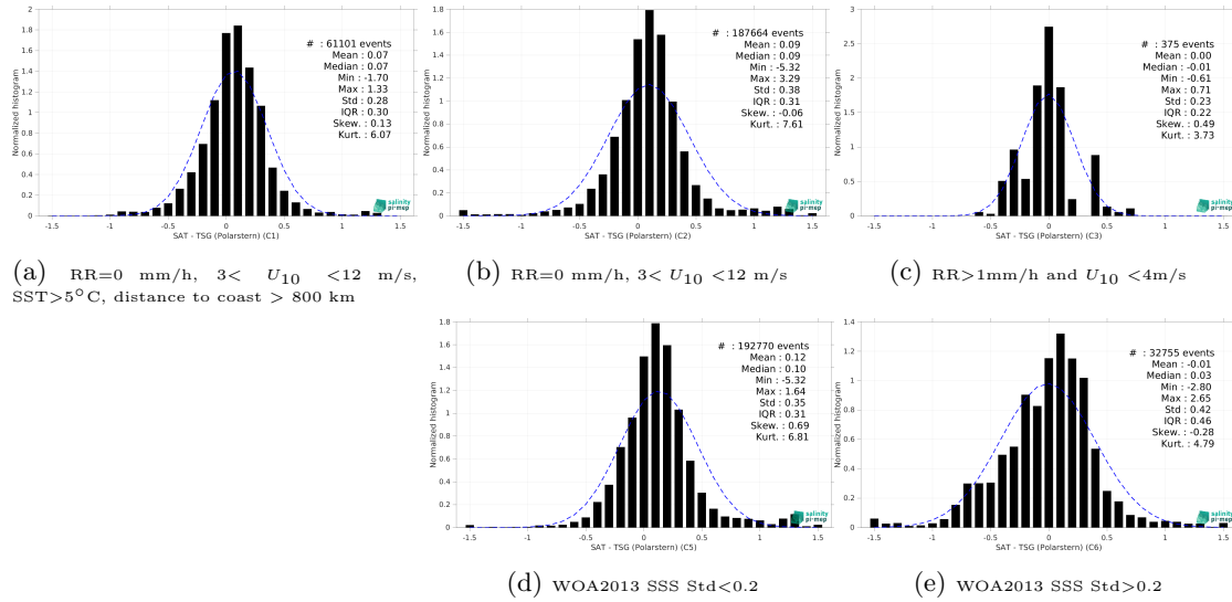
Figure 15: Normalized histogram of \Delta SSS (SMAP SSS L3 v5.0 - 8-Day running (JPL) - TSG (Polarstern)) for 5 different subdatasets corresponding to: RR=0 mm/h, 3 < U_{10} < 12 m/s, SST > 5°C, distance to coast > 800 km (a), RR=0 mm/h, 3 < U_{10} < 12 m/s (b), RR > 1mm/h and U_{10} < 4 m/s (c), WOA2013 SSS Std < 0.2 (d), WOA2013 SSS Std > 0.2 (e).
