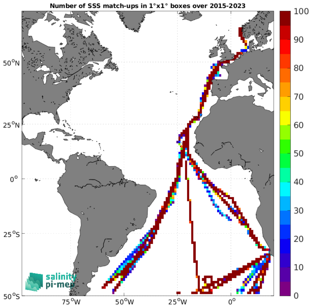
Figure 5: Number of SSS match-ups between TSG (Polarstern) SSS and the SMAP SSS L3 v5.0 - 8-Day running (JPL) SSS product for the Atlantic Ocean Pi-MEP region over 1°×1° boxes and for the full satellite product period.
