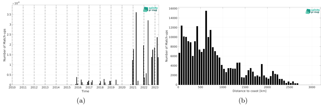
Figure 2: Number of match-ups between TSG (Polarstern) and SMAP SSS L3 v5.0 - 8-Day running (JPL) SSS as a function of time (a) and as function of the distance to coast (b) over the Atlantic Ocean Pi-MEP region and for the full satellite product period.
