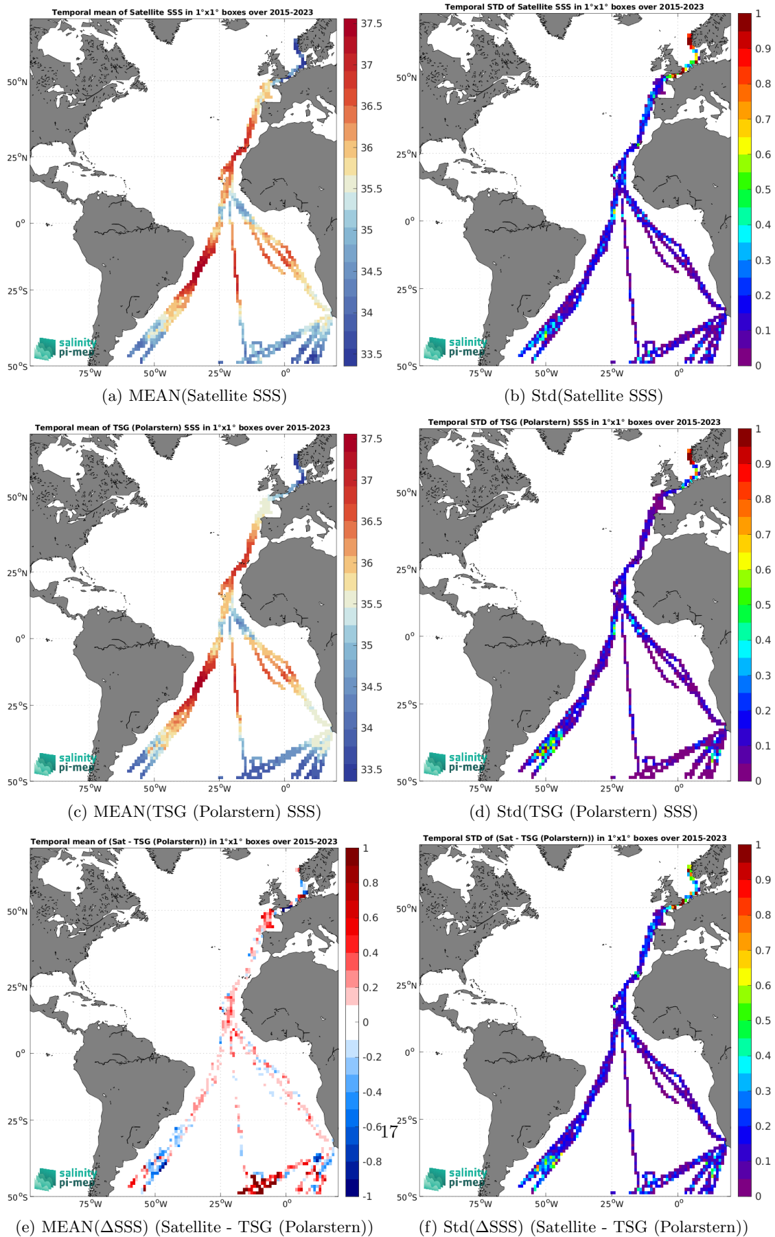
Figure 7: Temporal mean (left) and Std (right) of SSS from SMAP SSS L3 v5.0 - 8-Day running (JPL) (top), TSG (Polarstern) (middle), and of \Delta SSS (Satellite - TSG (Polarstern)). Only match-up pairs are used to generate these maps.
