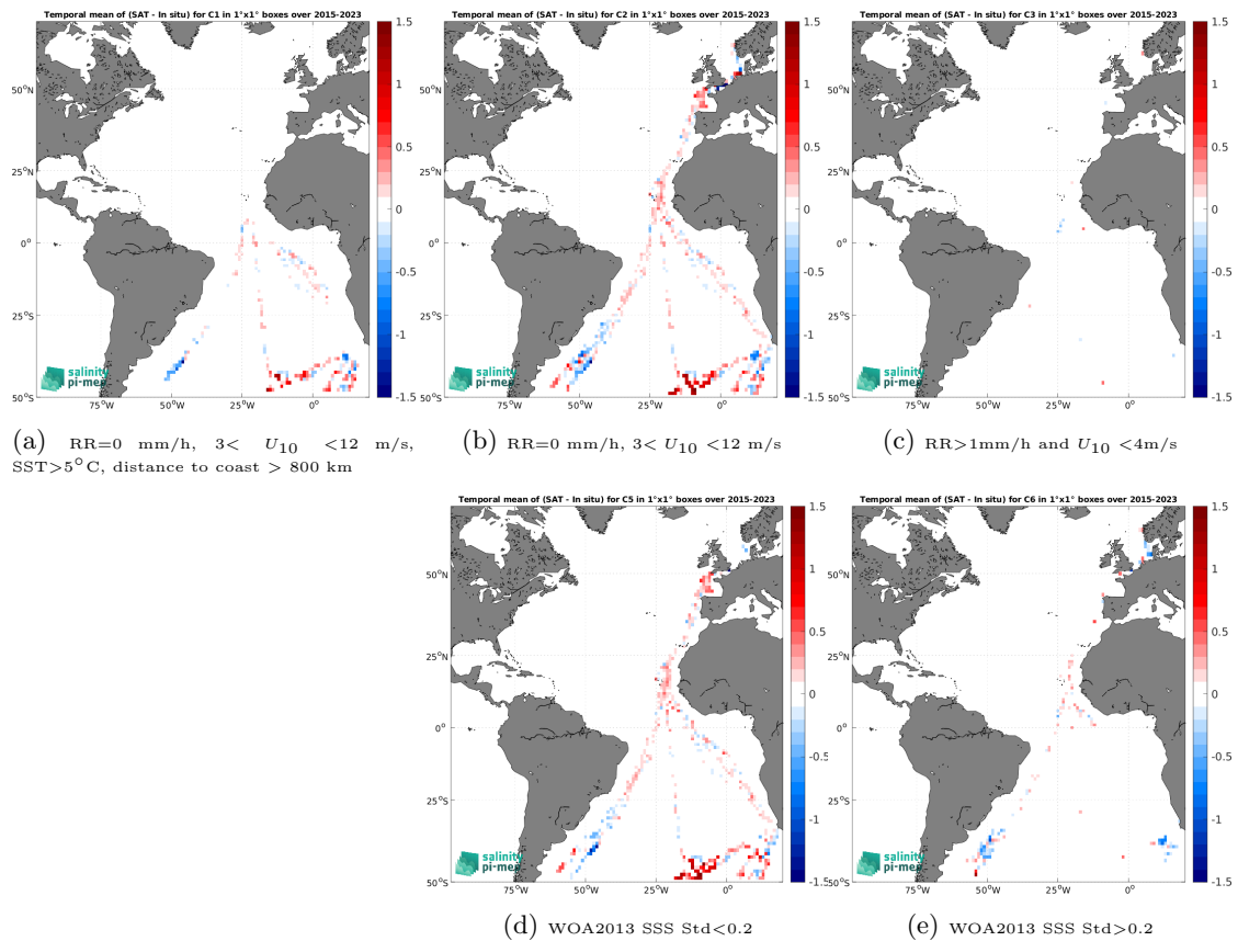
Figure 14: Temporal mean gridded over spatial boxes of size 1^\circ \times 1^\circ of \Delta SSS (SMAP SSS L3 v5.0 - 8-Day running (JPL) - TSG (Polarstern)) for 5 different subdatasets corresponding to:RR=0 mm/h, 3 < U_{10} < 12 m/s, SST >5^\circ\text{C} , distance to coast > 800 km (a), RR=0 mm/h, 3 < U_{10} < 12 m/s (b), RR >1 mm/h and U_{10} < 4 m/s (c), WOA2013 SSS Std <0.2 (d), WOA2013 SSS Std >0.2 (e).
