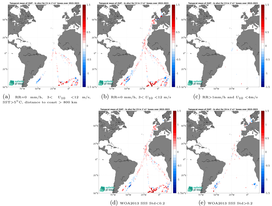
Figure 14: Temporal mean gridded over spatial boxes of size 1^\circ \times 1^\circ of \Delta SSS (SMAP SSS L3 v5.0 - 8-Day running (JPL) - TSG (Polarstern)) for 5 different subdatasets corresponding to:RR=0 mm/h, 3 < U_{10} < 12 m/s, SST >5^\circ\text{C} , distance to coast > 800 km (a), RR=0 mm/h, 3 < U_{10} < 12 m/s (b), RR >1 mm/h and U_{10} < 4 m/s (c), WOA2013 SSS Std <0.2 (d), WOA2013 SSS Std >0.2 (e).
