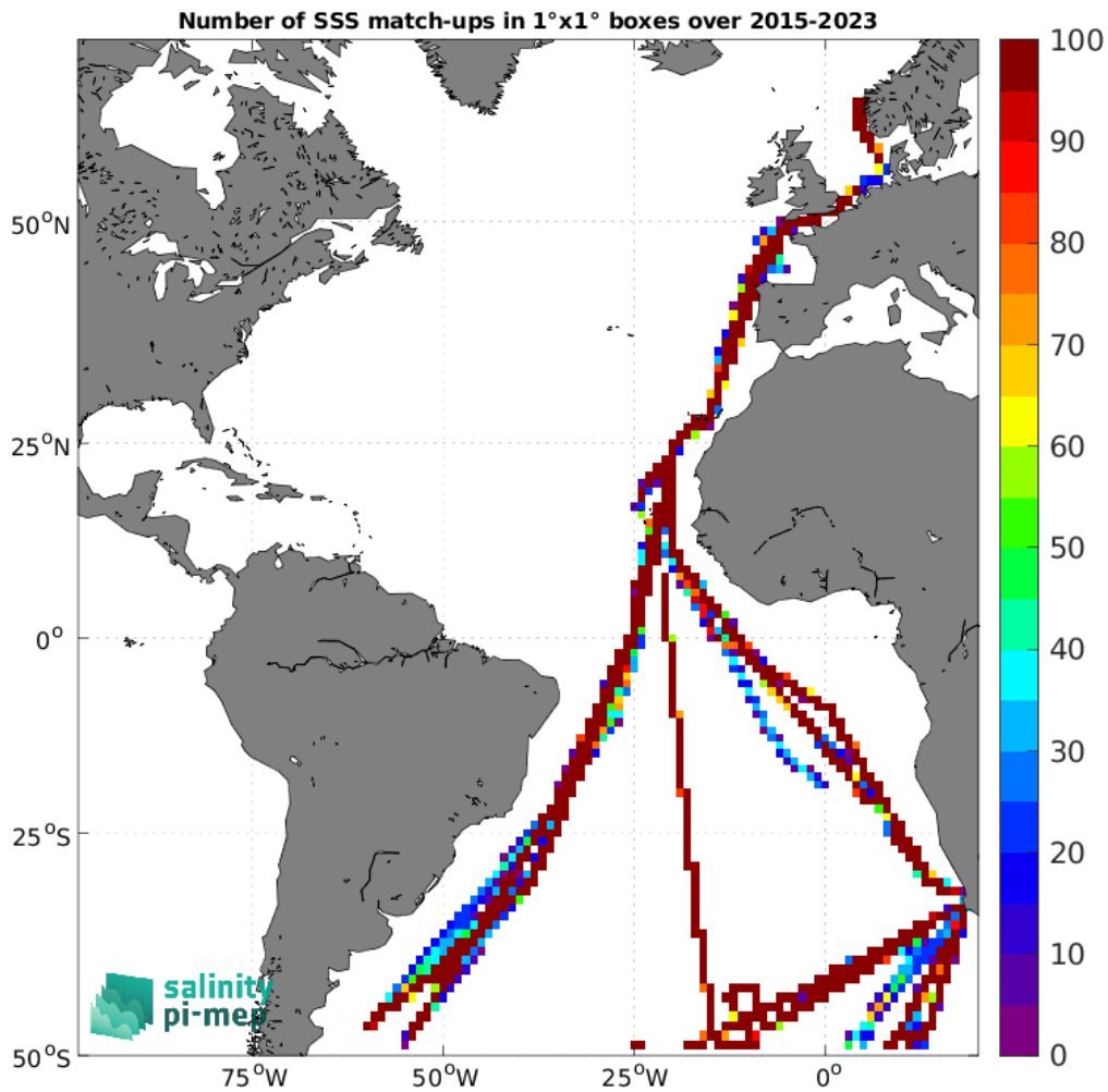
Figure 5: Number of SSS match-ups between TSG (Polarstern) SSS and the SMAP SSS L3 v5.0 - 8-Day running (JPL) SSS product for the Atlantic Ocean Pi-MEP region over 1^\circ \times 1^\circ boxes and for the full satellite product period.
