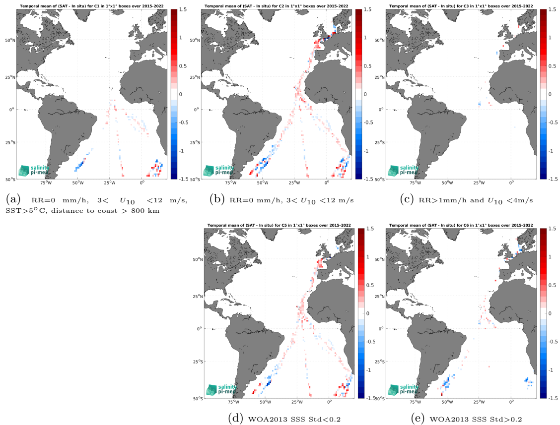
Figure 12: Temporal mean gridded over spatial boxes of size 1^\circ \times 1^\circ of \Delta SSS (SMAP SSS L3 v5.0 - 8-Day running (JPL) - TSG (Polarstern)) for 5 different subdatasets corresponding to:RR=0 mm/h, 3 < U_{10} < 12 m/s, SST >5^\circ\text{C} , distance to coast > 800 km (a), RR=0 mm/h, 3 < U_{10} < 12 m/s (b), RR >1 mm/h and U_{10} < 4 m/s (c), WOA2013 SSS Std <0.2 (d), WOA2013 SSS Std >0.2 (e).
