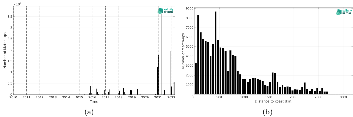
Figure 1: Number of match-ups between TSG (Polarstern) and SMAP SSS L3 v5.0 - 8-Day running (JPL) SSS as a function of time (a) and as function of the distance to coast (b) over the Atlantic Ocean Pi-MEP region and for the full satellite product period.
