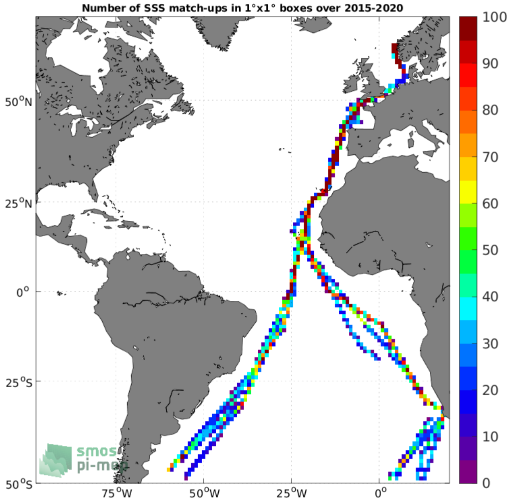
Figure 4: Number of SSS match-ups between TSG (Polarstern) SSS and the SMAP SSS L3 v5.0 - 8-Day running (JPL) SSS product for the Atlantic Ocean Pi-MEP region over 1°x1° boxes and for the full satellite product period.
