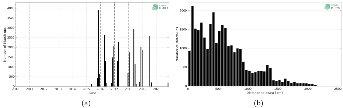
Figure 1: Number of match-ups between TSG (Polarstern) and SMAP SSS L3 v5.0 - 8-Day running (JPL) SSS as a function of time (a) and as function of the distance to coast (b) over the Atlantic Ocean Pi-MEP region and for the full satellite product period.
