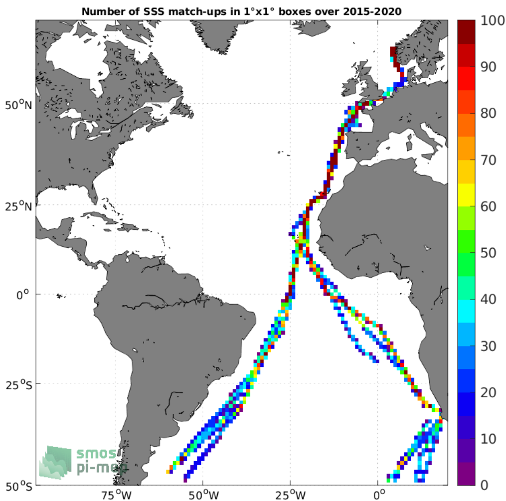
Figure 4: Number of SSS match-ups between TSG (Polarstern) SSS and the SMAP SSS L3 v5.0 - 8-Day running (JPL) SSS product for the Atlantic Ocean Pi-MEP region over 1°×1° boxes and for the full satellite product period.
