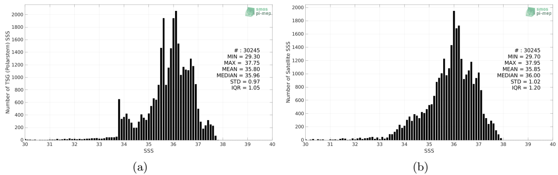
Figure 2: Histograms of SSS from TSG (Polarstern) (a) and SMAP SSS L3 v5.0 - 8-Day running (JPL) (b) considering all match-up pairs per bins of 0.1 over the Atlantic Ocean Pi-MEP region and for the full satellite product period.
