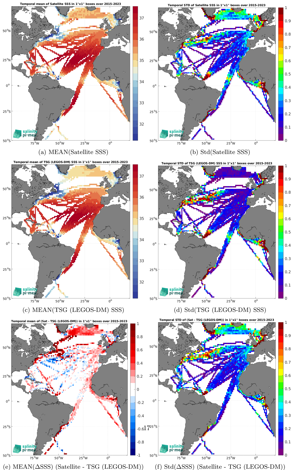
Figure 6: Temporal mean (left) and Std (right) of SSS from SMAP SSS L3 v5.0 - 8-Day running (JPL) (top), TSG (LEGOS-DM) (middle), and of \Delta SSS (Satellite - TSG (LEGOS-DM)). Only match-up pairs are used to generate these maps.
