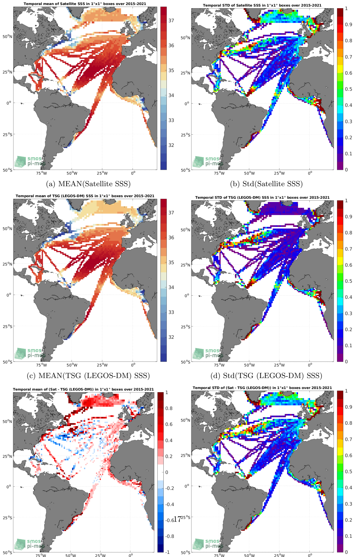
(e) MEAN( \Delta SSS) (Satellite - TSG (LEGOS-DM)) (f) Std( \Delta SSS) (Satellite - TSG (LEGOS-DM)) Figure 6: Temporal mean (left) and Std (right) of SSS from SMAP SSS L3 v5.0 - 8-Day running (JPL) (top), TSG (LEGOS-DM) (middle), and of \Delta SSS (Satellite - TSG (LEGOS-DM)). Only match-up pairs are used to generate these maps.
