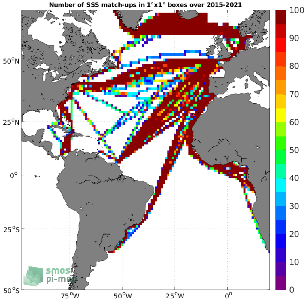
Figure 4: Number of SSS match-ups between TSG (LEGOS-DM) SSS and the SMAP SSS L3 v5.0 - 8-Day running (JPL) SSS product for the Atlantic Ocean Pi-MEP region over 1°x1° boxes and for the full satellite product period.
