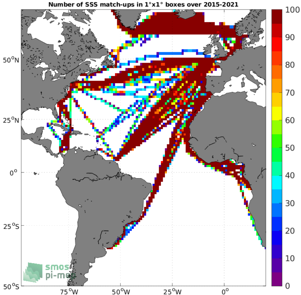
Figure 4: Number of SSS match-ups between TSG (LEGOS-DM) SSS and the SMAP SSS L3 v5.0 - 8-Day running (JPL) SSS product for the Atlantic Ocean Pi-MEP region over 1^\circ \times 1^\circ boxes and for the full satellite product period.
