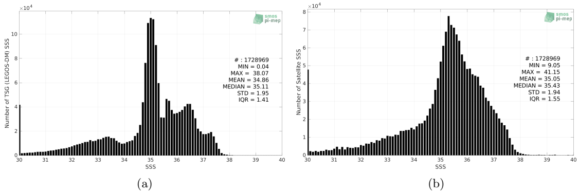
Figure 2: Histograms of SSS from TSG (LEGOS-DM) (a) and SMAP SSS L3 v5.0 - 8-Day running (JPL) (b) considering all match-up pairs per bins of 0.1 over the Atlantic Ocean Pi-MEP region and for the full satellite product period.
