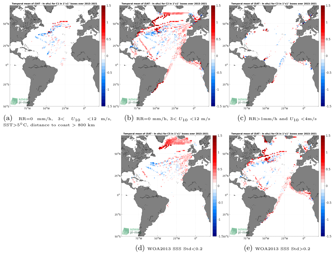
Figure 12: Temporal mean gridded over spatial boxes of size 1^\circ \times 1^\circ of \Delta SSS (SMAP SSS L3 v5.0 - 8-Day running (JPL) - TSG (LEGOS-DM)) for 5 different subdatasets corresponding to:RR=0 mm/h, 3 < U_{10} < 12 m/s, SST >5^\circ\text{C} , distance to coast > 800 km (a), RR=0 mm/h, 3 < U_{10} < 12 m/s (b), RR >1 mm/h and U_{10} < 4 m/s (c), WOA2013 SSS Std <0.2 (d), WOA2013 SSS Std >0.2 (e).
