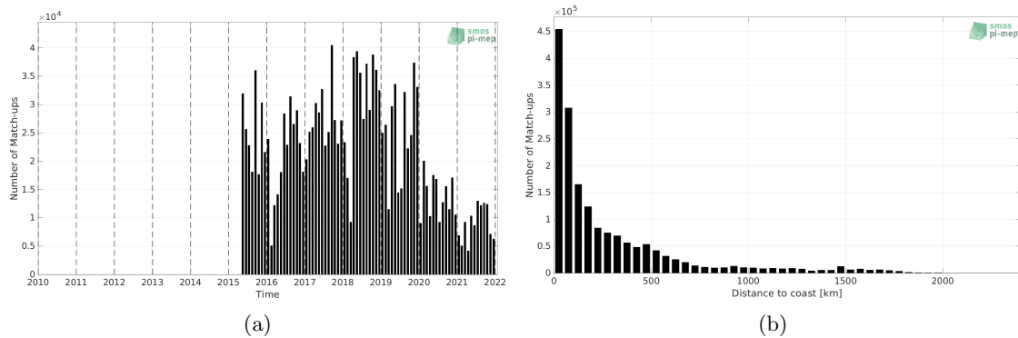
Figure 1: Number of match-ups between TSG (LEGOS-DM) and SMAP SSS L3 v5.0 - 8-Day running (JPL) SSS as a function of time (a) and as function of the distance to coast (b) over the Atlantic Ocean Pi-MEP region and for the full satellite product period.
