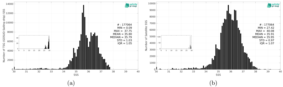
Figure 3: Histograms of SSS from TSG (GOSUD-Sailing-ship) (a) and SMAP SSS L3 v5.0 - 8-Day running (JPL) (b) considering all match-up pairs per bins of 0.1 over the Atlantic Ocean Pi-MEP region and for the full satellite product period.
