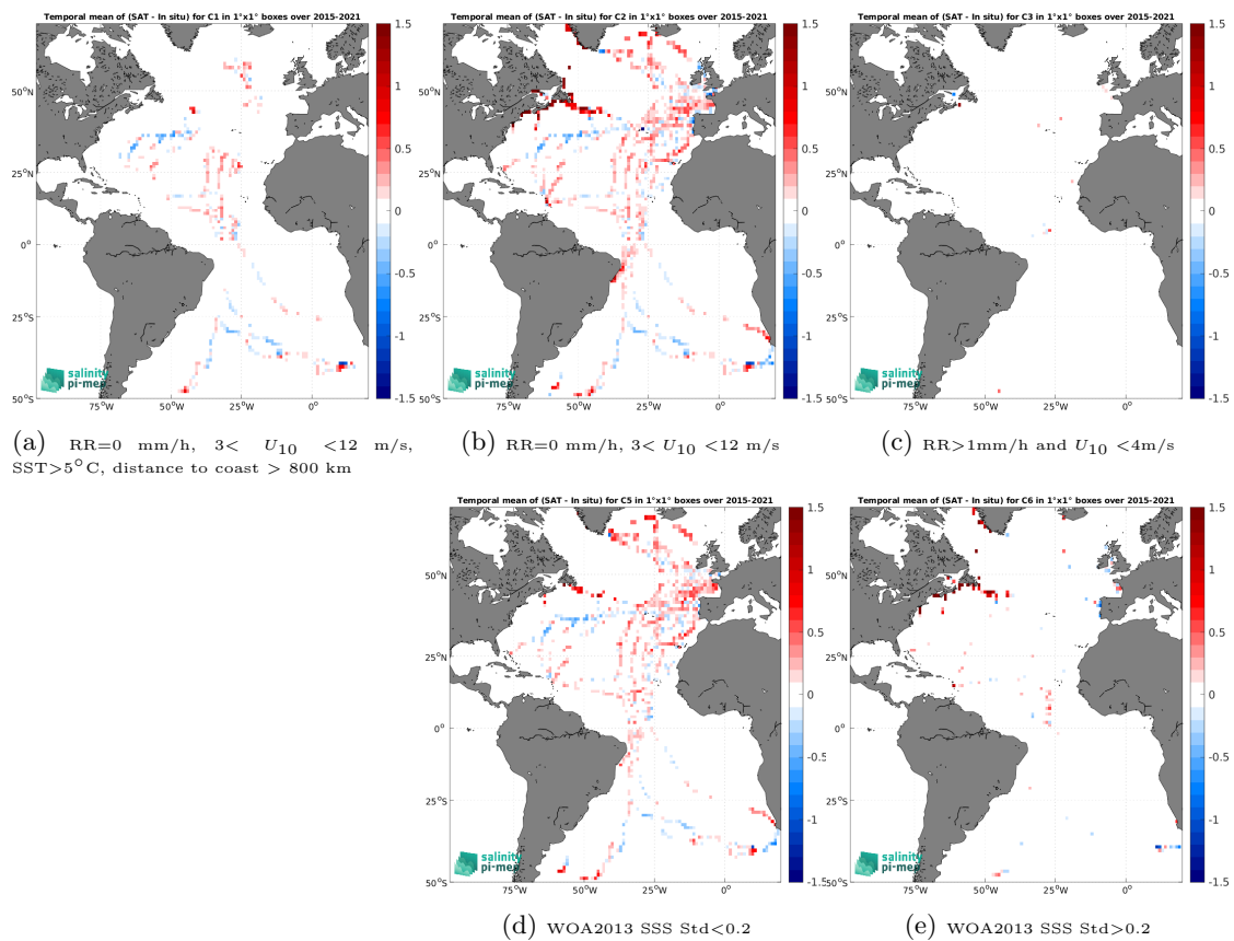
Figure 14: Temporal mean gridded over spatial boxes of size 1^\circ \times 1^\circ of \Delta\text{SSS} (SMAP SSS L3 v5.0 - 8-Day running (JPL) - TSG (GOSUD-Sailing-ship)) for 5 different subdatasets corresponding to:RR=0 mm/h, 3 < U_{10} < 12 m/s, SST >5^\circ\text{C} , distance to coast > 800 km (a), RR=0 mm/h, 3 < U_{10} < 12 m/s (b), RR >1 mm/h and U_{10} < 4 m/s (c), WOA2013 SSS Std <0.2 (d), WOA2013 SSS Std >0.2 (e).
