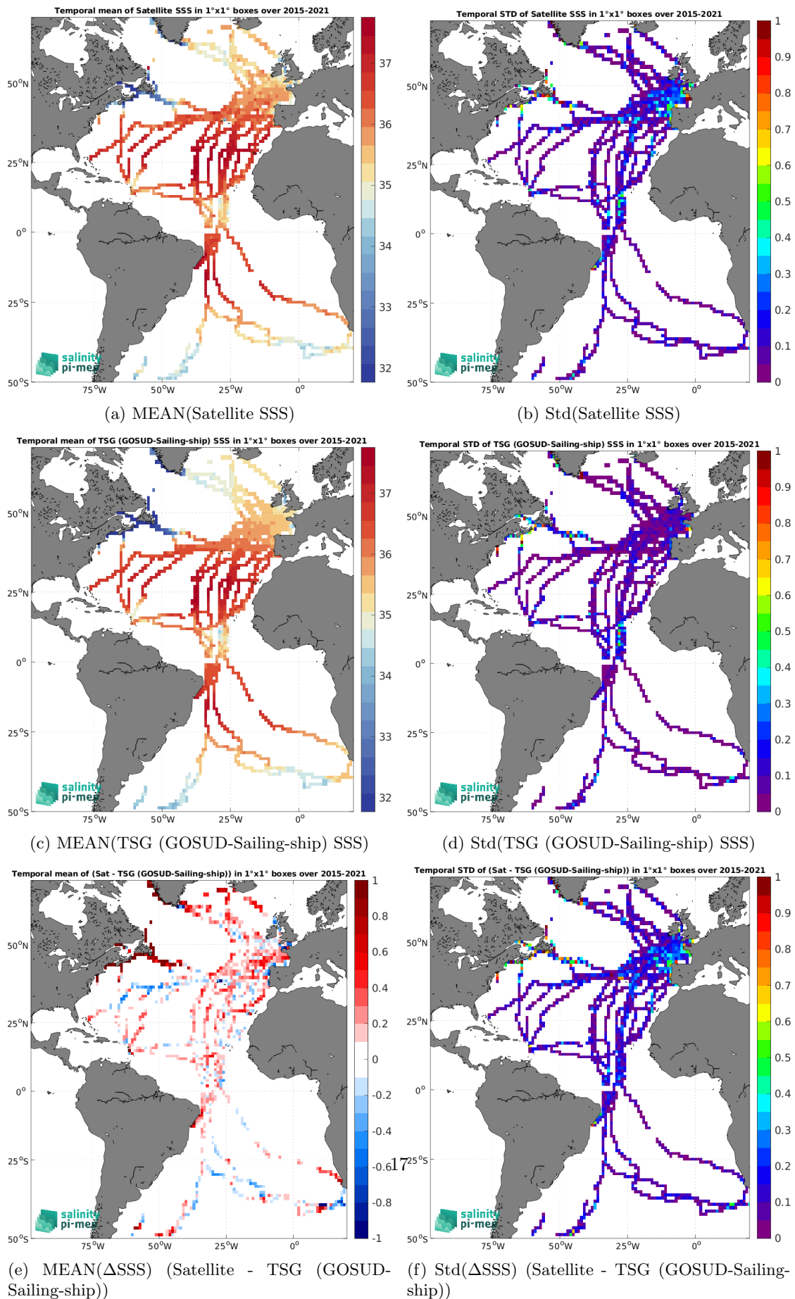
Figure 7: Temporal mean (left) and Std (right) of SSS from SMAP SSS L3 v5.0 - 8-Day running (JPL) (top), TSG (GOSUD-Sailing-ship) (middle), and of \Delta SSS (Satellite - TSG (GOSUD-Sailing-ship)). Only match-up pairs are used to generate these maps.
