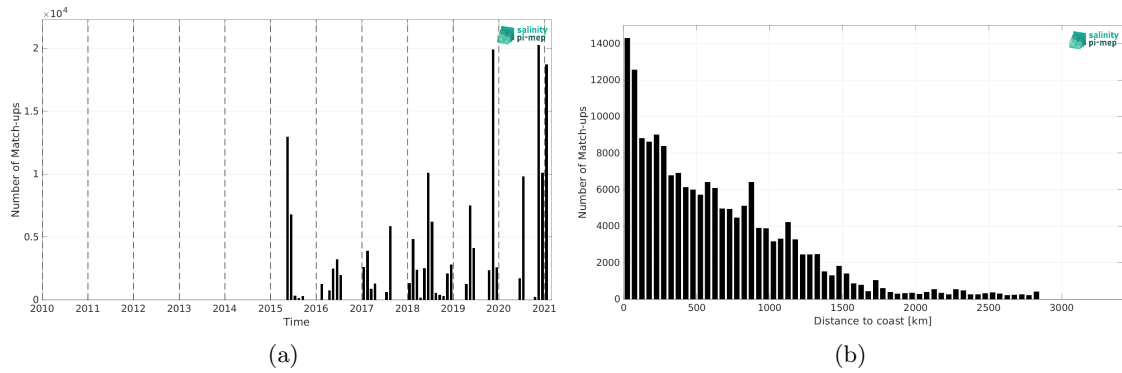
Figure 2: Number of match-ups between TSG (GOSUD-Sailing-ship) and SMAP SSS L3 v5.0 - 8-Day running (JPL) SSS as a function of time (a) and as function of the distance to coast (b) over the Atlantic Ocean Pi-MEP region and for the full satellite product period.
