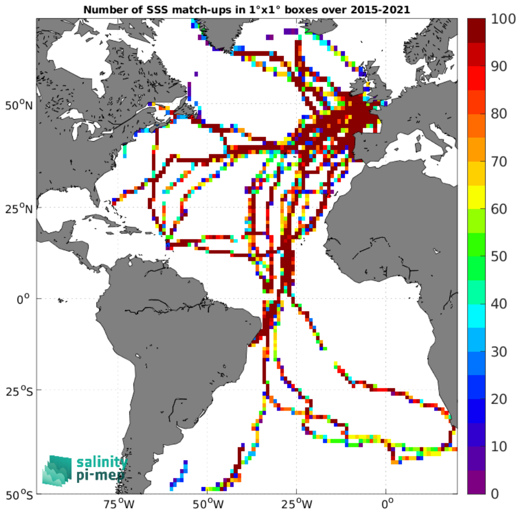
Figure 5: Number of SSS match-ups between TSG (GOSUD-Sailing-ship) SSS and the SMAP SSS L3 v5.0 - 8-Day running (JPL) SSS product for the Atlantic Ocean Pi-MEP region over 1^\circ \times 1^\circ boxes and for the full satellite product period.
