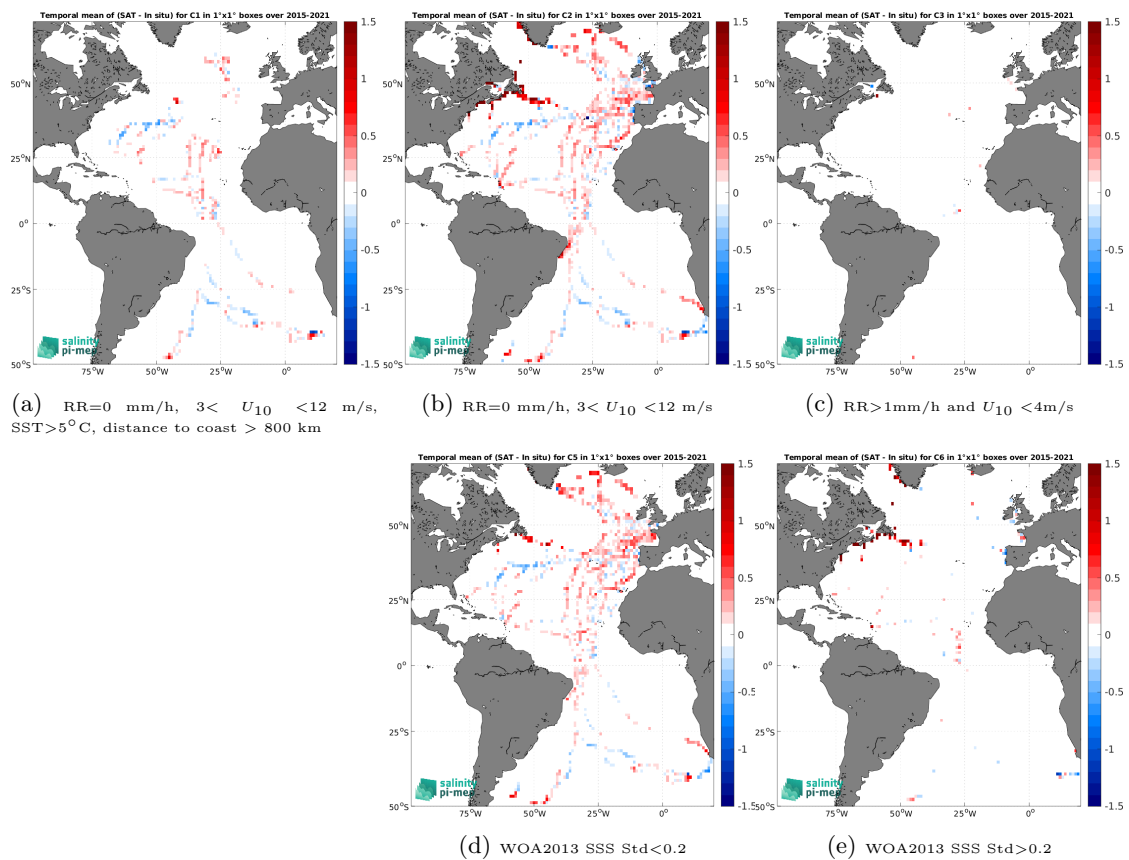
Figure 14: Temporal mean gridded over spatial boxes of size 1^\circ \times 1^\circ of \Delta SSS (SMAP SSS L3 v5.0 - 8-Day running (JPL) - TSG (GOSUD-Sailing-ship)) for 5 different subdatasets corresponding to:RR=0 mm/h, 3 < U_{10} < 12 m/s, SST >5^\circ\text{C} , distance to coast > 800 km (a), RR=0 mm/h, 3 < U_{10} < 12 m/s (b), RR >1 mm/h and U_{10} < 4 m/s (c), WOA2013 SSS Std <0.2 (d), WOA2013 SSS Std >0.2 (e).
