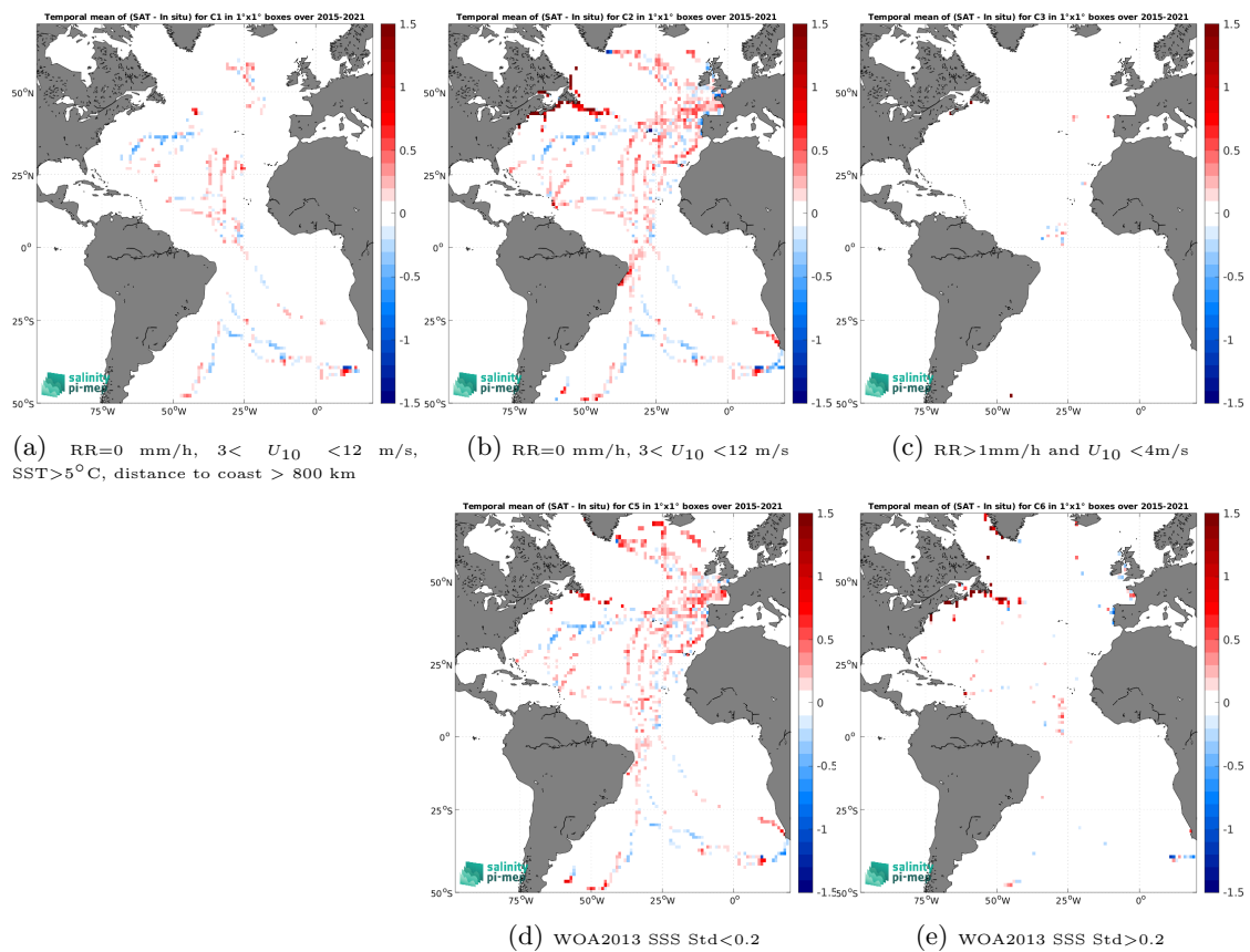
Figure 12: Temporal mean gridded over spatial boxes of size 1^\circ \times 1^\circ of \Delta\text{SSS} (SMAP SSS L3 v5.0 - 8-Day running (JPL) - TSG (GOSUD-Sailing-ship)) for 5 different subdatasets corresponding to:RR=0 mm/h, 3 < U_{10} < 12 m/s, SST >5^\circ\text{C} , distance to coast > 800 km (a), RR=0 mm/h, 3 < U_{10} < 12 m/s (b), RR >1 mm/h and U_{10} < 4 m/s (c), WOA2013 SSS Std <0.2 (d), WOA2013 SSS Std >0.2 (e).
