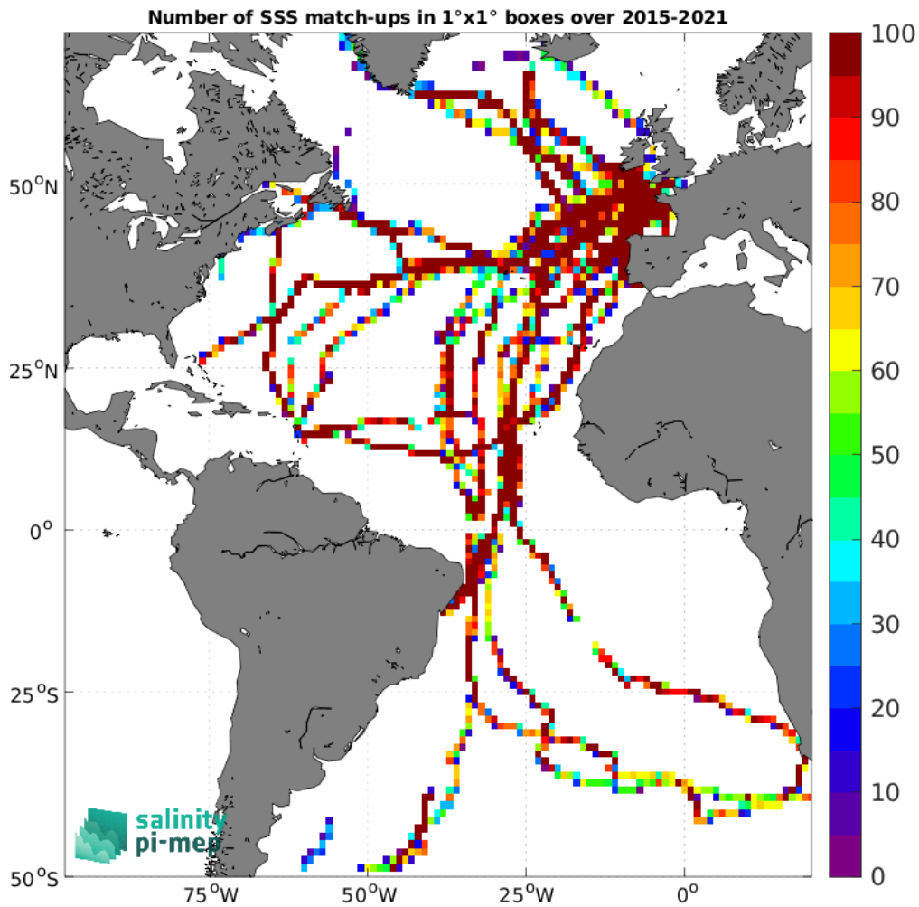
Figure 4: Number of SSS match-ups between TSG (GOSUD-Sailing-ship) SSS and the SMAP SSS L3 v5.0 - 8-Day running (JPL) SSS product for the Atlantic Ocean Pi-MEP region over 1°×1° boxes and for the full satellite product period.
