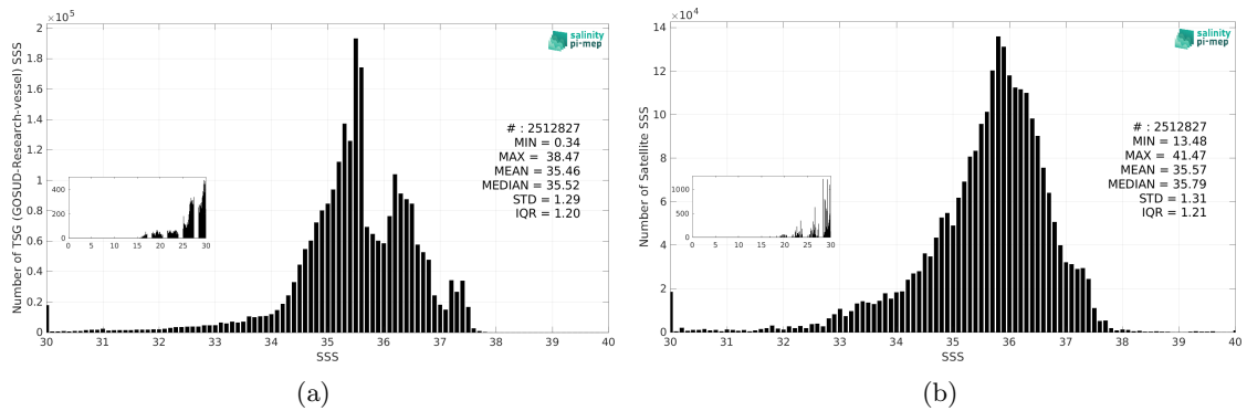
Figure 3: Histograms of SSS from TSG (GOSUD-Research-vessel) (a) and SMAP SSS L3 v5.0 - 8-Day running (JPL) (b) considering all match-up pairs per bins of 0.1 over the Atlantic Ocean Pi-MEP region and for the full satellite product period.
