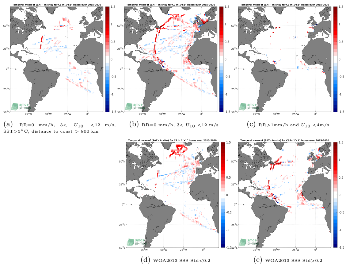
Figure 12: Temporal mean gridded over spatial boxes of size 1^\circ \times 1^\circ of \Delta\text{SSS} (SMAP SSS L3 v5.0 - 8-Day running (JPL) - TSG (GOSUD-Research-vessel)) for 5 different subdatasets corresponding to:RR=0 mm/h, 3 < U_{10} < 12 m/s, SST>5°C, distance to coast > 800 km (a), RR=0 mm/h, 3 < U_{10} < 12 m/s (b), RR>1mm/h and U_{10} < 4 m/s (c), WOA2013 SSS Std<0.2 (d), WOA2013 SSS Std>0.2 (e).
