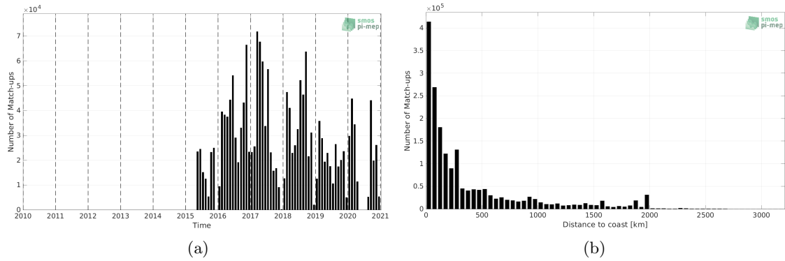
Figure 1: Number of match-ups between TSG (GOSUD-Research-vessel) and SMAP SSS L3 v5.0 - 8-Day running (JPL) SSS as a function of time (a) and as function of the distance to coast (b) over the Atlantic Ocean Pi-MEP region and for the full satellite product period.
