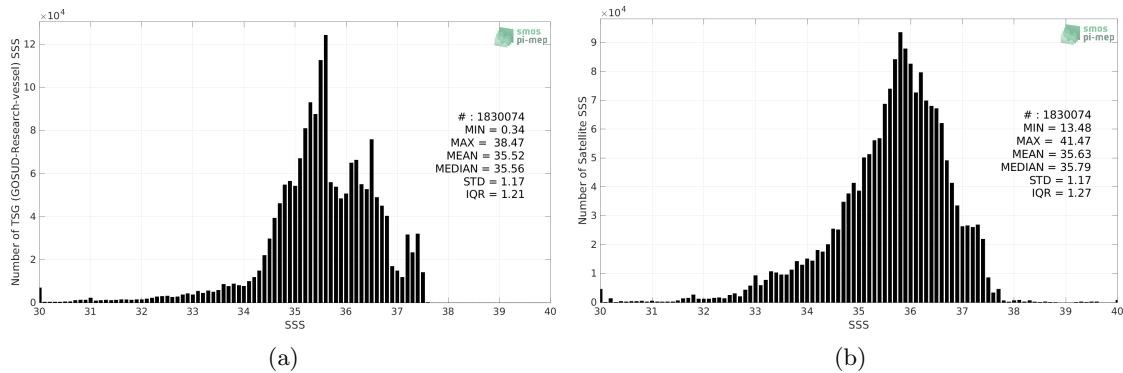
Figure 2: Histograms of SSS from TSG (GOSUD-Research-vessel) (a) and SMAP SSS L3 v5.0 - 8-Day running (JPL) (b) considering all match-up pairs per bins of 0.1 over the Atlantic Ocean Pi-MEP region and for the full satellite product period.
