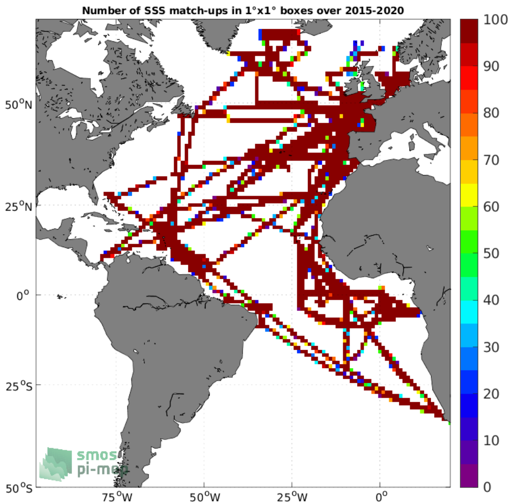
Figure 4: Number of SSS match-ups between TSG (GOSUD-Research-vessel) SSS and the SMAP SSS L3 v5.0 - 8-Day running (JPL) SSS product for the Atlantic Ocean Pi-MEP region over 1^\circ \times 1^\circ boxes and for the full satellite product period.
